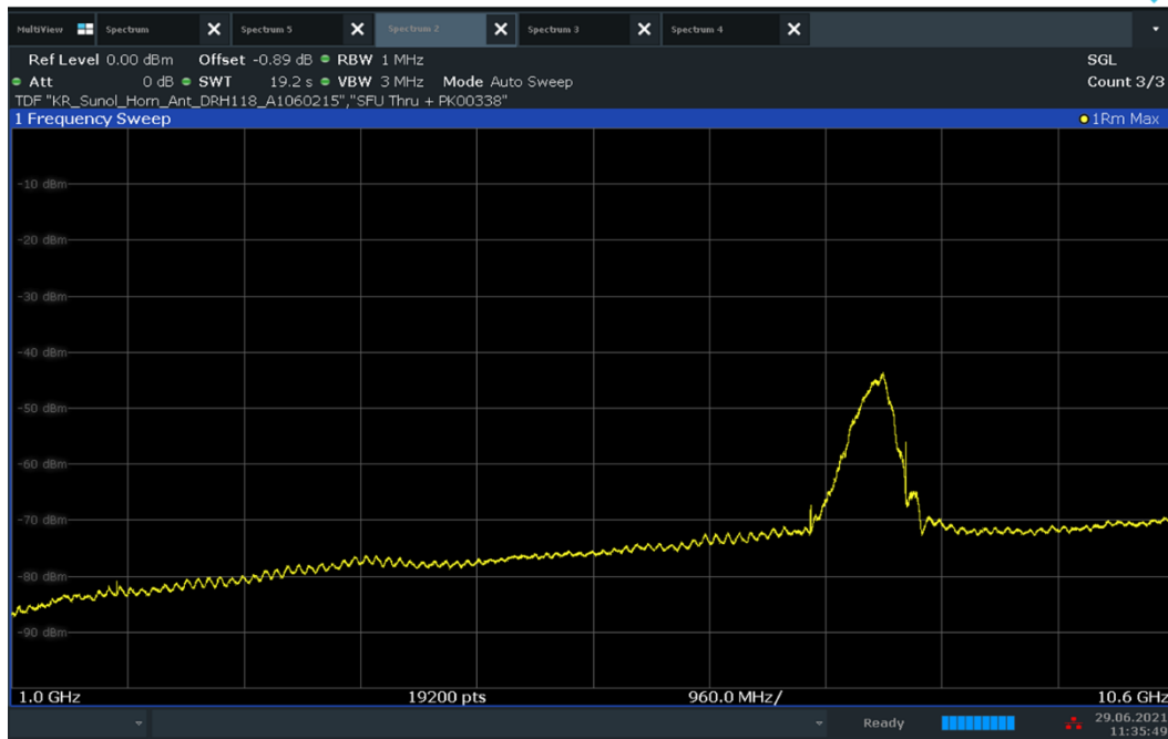
Plot 7-27. Radiated Spurious Pre-Scan 1000 - 10600 MHz - CH.9 - ANT 1
