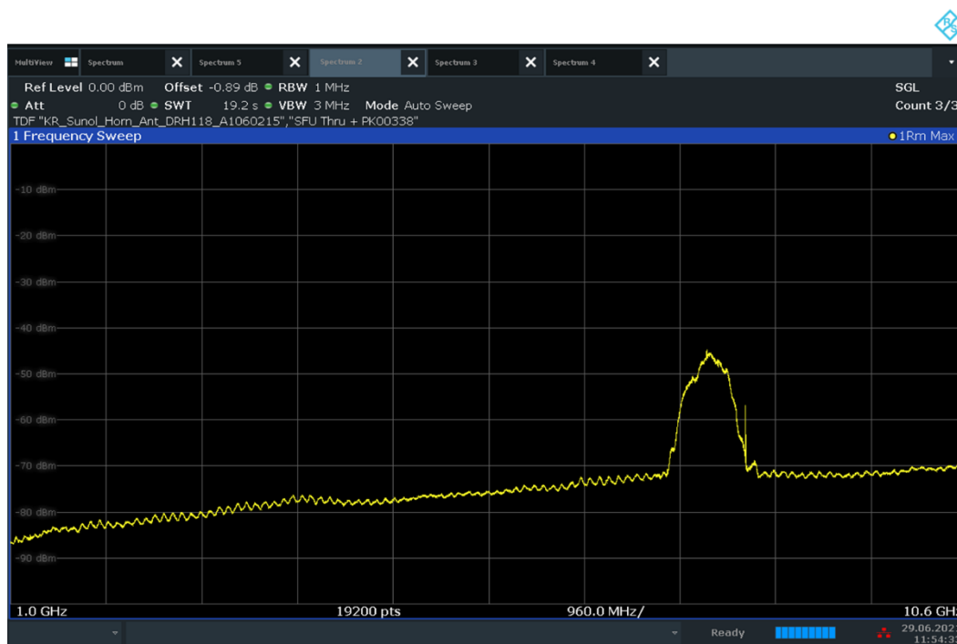
Plot 7-32. Radiated Spurious Pre-Scan 1000 - 10600 MHz - CH.9 - ANT 2
