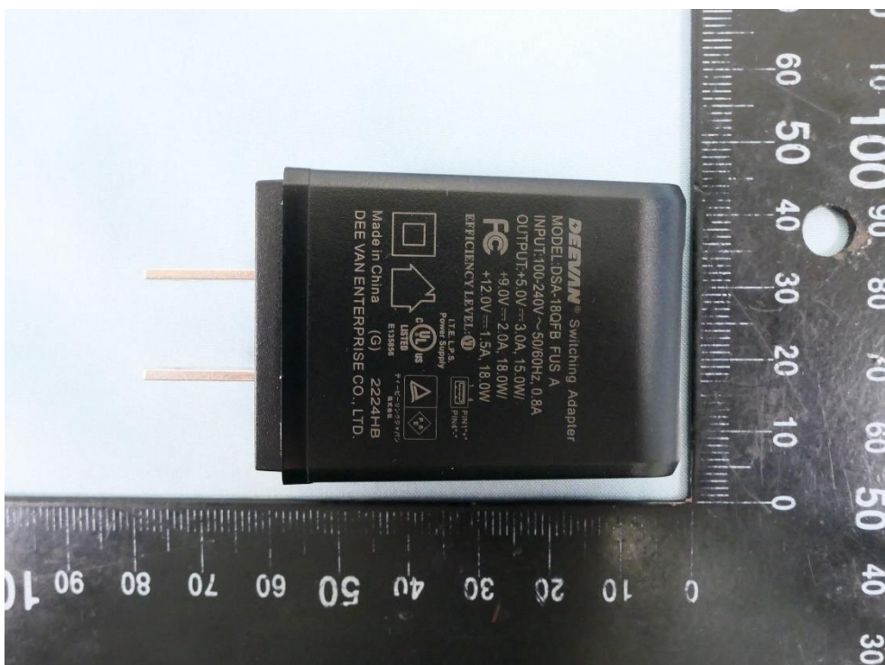
(8) EUT Photo (Brand: DEEVAN, M/N: DSA-18QFB FUS A)
