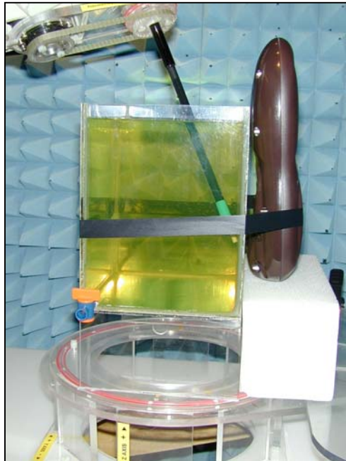
Figure 36. Positional photograph of 4111-GPRS Touch Position Rear Facing
