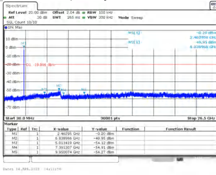
Tx. Spurious NVNT g 2462MHz Ant1 Emission
