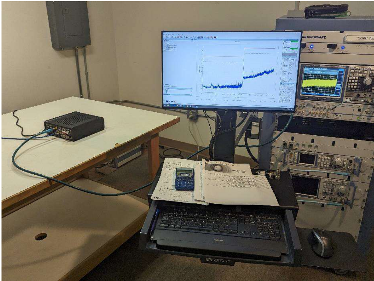
Photograph 5: Antenna Port Conducted Emissions Setup
