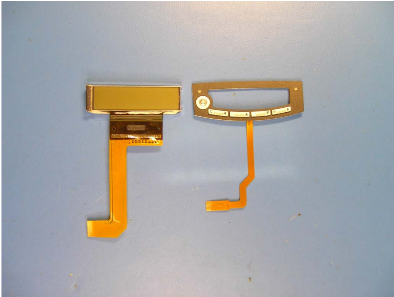
Figure 4 Display and Keyboard
