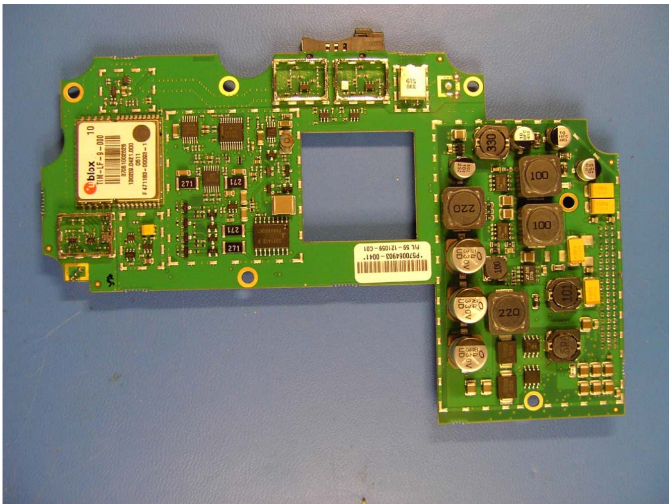
Figure 1 PSU, 2-Wire and GPS Board
