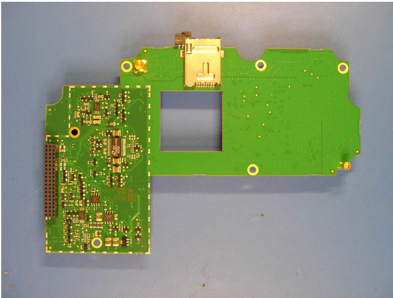
Figure 2 PSU, 2-Wire and GPS Board
