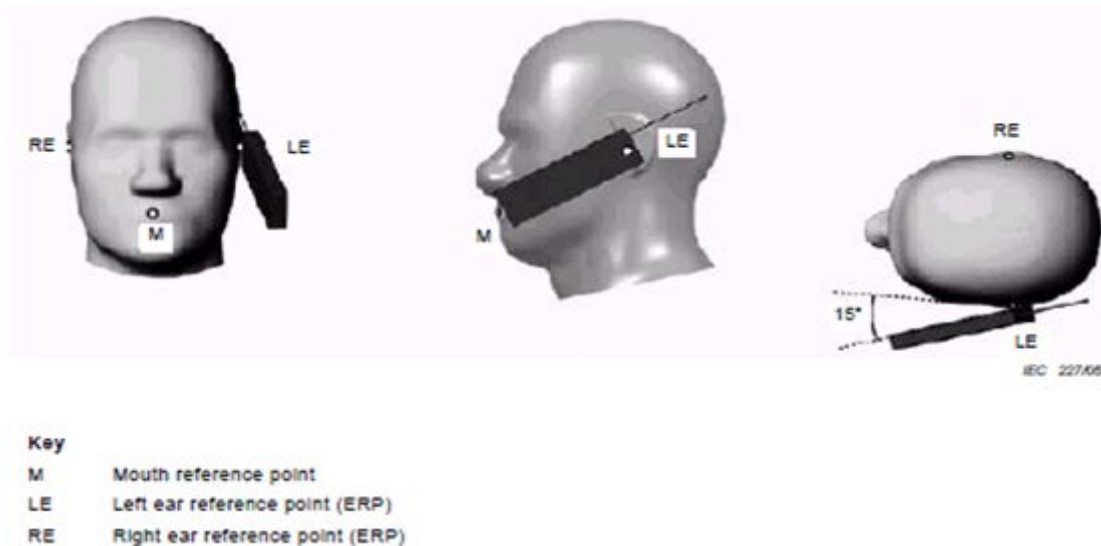
Figure 4 Tilt position of the wireless device on the left side of SAM
