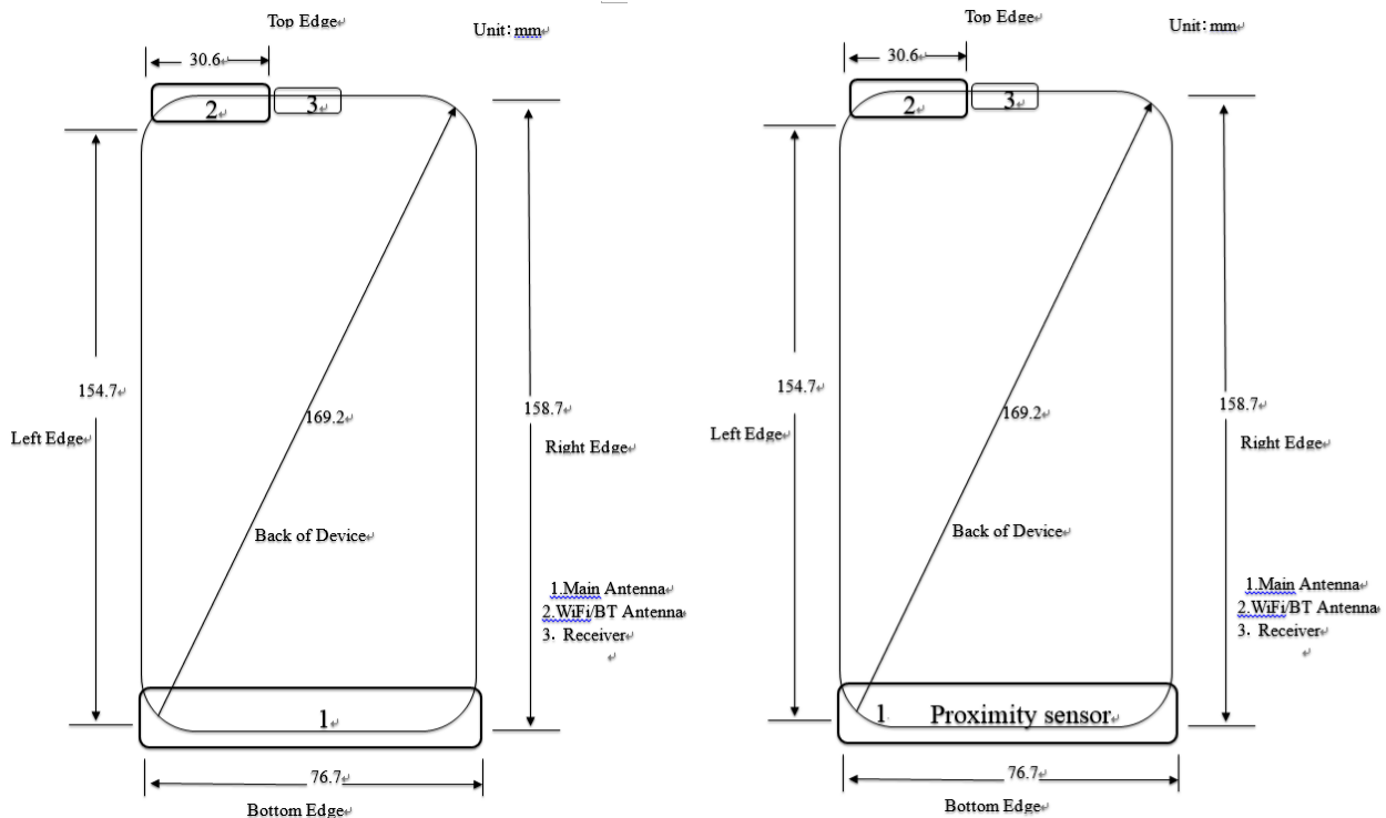
Figure1: The location of the antennas and the proximity sensor
