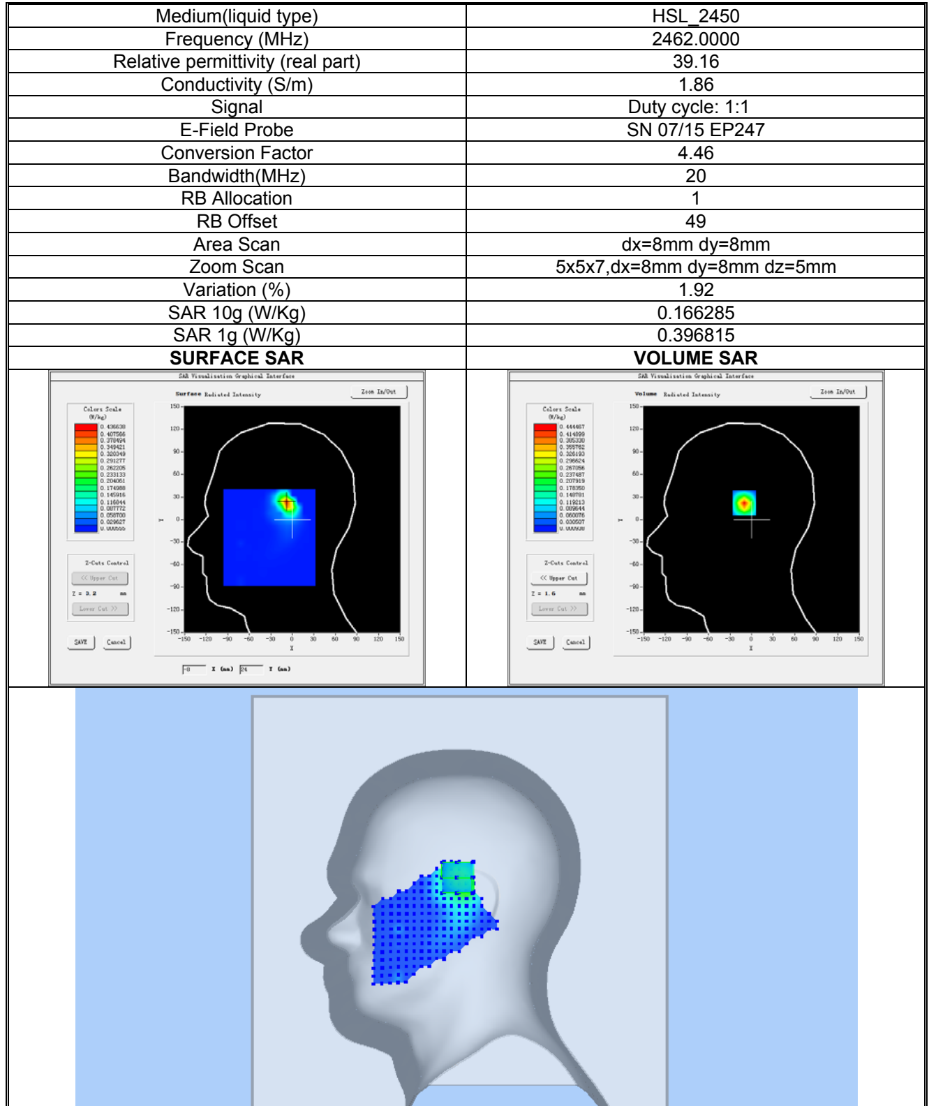
Plot 19:802.11b, High channel (Right Head Tilt) Product Description: Mobile Phone Test Date: 2020-01-13
