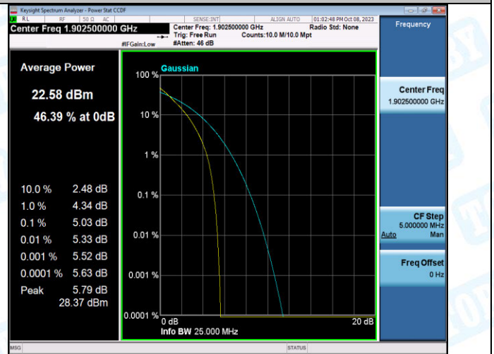
Band2-15MHz-QPSK-19125-75RB#0-PASS
