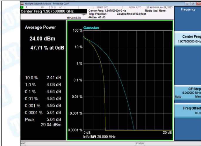
Band2-5MHz-QPSK-19175-25RB#0-PASS
