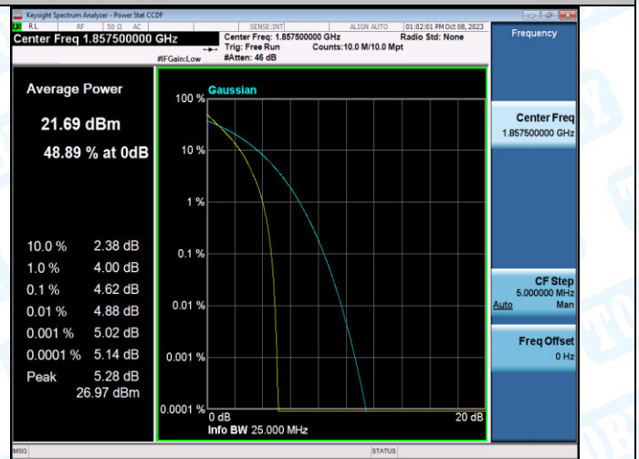
Band2-15MHz-QPSK-18675-75RB#0-PASS
