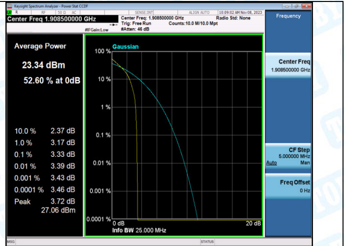
Band2-3MHz-QPSK-19185-1RB#0-PASS
