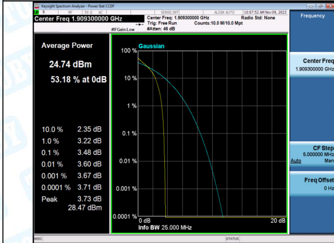
Band2-1.4MHz-QPSK-19193-1RB#0-PASS
