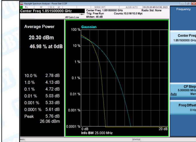
Band2-3MHz-16QAM-18615-15RB#0-PASS
