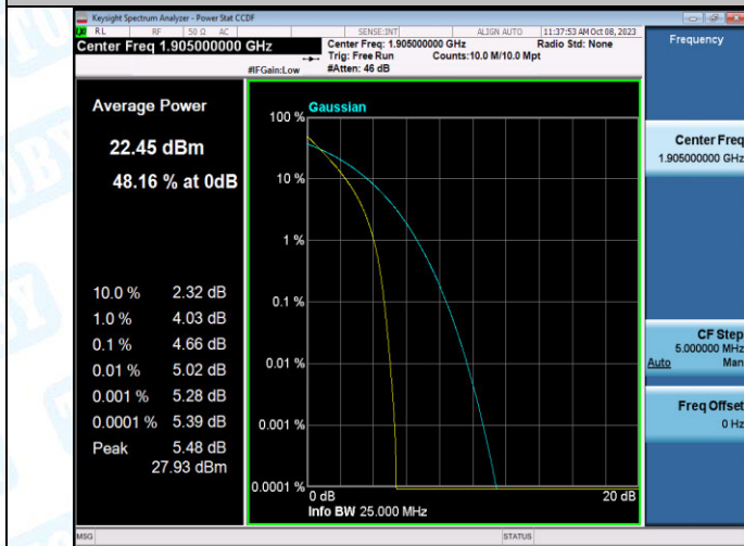
Band2-10MHz-QPSK-19150-50RB#0-PASS
