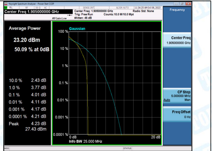
Band2-10MHz-QPSK-19150-1RB#0-PASS
