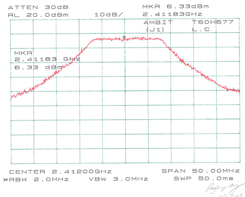
Plots of Peak Output Power for 802.11 g (15.247)
