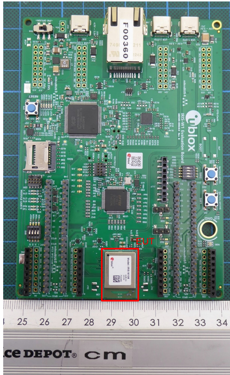
IRIS-W106-00B on evaluation board – top view
