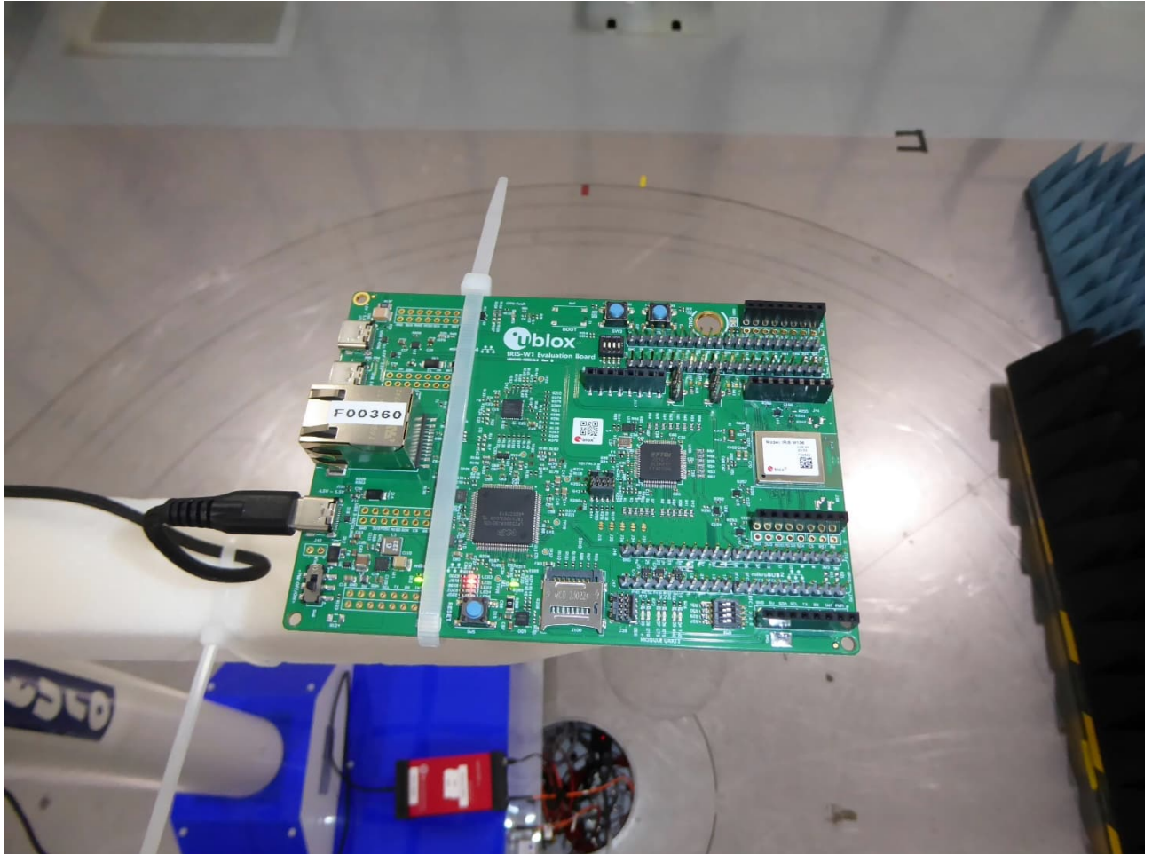
EUT on positioner
