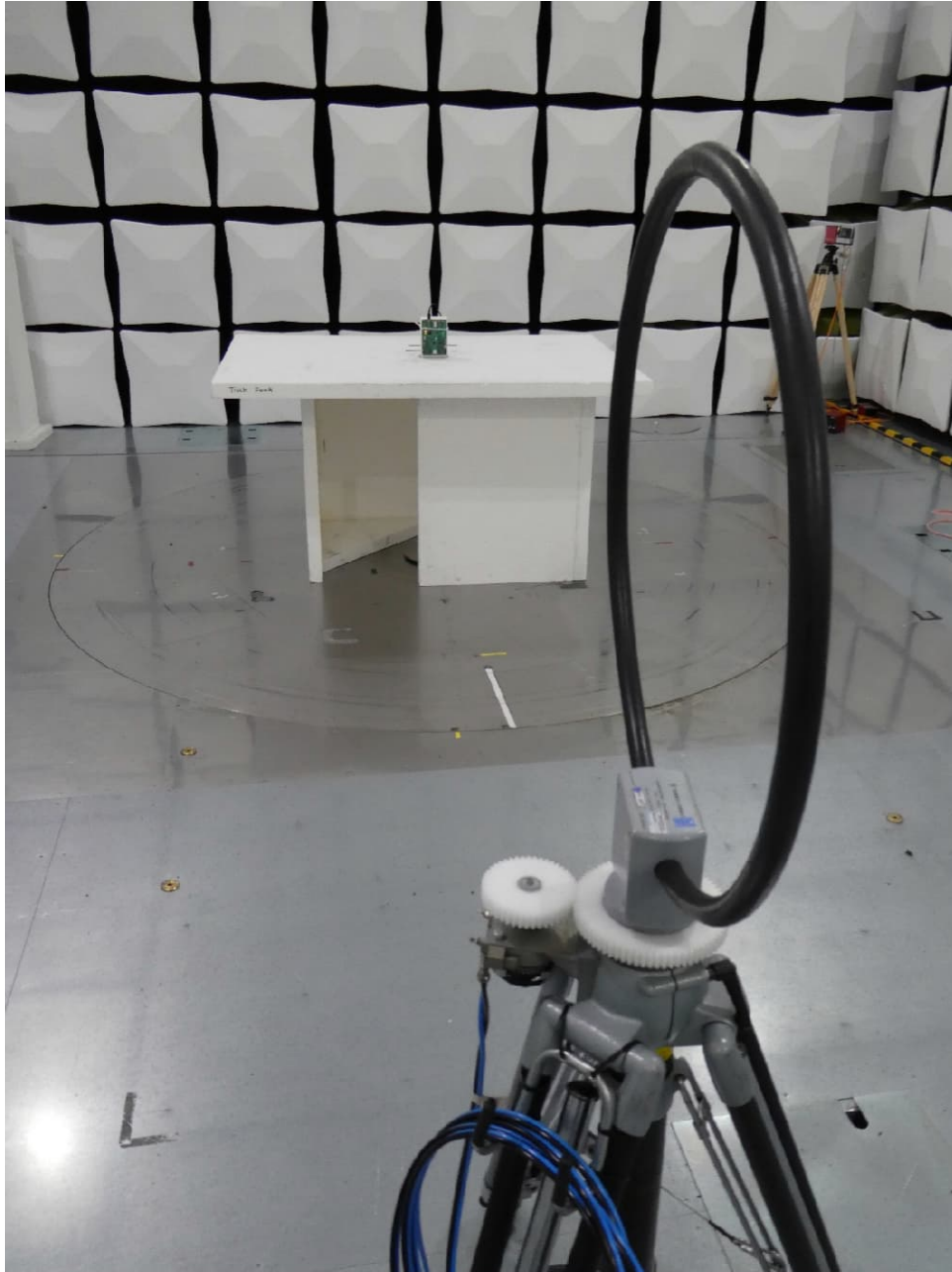
Antenna position 2, EUT Position 3
