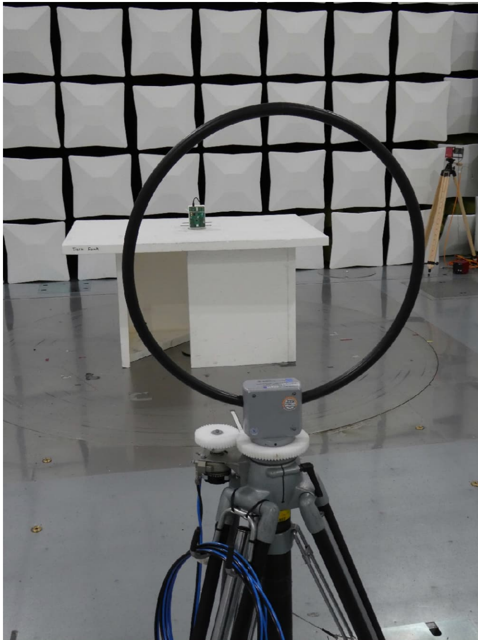
Antenna position 1, EUT Position 3
