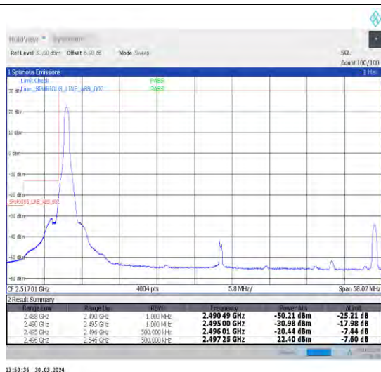
1-N41-30-50-L-1-DFT-PI2BPSK-Edge_1RB_Left-1@0-Ant1-1--PASS-see graph
