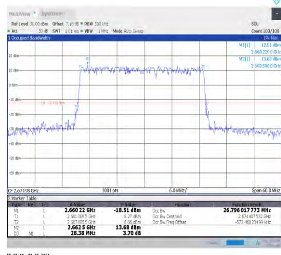
1-N41-30-30-H-4-DFT-64QAM-Outet_Full-75@0-Ant1 1-26.796-28.380-≤30-PASS
