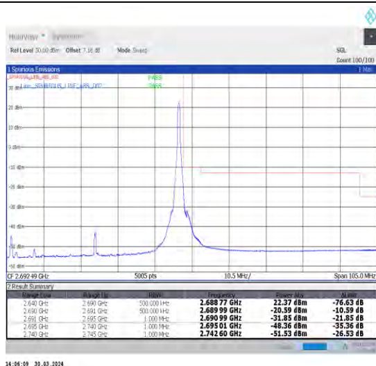
1-N41-30-50-H-2-DFT-PI2BPSK-Edge_1RB_Right-1@132-Ant1-1--PASS-see graph
