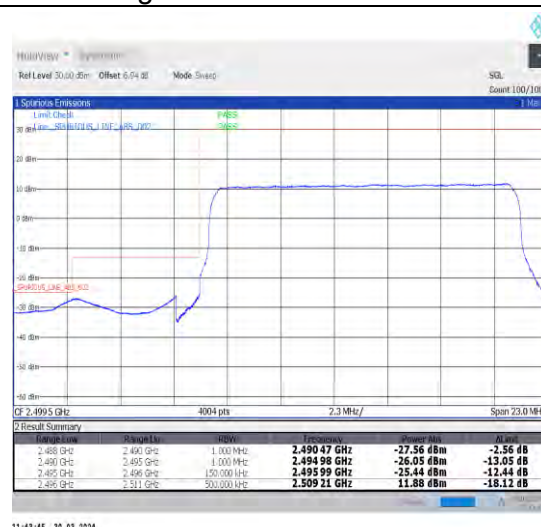
1-N41-30-15-L-3-DFT-PI2BPSK-Outer_Full-36@0-Ant1-1--PASS-see graph
