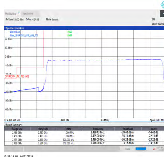
1-N41-30-25-L-6-CP-QPSK-Outer_Full-65@0-Ant1-1--PASS-see graph
