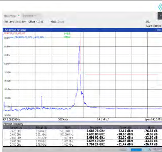
1-N41-30-70-H-2-DFT-PI2BPSK-Edge_1RB_Right-1@188-Ant1-1--PASS-see graph
