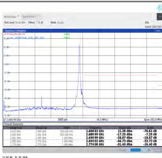
1-N41-30-80-H-5-CP-QPSK-Edge_1RB_Right-1@216- Ant1-1--PASS-see graph
