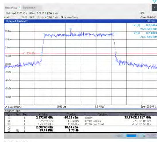
1-N41-30-40-M-3-DFT-16QAM-Outer_Full-100@0-Ant1 nt1-35.974-38.480-≤40-PASS
