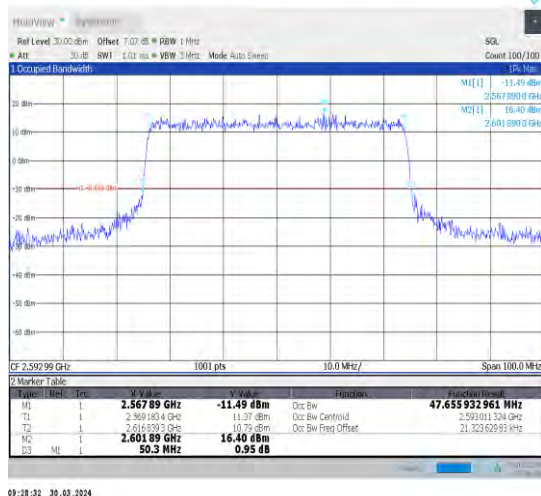
1-N41-30-50-M-8-CP-64QAM-Outer_Full-133@0-Ant t1-47.656-50.300-≤50-PASS
