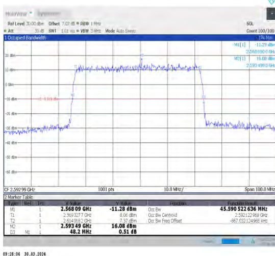
1-N41-30-50-M-5-DFT-256QAM-Outer_Full-128@0-A Ant1-45.591-48.200-≤50-PASS
