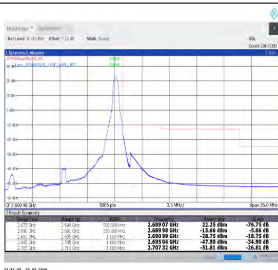
1-N41-30-15-H-2-DFT-PI2BPSK-Edge_1RB_Right-1@37-Ant1-1--PASS-see graph
