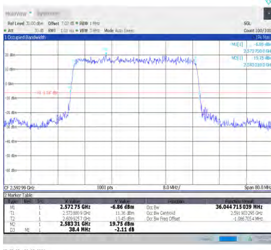
1-N41-30-40-M-2-DFT-PI2BPSK-Outer_Full-100@0-Ant1 Ant1-36.045-38.400-≤40-PASS
