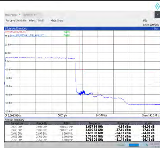
1-N41-30-70-H-3-DFT-PI2BPSK-Outer_Full-180@0-Ant1-1--PASS-see graph
