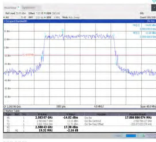
1-N41-30-20-M-2-DFT-PI2BPSK-Outer_Full-50@0-Ant1 -17.887-19.320-≤20-PASS
