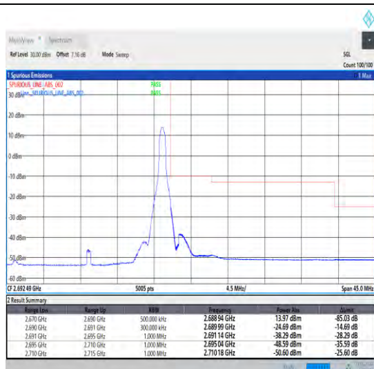
1-N41-30-20-H-2-DFT-PI2BPSK-Edge_1RB_Right-1@50-Ant1-1--PASS-see graph
