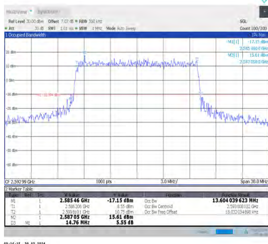
1-N41-30-15-M-8-CP-64QAM-Outer_Full-38@0-Ant1 -13.604-14.760-≤15-PASS
