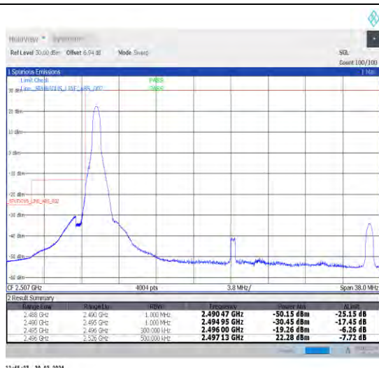
1-N41-30-30-L-1-DFT-PI2BPSK-Edge_1RB_Left-1@0-Ant1-1--PASS-see graph
