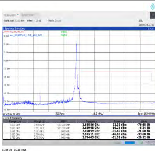
1-N41-30-90-H-5-CP-QPSK-Edge_1RB_Right-1@244-Ant1-1--PASS-see graph
