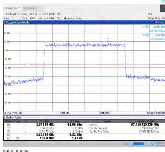
1-N41-30-100-M-9-CP-256QAM-Outer_Full-273@0-A Ant1-97.41-100.800≤100-PASS
