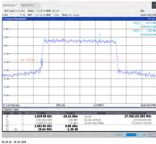
1-N41-30-30-H-9-CP-256QAM-Outer_Full-78@0-Ant 1-27.77-29.640-≤30-PASS
