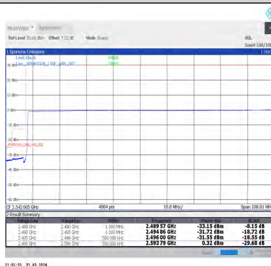
1-N41-30-100-L-6-CP-QPSK-Outer_Full-273@0-Ant1-1--PASS-see graph
