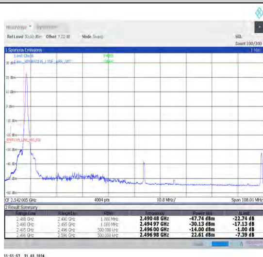
1-N41-30-100-L-4-CP-QPSK-Edge_1RB_Left-1@0-Ant1-1--PASS-see graph
