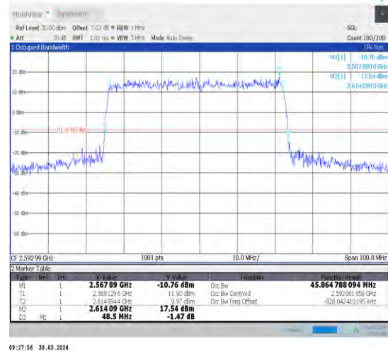
1-N41-30-50-M-4-DFT-64QAM-Outer_Full-128@0-A nt1-45.865-48.500-≤50-PASS
