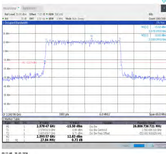
1-N41-30-30-M-4-DFT-64QAM-Outer_Full-75@0-Ant 1-26.808-27.840-≤30-PASS
