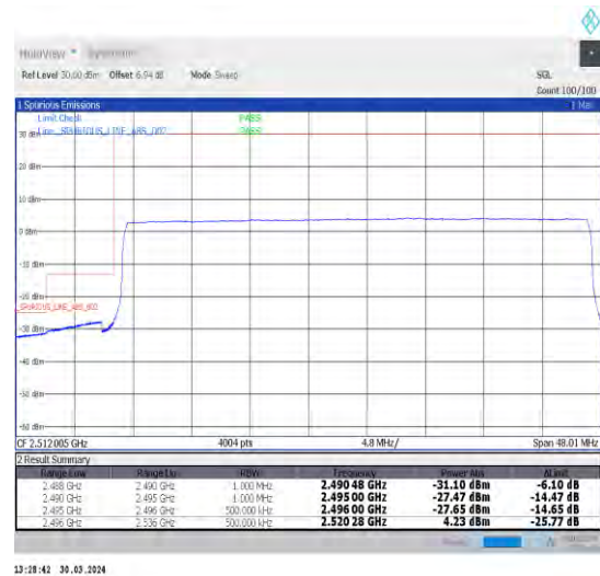
1-N41-30-40-L-6-CP-QPSK-Outer_Full-106@0-Ant1-1--PASS-see graph
