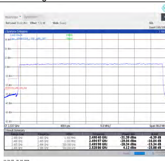
1-N41-30-90-L-3-DFT-PI2BPSK-Outer_Full-240@0-Ant1-1--PASS-see graph
