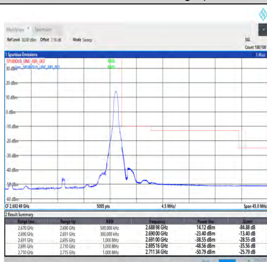
1-N41-30-20-H-5-CP-QPSK-Edge_1RB_Right-1@50-Ant1-1--PASS-see graph
