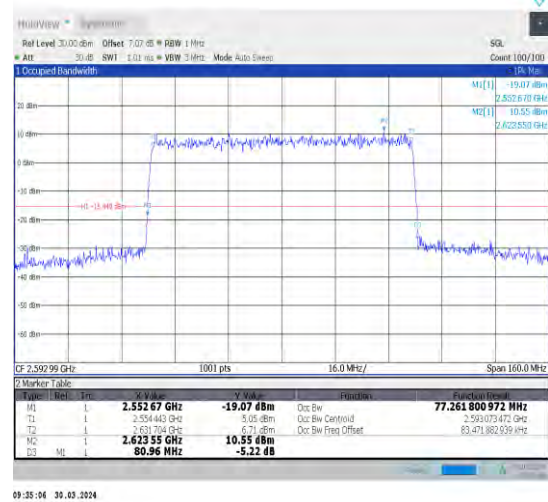
1-N41-30-80-M-9-CP-256QAM-Outer_Full-217@0-A nt1-77.262-80.960-≤80-PASS
