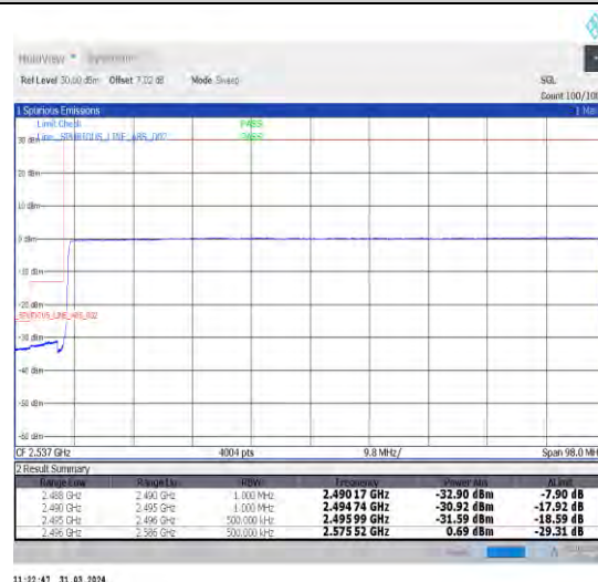
1-N41-30-90-L-6-CP-QPSK-Outer_Full-245@0-Ant1-1--PASS-see graph
