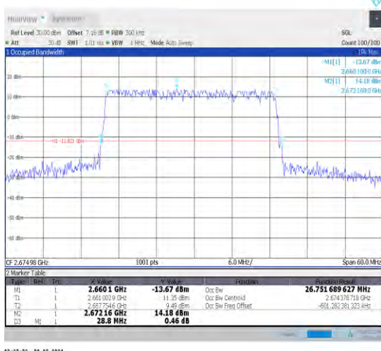
1-N41-30-30-H-3-DFT-16QAM-Outet_Full-75@0-Ant1 1-26.752-28.800-≤30-PASS
