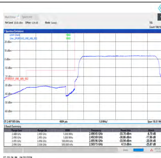
1-N41-30-10-L-3-DFT-PI2BPSK-Outer_Full-24@0-Ant1-1--PASS-see graph
