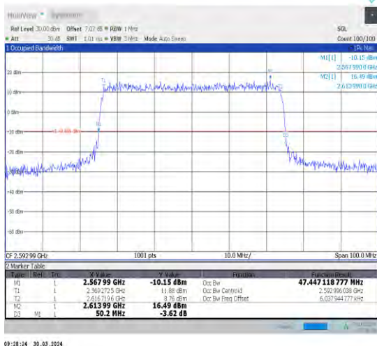
1-N41-30-50-M-7-CP-16QAM-Outer_Full-133@0-Ant 1-47.447-50.200-≤50-PASS
