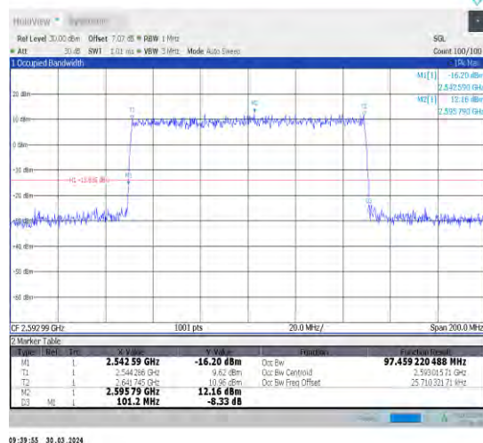
1-N41-30-100-M-7-CP-16QAM-Outer_Full-273@0-A nt1-97.459-101.200≤100-PASS
