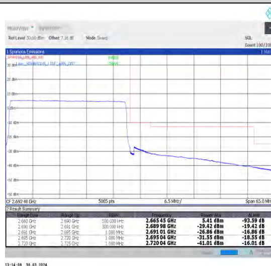
1-N41-30-30-H-6-CP-QPSK-Outer_Full-78@0-Ant1-1--PASS-see graph
