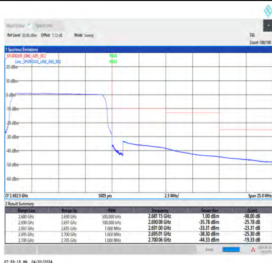
1-N41-30-10-H-6-CP-QPSK-Outer_Full-24@0-Ant1-1--PASS-see graph
