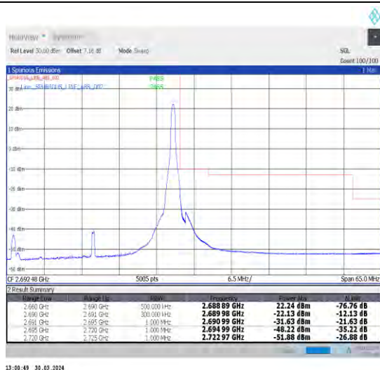
1-N41-30-30-H-2-DFT-PI2BPSK-Edge_1RB_Right-1@77-Ant1-1--PASS-see graph
