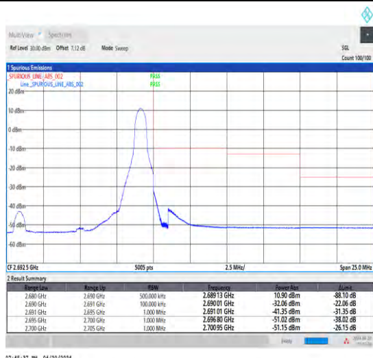
1-N41-30-10-H-2-DFT-PI2BPSK-Edge_1RB_Right-1@23-Ant1-1--PASS-see graph
