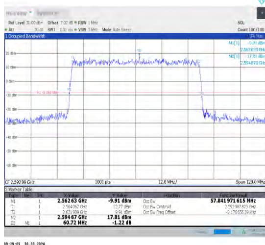
1-N41-30-60-M-1-DFT-QPSK-Outer_Full-162@0-Ant 1-57.842-60.720-≤60-PASS
