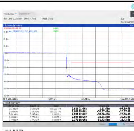
1-N41-30-80-H-6-CP-QPSK-Outer_Full-217@0-A nt1-1--PASS-see graph
