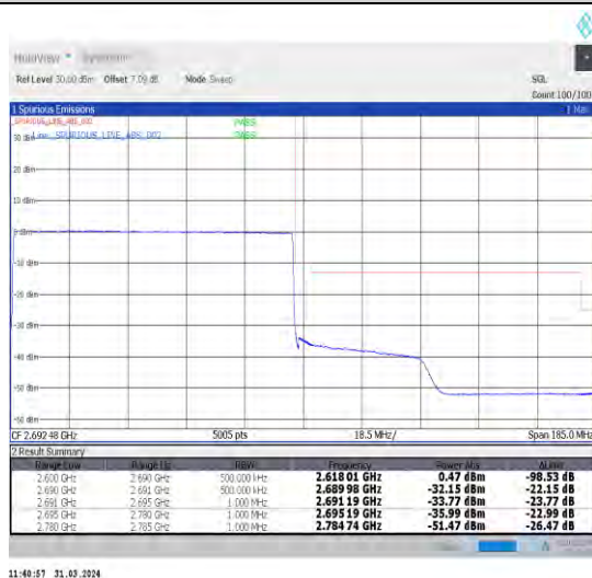
1-N41-30-90-H-6-CP-QPSK-Outer_Full-245@0-Ant1-1--PASS-see graph
