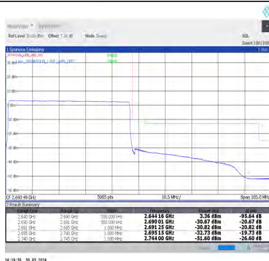
1-N41-30-50-H-6-CP-QPSK-Outer_Full-133@0-Ant1-1--PASS-see graph
