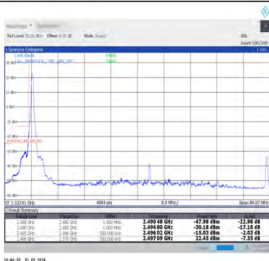
1-N41-30-80-L-4-CP-QPSK-Edge_1RB_Left-1@0-Ant1-1--PASS-see graph
