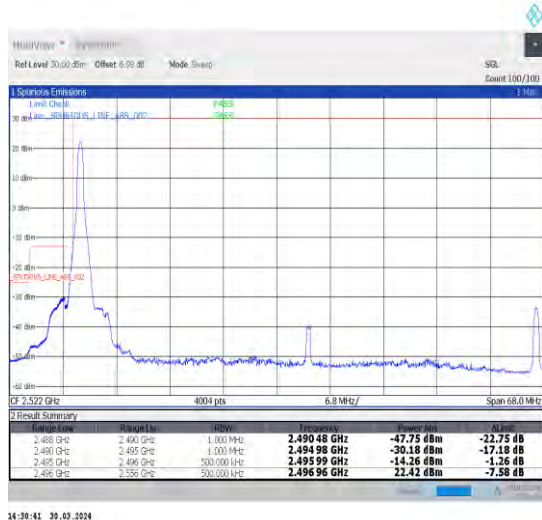
1-N41-30-60-L-4-CP-QPSK-Edge_1RB_Left-1@0-Ant1-1--PASS-see graph
