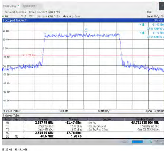
1-N41-30-50-M-3-DFT-16QAM-Outer_Full-128@0-A nt1-45.732-48.600-≤50-PASS
