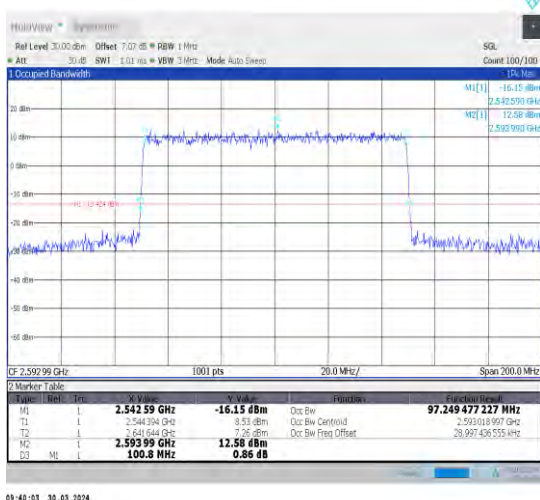
1-N41-30-100-M-8-CP-64QAM-Outer_Full-273@0-A nt1-97.249-100.800≤100-PASS
