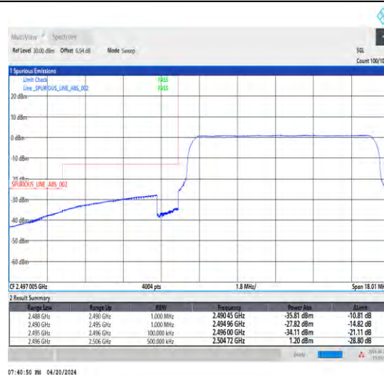
1-N41-30-10-L-6-CP-QPSK-Outer_Full-24@0-Ant1-1--PASS-see graph
