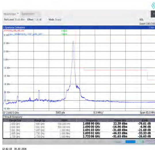
1-N41-30-40-H-5-CP-QPSK-Edge_1RB_Right-1@105-Ant1-1--PASS-see graph
