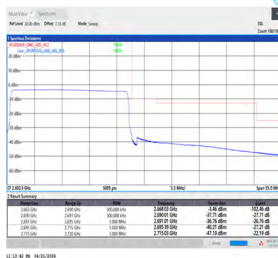
1-N41-30-25-H-6-CP-QPSK-Outer_Full-65@0-Ant1-1--PASS-see graph
