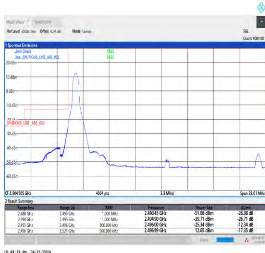
1-N41-30-25-L-4-CP-QPSK-Edge_1RB_Left-1@0-Ant1-1--PASS-see graph
