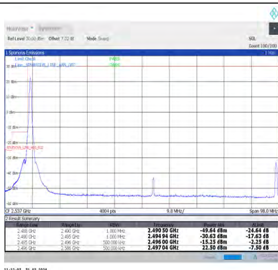
1-N41-30-90-L-1-DFT-PI2BPSK-Edge_1RB_Left-1@0-Ant1-1--PASS-see graph
