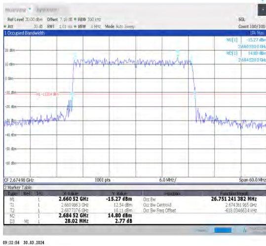
1-N41-30-30-H-1-DFT-QPSK-Outet_Full-75@0-Ant1 -26.752-28.020-≤30-PASS
