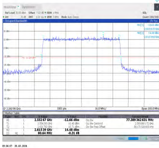
1-N41-30-80-M-8-CP-64QAM-Outer_Full-217@0-Ant 1-77.389-80.640-≤80-PASS
