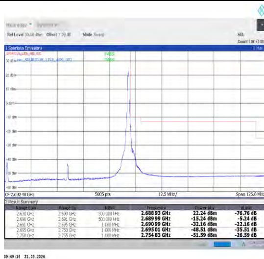
1-N41-30-60-H-2-DFT-PI2BPSK-Edge_1RB_Right-1@161-Ant1-1--PASS-see graph
