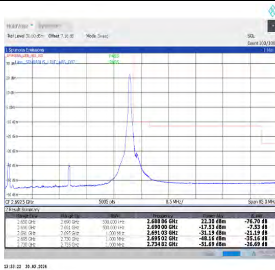
1-N41-30-40-H-2-DFT-PI2BPSK-Edge_1RB_Right-1@105-Ant1-1--PASS-see graph
