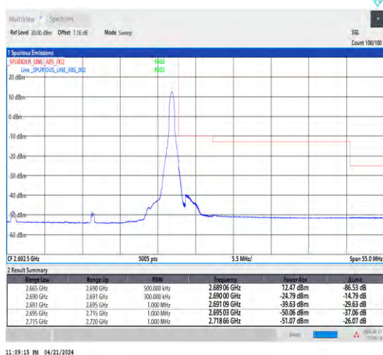
1-N41-30-25-H-5-CP-QPSK-Edge_1RB_Right-1@64-Ant1-1--PASS-see graph
