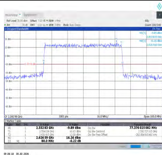
1-N41-30-80-M-3-DFT-16QAM-Outer_Full-216@0-A nt1-77.376-80.000-≤80-PASS
