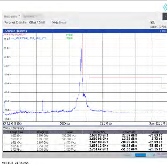
1-N41-30-60-H-5-CP-QPSK-Edge_1RB_Right-1@161-Ant1-1--PASS-see graph
