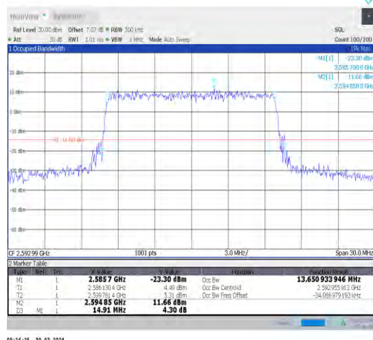
1-N41-30-15-M-9-CP-256QAM-Outer_Full-38@0-Ant1 -13.651-14.910-≤15-PASS
