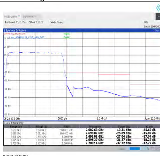
1-N41-30-10-H-3-DFT-PI2BPSK-Outer_Full-24@0-Ant1-1--PASS-see graph
