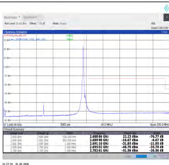
1-N41-30-90-H-2-DFT-PI2BPSK-Edge_1RB_Right-1@244-Ant1-1--PASS-see graph
