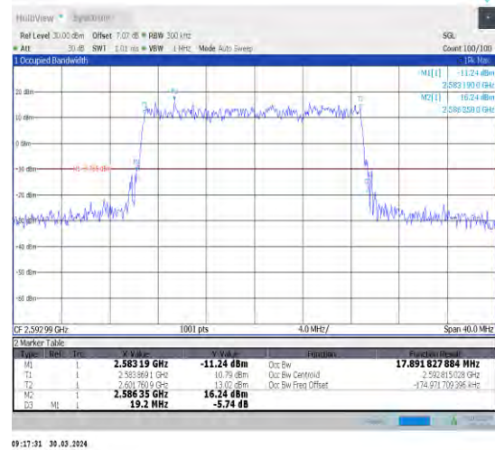
1-N41-30-20-M-4-DFT-64QAM-Outer_Full-50@0-Ant 1-17.892-19.200-≤20-PASS
