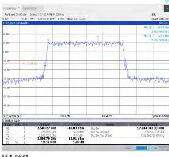
1-N41-30-20-M-5-DFT-256QAM-Outer_Full-50@0-Ant 1-17.844-19.320-≤20-PASS
