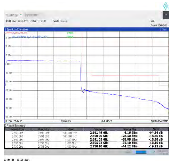
1-N41-30-40-H-6-CP-QPSK-Outer_Full-106@0-Ant1-1--PASS-see graph
