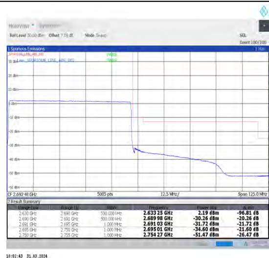
1-N41-30-60-H-6-CP-QPSK-Outer_Full-162@0-Ant1-1--PASS-see graph
