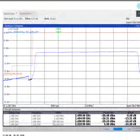
1-N41-30-30-L-6-CP-QPSK-Outer_Full-78@0-Ant1-1--PASS-see graph
