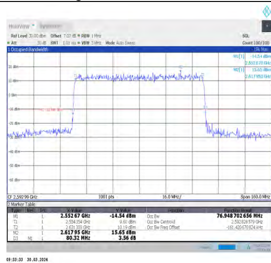
1-N41-30-80-M-1-DFT-QPSK-Outer_Full-216@0-Ant 1-76.949-80.320-≤80-PASS
