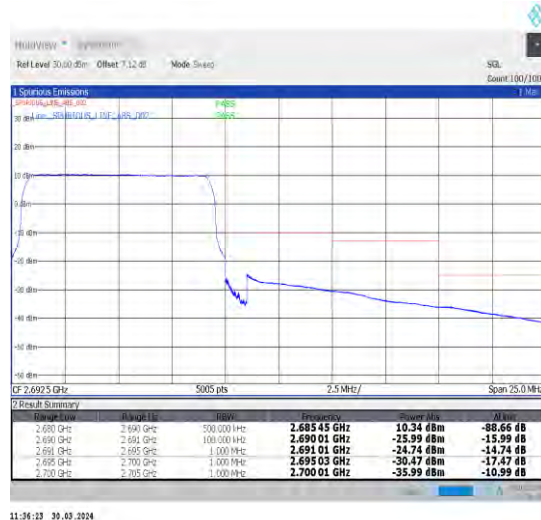
1-N41-30-10-H-6-CP-QPSK-Outer_Full-24@0-Ant1-1--PASS-see graph
