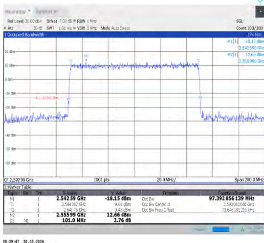
1-N41-30-100-M-6-CP-QPSK-Outer_Full-273@0-Ant 1-97.393-101.000≤100-PASS
