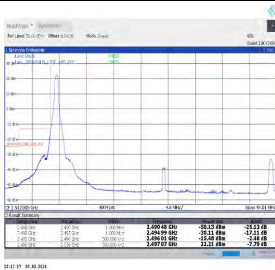
1-N41-30-40-L-1-DFT-PI2BPSK-Edge_1RB_Left-1@0-Ant1-1--PASS-see graph
