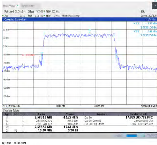
1-N41-30-20-M-3-DFT-16QAM-Outer_Full-50@0-Ant 1-17.889-19.280-≤20-PASS
