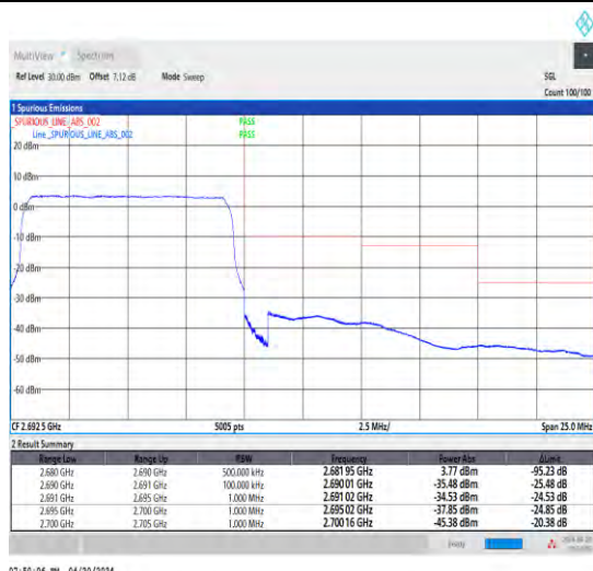
1-N41-30-10-H-3-DFT-PI2BPSK-Outer_Full-24@0-Ant1-1--PASS-see graph
