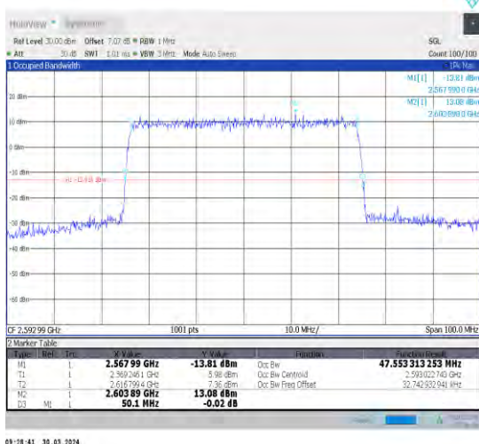
1-N41-30-50-M-9-CP-256QAM-Outer_Full-133@0-A nt1-47.553-50.100-≤50-PASS
