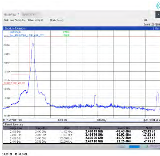
1-N41-30-40-L-4-CP-QPSK-Edge_1RB_Left-1@0-Ant1-1--PASS-see graph
