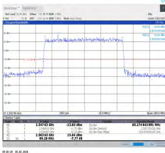
1-N41-30-90-M-1-DFT-QPSK-Outer_Full-240@0-Ant 1-85.275-89.280-≤90-PASS
