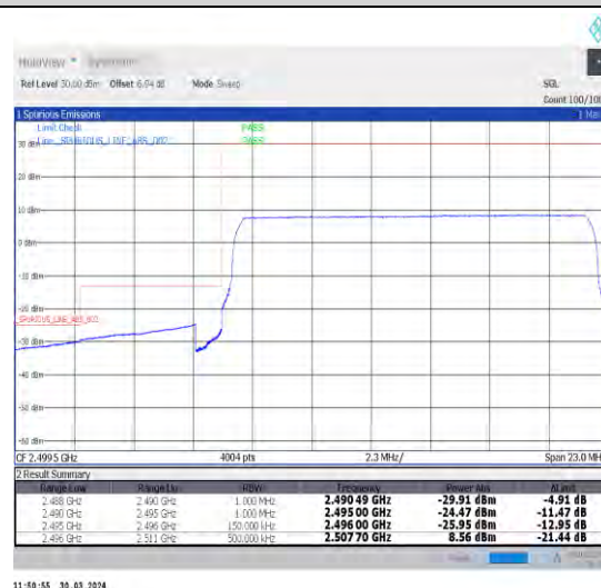
1-N41-30-15-L-6-CP-QPSK-Outer_Full-38@0-Ant1-1--PASS-see graph
