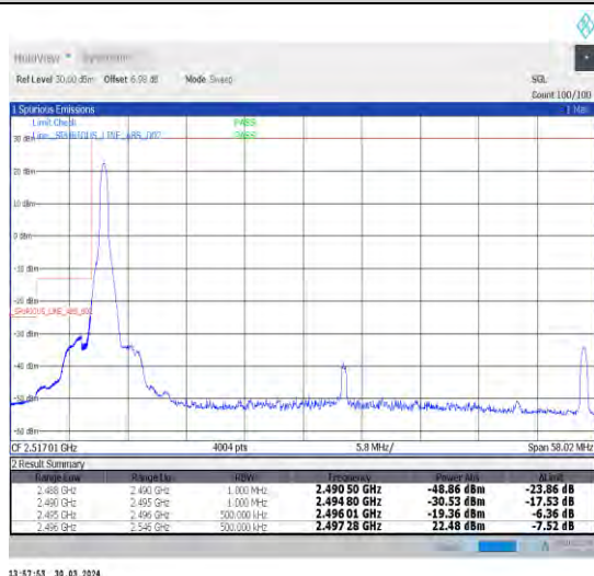
1-N41-30-50-L-4-CP-QPSK-Edge_1RB_Left-1@0-Ant1-1--PASS-see graph
