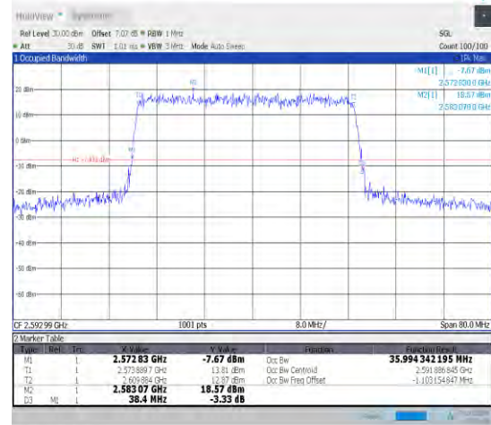
1-N41-30-40-M-1-DFT-QPSK-Outer_Full-100@0-Ant 1-35.994-38.400-≤40-PASS
