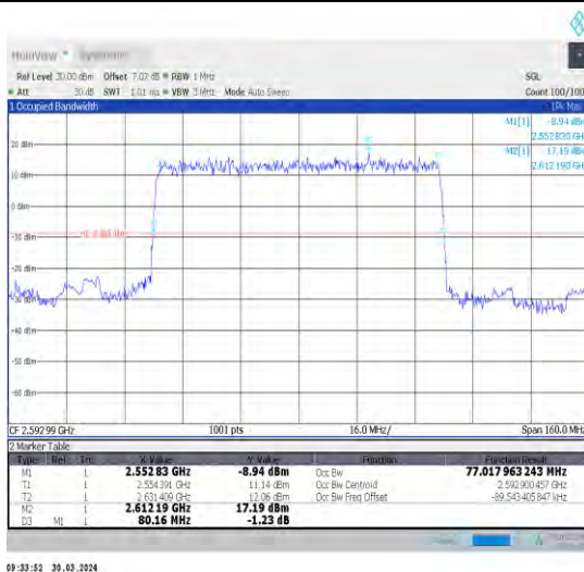
1-N41-30-80-M-2-DFT-PI2BPSK-Outer_Full-216@0-Ant1 Ant1-77.018-80.160-≤80-PASS
