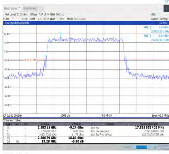
1-N41-30-20-M-1-DFT-QPSK-Outer_Full-50@0-Ant1 -17.856-19.280-≤20-PASS
