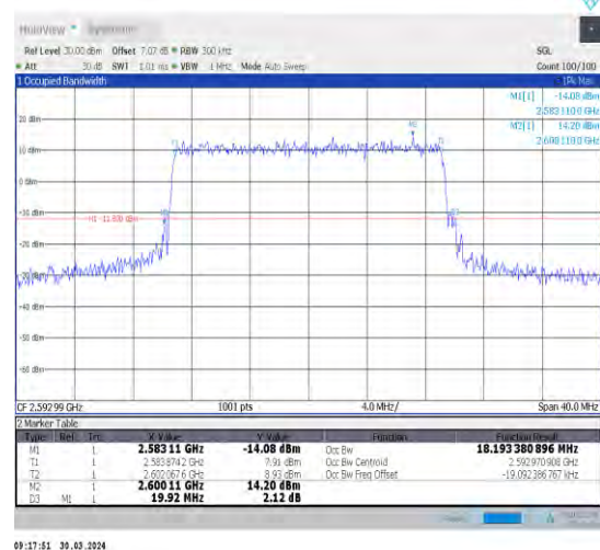
1-N41-30-20-M-6-CP-QPSK-Outer_Full-51@0-Ant 1-18.193-19.920-≤20-PASS
