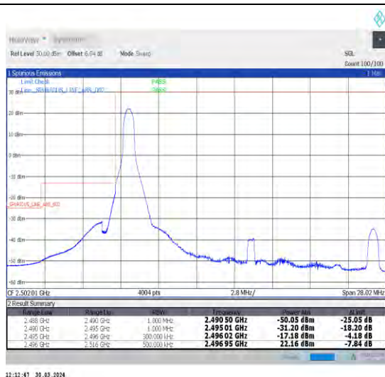
1-N41-30-20-L-1-DFT-PI2BPSK-Edge_1RB_Left-1@0-Ant1-1--PASS-see graph
