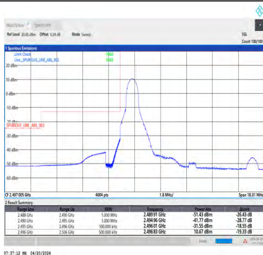
1-N41-30-10-L-4-CP-QPSK-Edge_1RB_Left-1@0-Ant1-1--PASS-see graph
