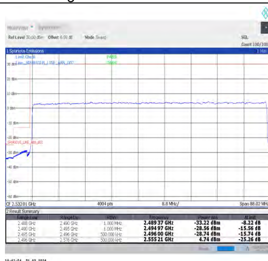
1-N41-30-80-L-3-DFT-PI2BPSK-Outer_Full-216@0-Ant1-1--PASS-see graph
