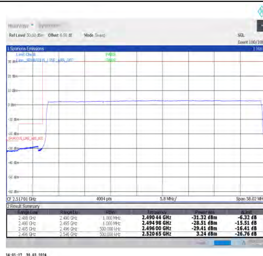
1-N41-30-50-L-6-CP-QPSK-Outer_Full-133@0-Ant1-1--PASS-see graph
