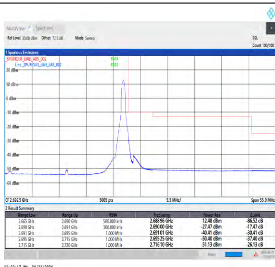
1-N41-30-25-H-2-DFT-PI2BPSK-Edge_1RB_Right-1@64-Ant1-1--PASS-see graph
