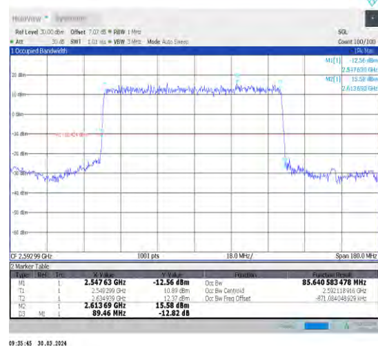
1-N41-30-90-M-2-DFT-PI2BPSK-Outer_Full-240@0- Ant1-85.641-89.460-≤90-PASS
