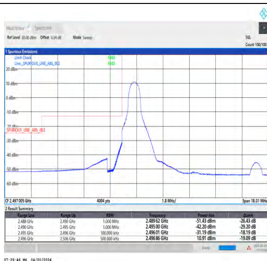
1-N41-30-10-L-1-DFT-PI2BPSK-Edge_1RB_Left-1@0-Ant1-1--PASS-see graph
