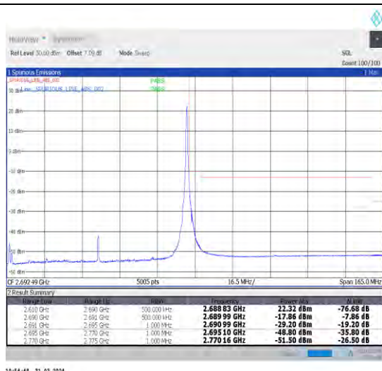
1-N41-30-80-H-2-DFT-PI2BPSK-Edge_1RB_Right-1@ 216-Ant1-1--PASS-see graph
