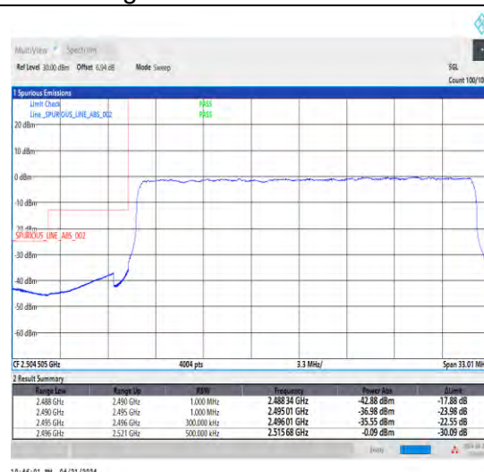
1-N41-30-25-L-3-DFT-PI2BPSK-Outer_Full-64@0-Ant1-1--PASS-see graph
