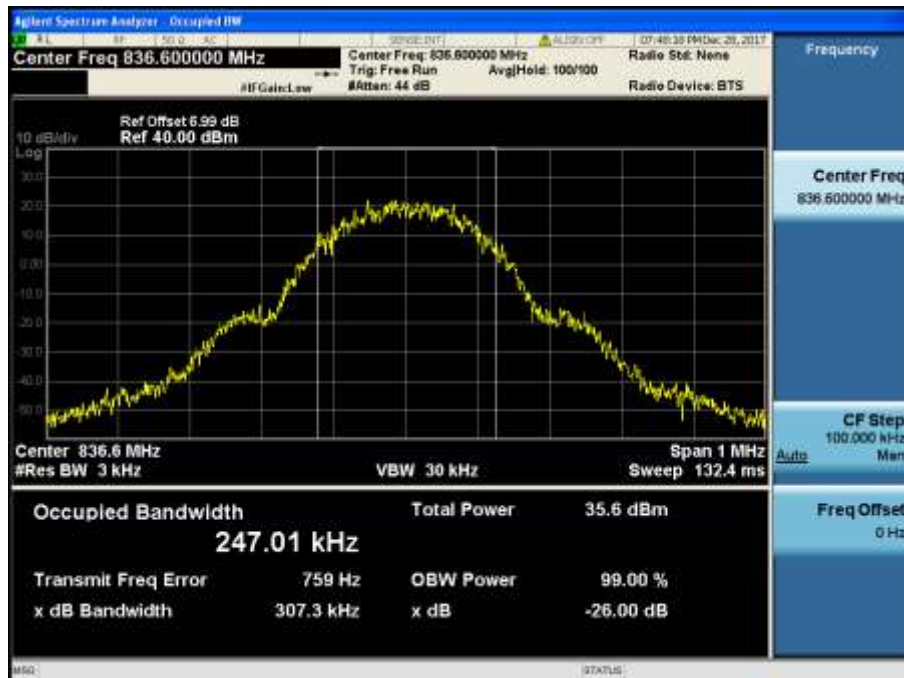
GSM850 & Channel: 190
