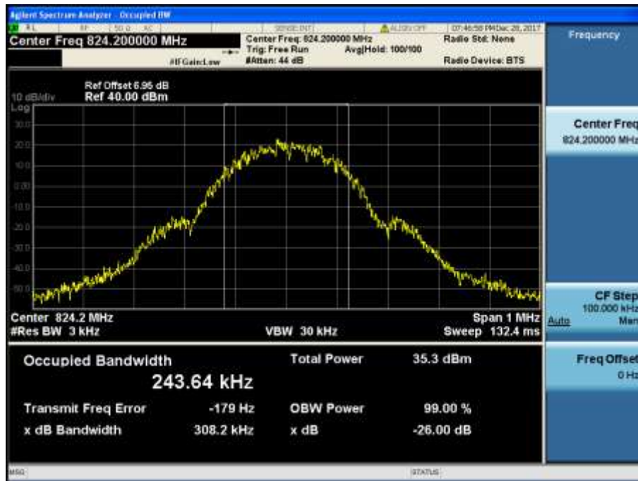
GSM850 & Channel: 128
