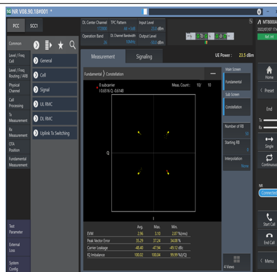
1-N26-814-824--15-10-M-2-DFT-QPSK-Outer_Full-50@0-Ant1-see graph-PASS
