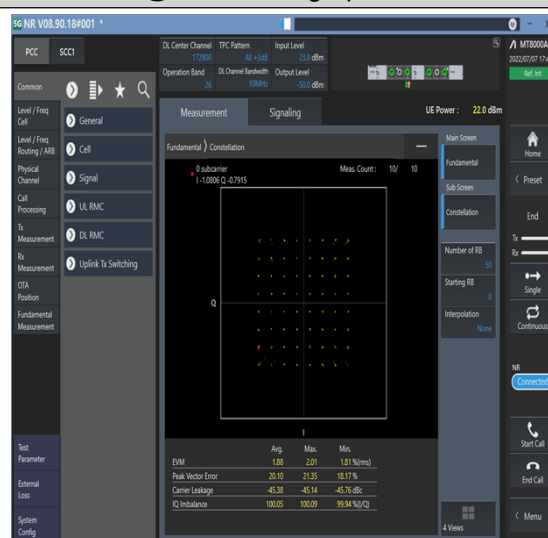
1-N26-814-824--15-10-M-4-DFT-64QAM-Outer_Full-50@0-Ant1-see graph-PASS
