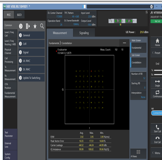
1-N26-814-824--15-10-M-8-CP-64QAM-Outer_Full-52@0-Ant1-see graph-PASS
