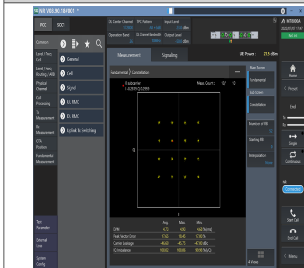
1-N26-814-824--15-10-M-7-CP-16QAM-Outer_Full-52@0-Ant1-see graph-PASS
