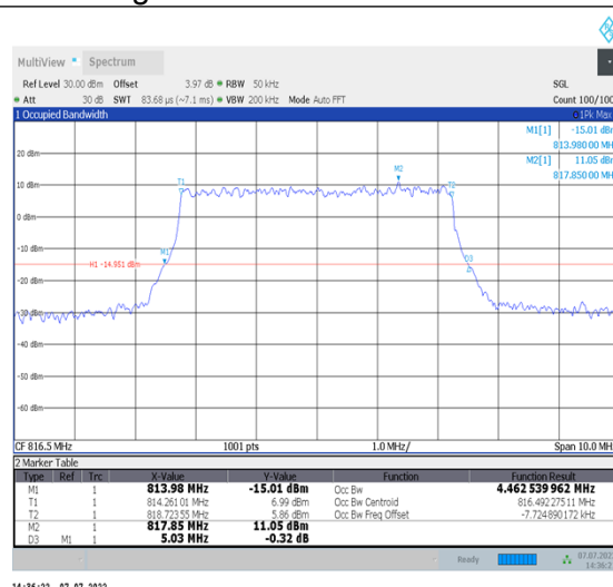
1-N26-814-824--15-5-L-6-CP-QPSK-Outer_Full-25@0-Ant1-4.463-5.030-≤5-PASS
