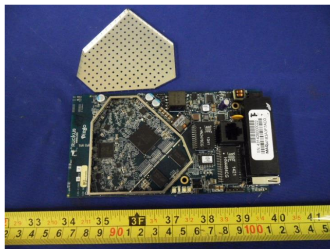
Main Board without Shielding Top View
