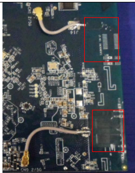
Antenna Location
