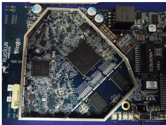
Main Board without Shielding Close View
