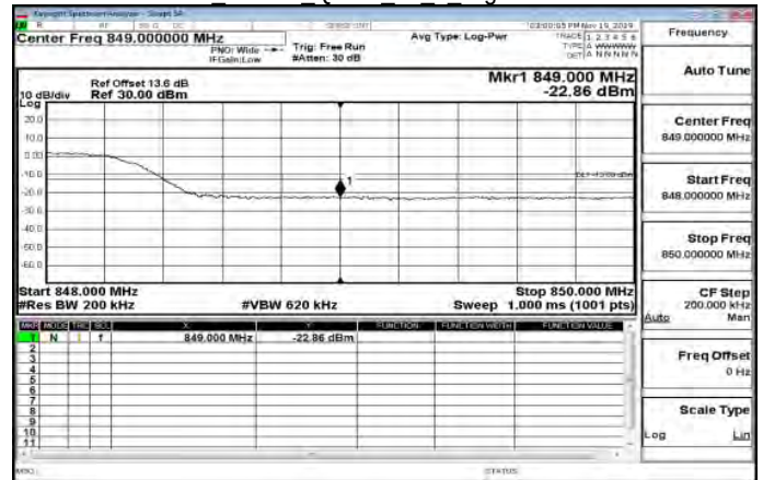
LTE\Band26 15MHz QPSK 75 0 HighCH26965-841.5
