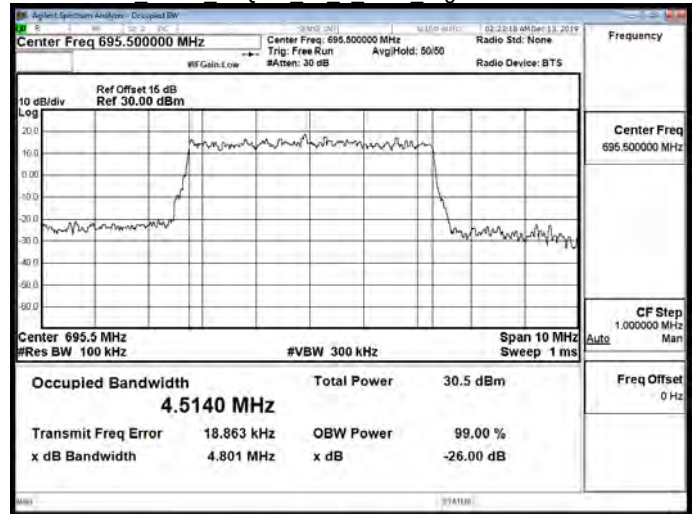
Band71 5MHz 64QAM 25 0 Main High CH133447-695.5
