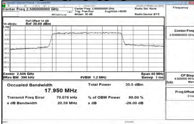
Band41 20MHz QPSK 100 0 Main LowCH39750-2506
