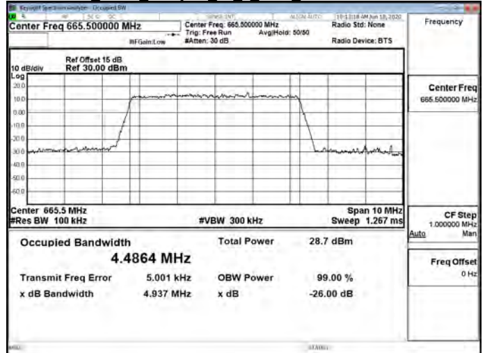
Band71 5MHz 256QAM 25 0 Main Low CH133147-665.5
