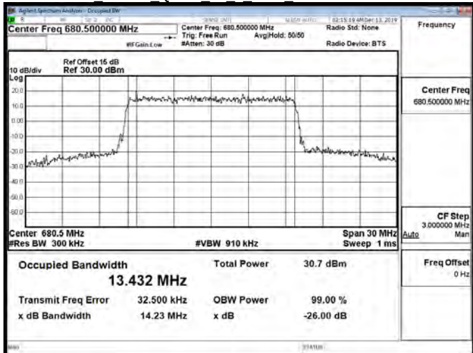
Band71 15MHz QPSK 75 0 Main Mid CH133297-680.5
