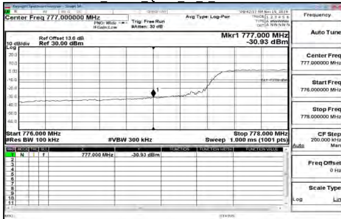
LTE\Band13 10MHz QPSK 50 0 LowCH23230-782
