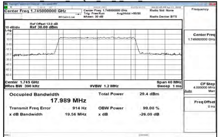
Band66 20MHz 256QAM 100 0 Main MidCH132322-1745
