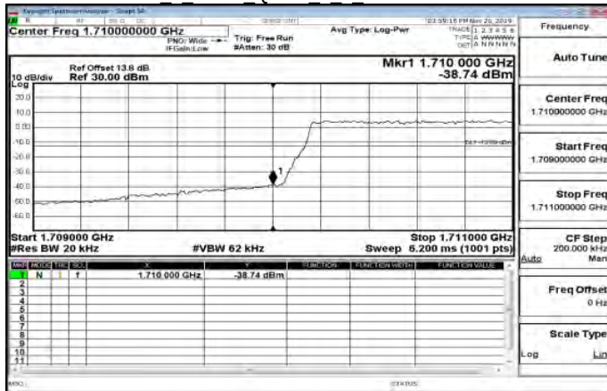
LTE\Band66 1 4MHz QPSK 6 0 LowCH131979-1710.7
