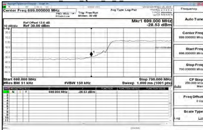
LTE\Band12 5MHz QPSK 25 0 LowCH23035-701.5
