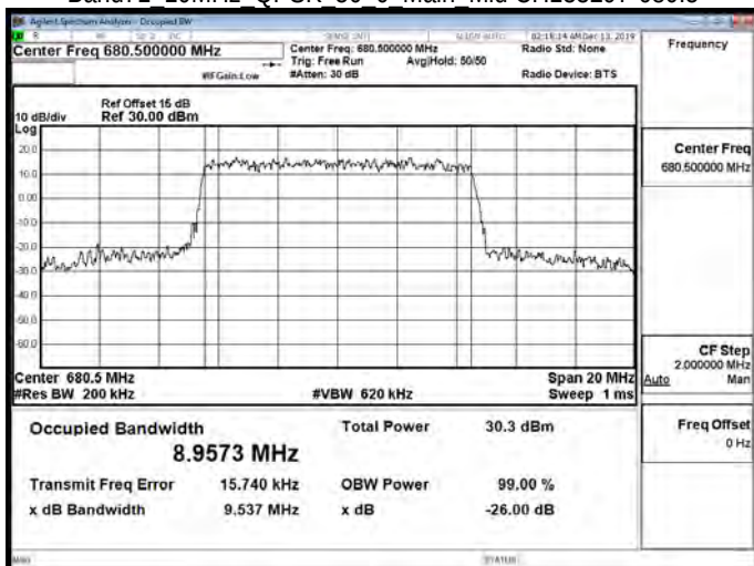
Band71 10MHz QPSK 50 0 Main Mid CH133297-680.5
