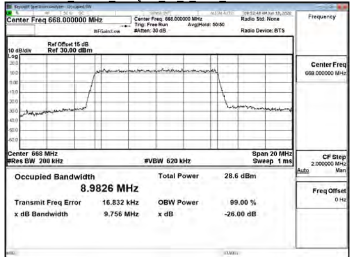
Band71 10MHz 256QAM 50 0 Main Low CH133172-668
