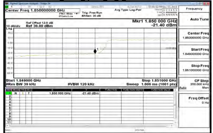
LTE\Band25 3MHz QPSK 15 0 LowCH26055-1851.5
