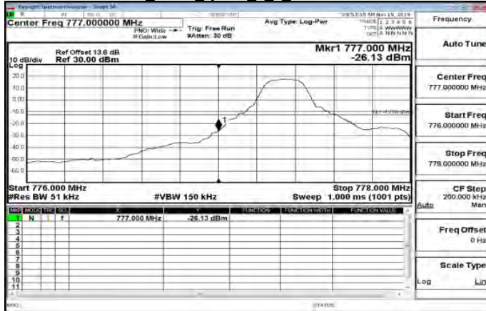
LTE\Band13 5MHz QPSK 1 0 LowCH23205-779.5
