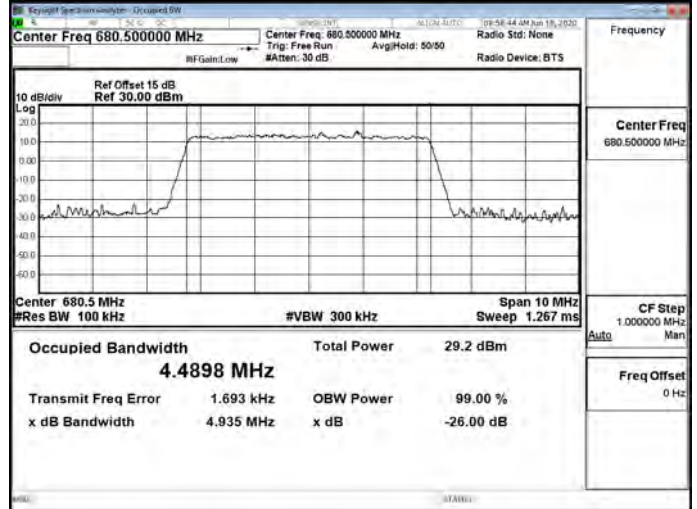
Band71 5MHz 256QAM 25 0 Main Mid CH133297-680.5
