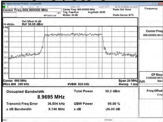
Band71 10MHz 64QAM 50 0 Main Low CH133172-668
