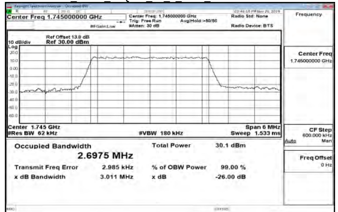
Band66 3MHz 16QAM 15 0 Main MidCH132322-1745
