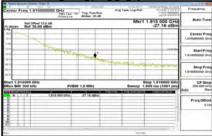
LTEBand25 20MHz QPSK 1 99 HighCH26590-1905
