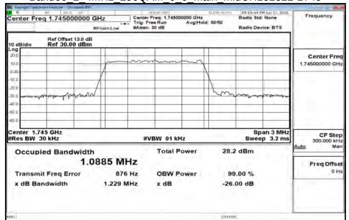
Band66 1 4MHz 256QAM 6 0 Main MidCH132322-1745
