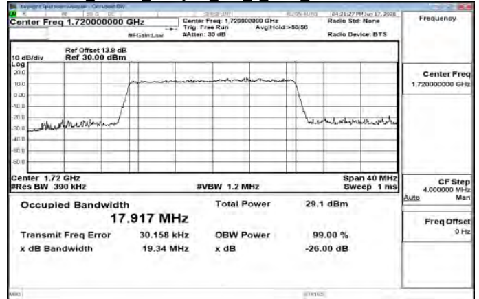
Band66 20MHz 256QAM 100 0 Main LowCH132072-1720
