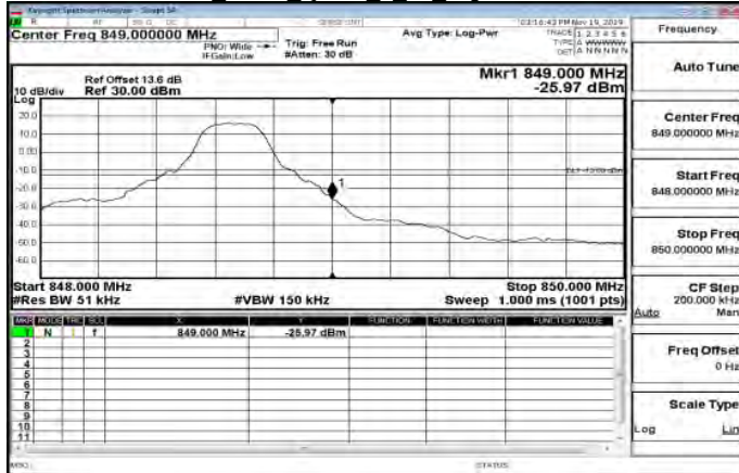
LTE\Band26 5MHz QPSK 1 24 HighCH27015-846.5
