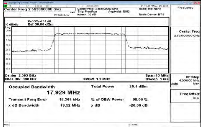
Band41 20MHz 16QAM 100 0 Main MidCH40620-2593
