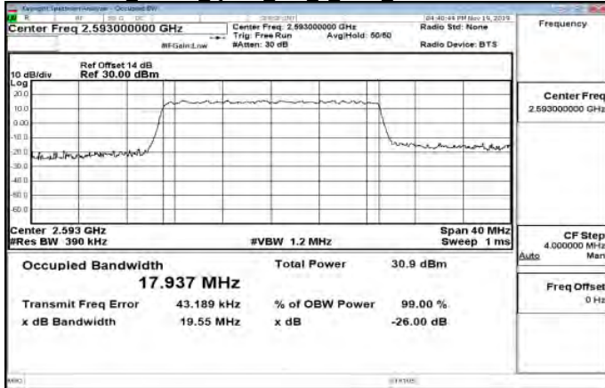
Band41 20MHz QPSK 100 0 Main MidCH40620-2593
