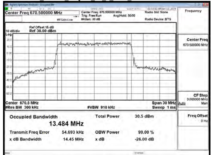
Band71 15MHz 16QAM 75 0 Main Low CH133197-670.5
