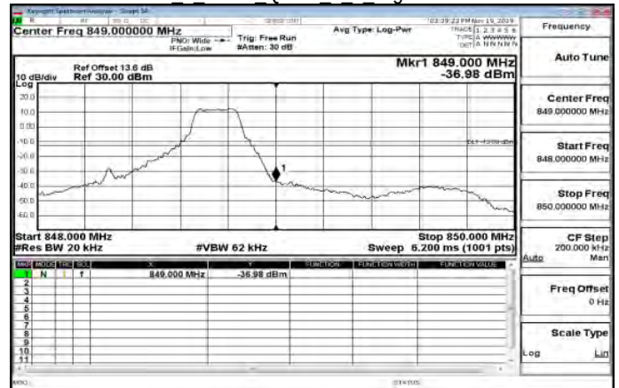
LTEBand26 1 4MHz QPSK 1 5 HighCH27033-848.3
