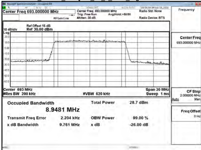
Band71 10MHz 256QAM 50 0 Main High CH133422-693
