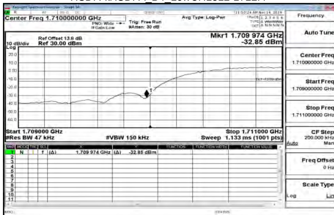
HSDPA\HSDPA B4 LowCH1312-1712.4
