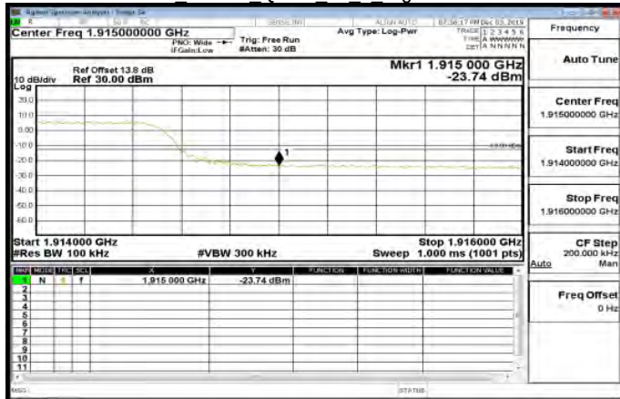
LTE\Band25 10MHz QPSK 50 0 HighCH26640-1910
