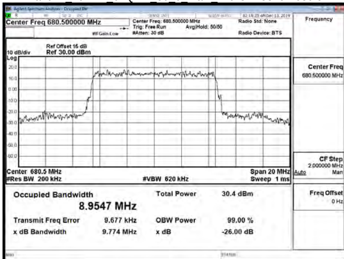
Band71 10MHz 64QAM 50 0 Main Mid CH133297-680.5
