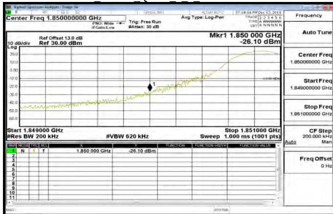
LTE\Band25 15MHz QPSK 1 0 LowCH26115-1857.5
