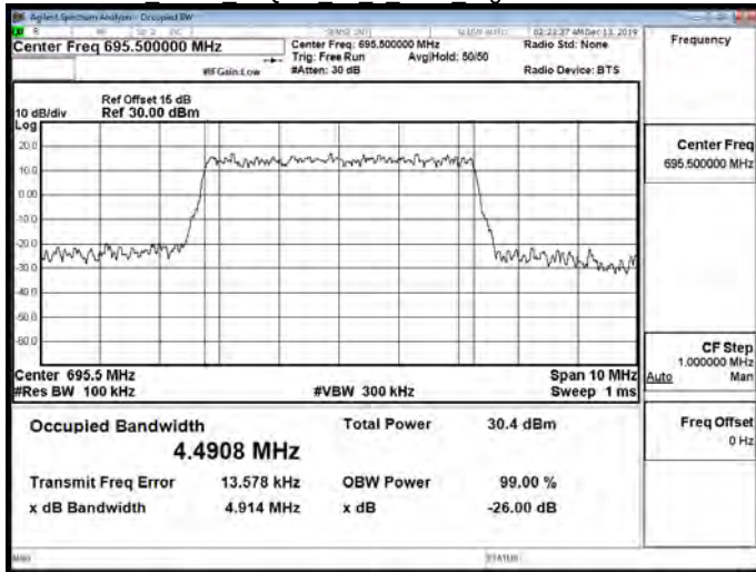
Band71 5MHz 16QAM 25 0 Main High CH133447-695.5
