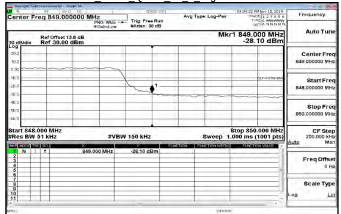
LTE\Band5 5MHz QPSK 25 0 HighCH20625-846.5
