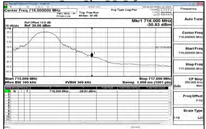
LTE\Band12 10MHz QPSK 1 49 HighCH23130-711
