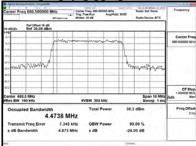
Band71 5MHz 64QAM 25 0 Main Mid CH133297-680.5
