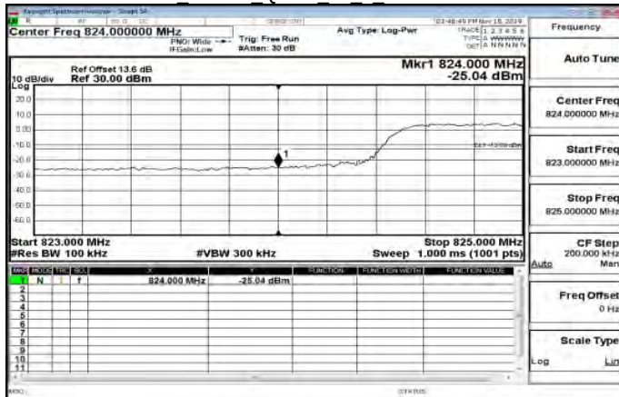
LTEBand5 10MHz QPSK 50 0 LowCH20450-829
