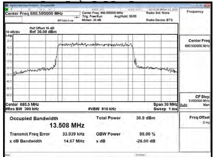
Band71 15MHz 16QAM 75 0 Main Mid CH133297-680.5
