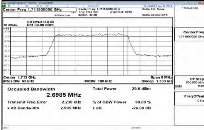
Band66 3MHz QPSK 15 0 Main LowCH131987-1711.5
