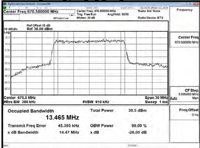
Band71 15MHz QPSK 75 0 Main Low CH133197-670.5
