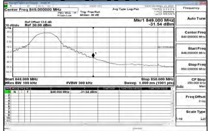
LTE\Band26 10MHz QPSK 1 49 HighCH26990-844
