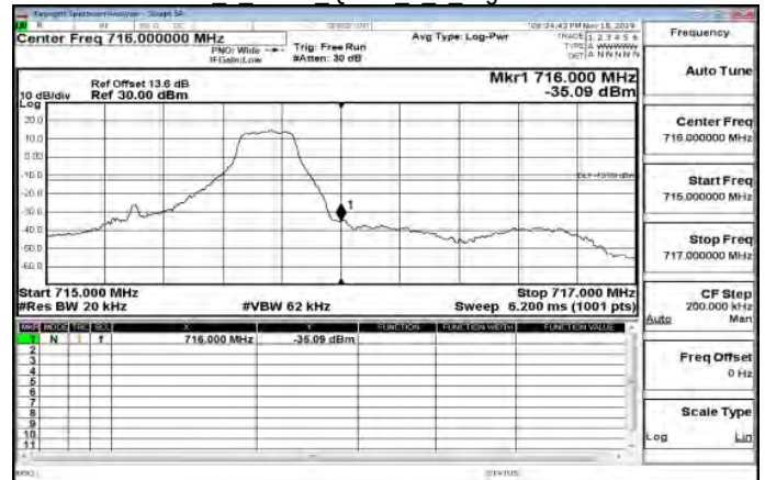
LTEBand12 1 4MHz QPSK 1 5 HighCH23173-715.3
