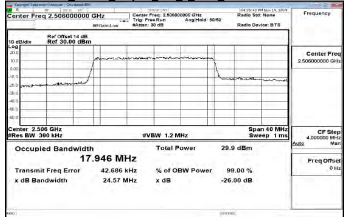
Band41 20MHz 16QAM 100 0 Main LowCH39750-2506
