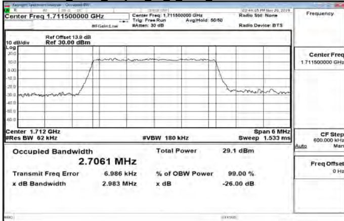
Band66 3MHz 64QAM 15 0 Main LowCH131987-1711.5
