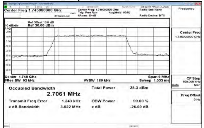
Band66 3MHz 256QAM 15 0 Main MidCH132322-1745
