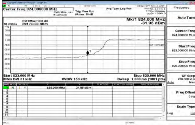
LTE\Band26 5MHz QPSK 25 0 LowCH26815-826.5
