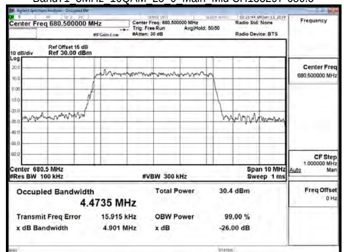
Band71 5MHz 16QAM 25 0 Main Mid CH133297-680.5
