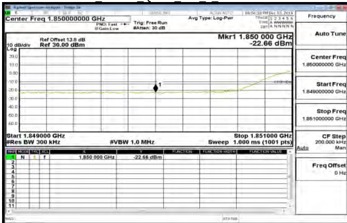
LTEBand25 20MHz QPSK 100 0 LowCH26140-1860
