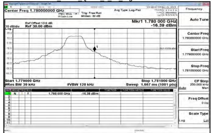
LTE\Band66 3MHz QPSK 1 14 HighCH132657-1778.5
