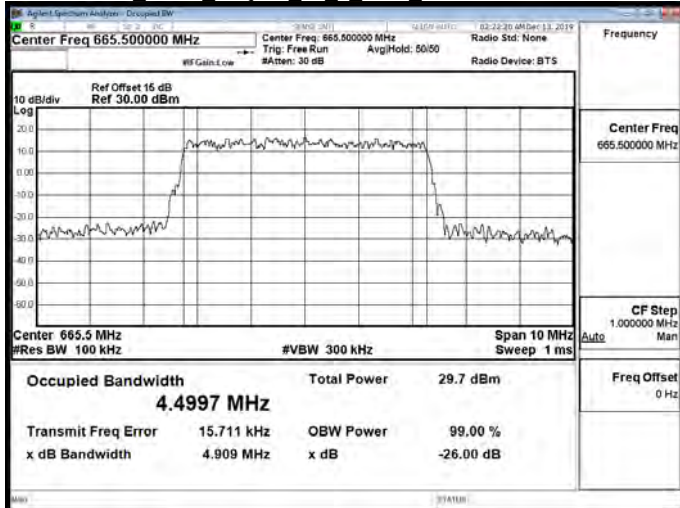
Band71 5MHz 64QAM 25 0 Main Low CH133147-665.5
