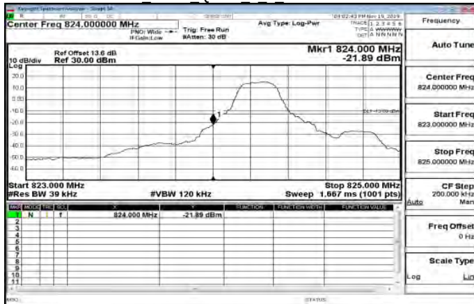
LTE\Band26 3MHz QPSK 1 0 LowCH26805-825.5
