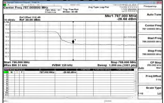
LTE\Band13 5MHz QPSK 25 0 HighCH23255-784.5
