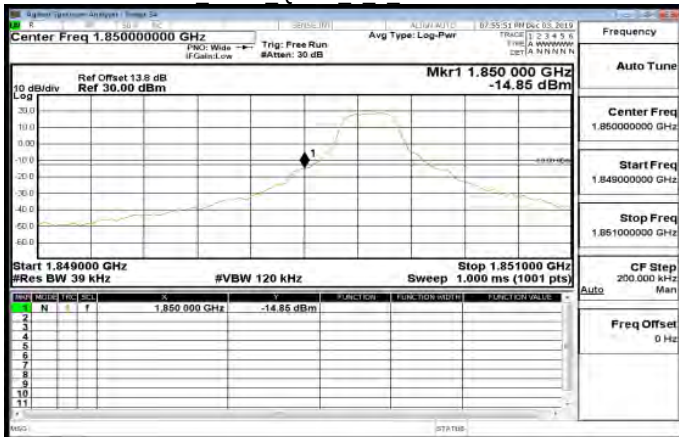
LTE\Band25 3MHz QPSK 1 0 LowCH26055-1851.5
