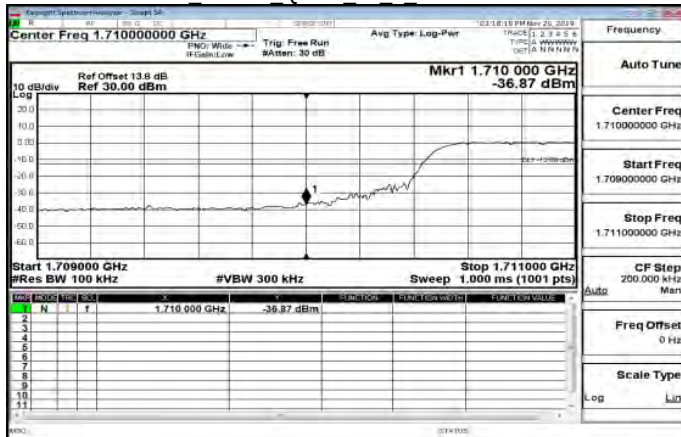
LTE\Band66 10MHz QPSK 50 0 LowCH132022-1715
