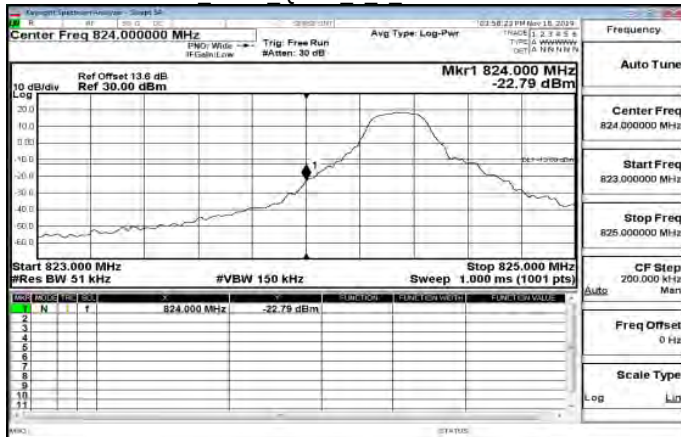
LTE\Band5 5MHz QPSK 1 0 LowCH20425-826.5
