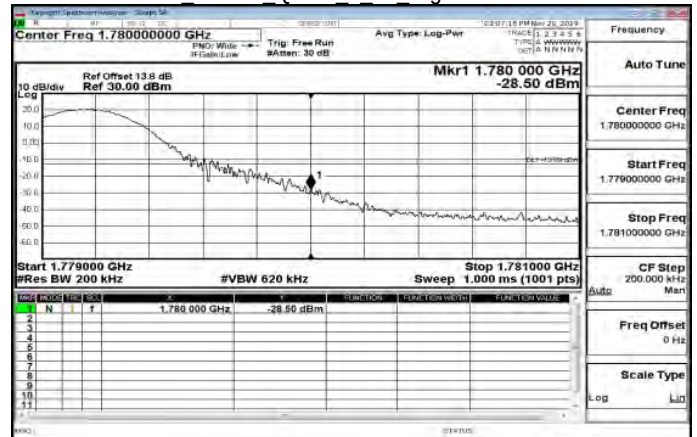
LTE\Band66 15MHz QPSK 1 74 HighCH132597-1772.5
