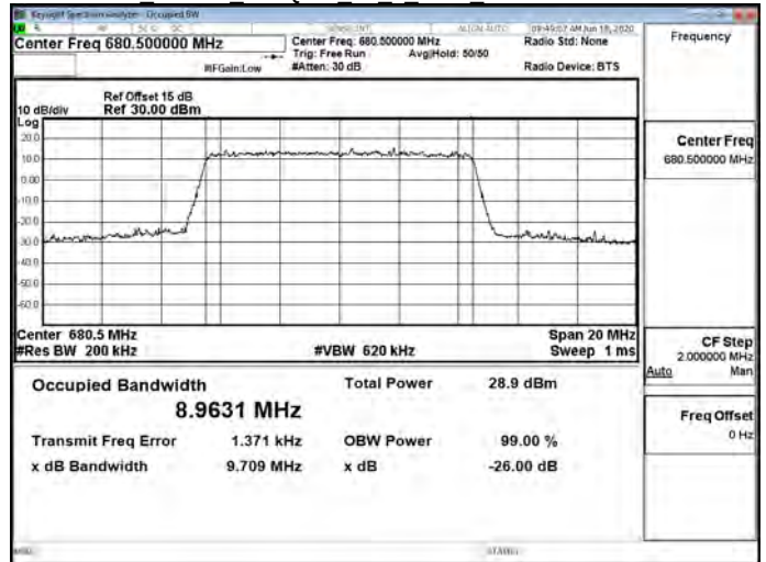
Band71 10MHz 256QAM 50 0 Main Mid CH133297-680.5
