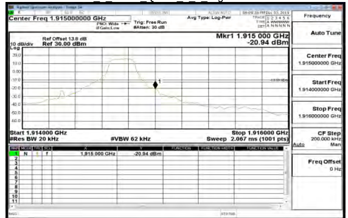
LTE\Band25 1 4MHz QPSK 1 5 HighCH26683-1914.3
