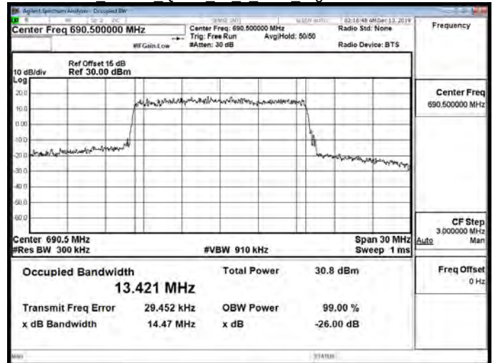
Band71 15MHz QPSK 75 0 Main High CH133397-690.5
