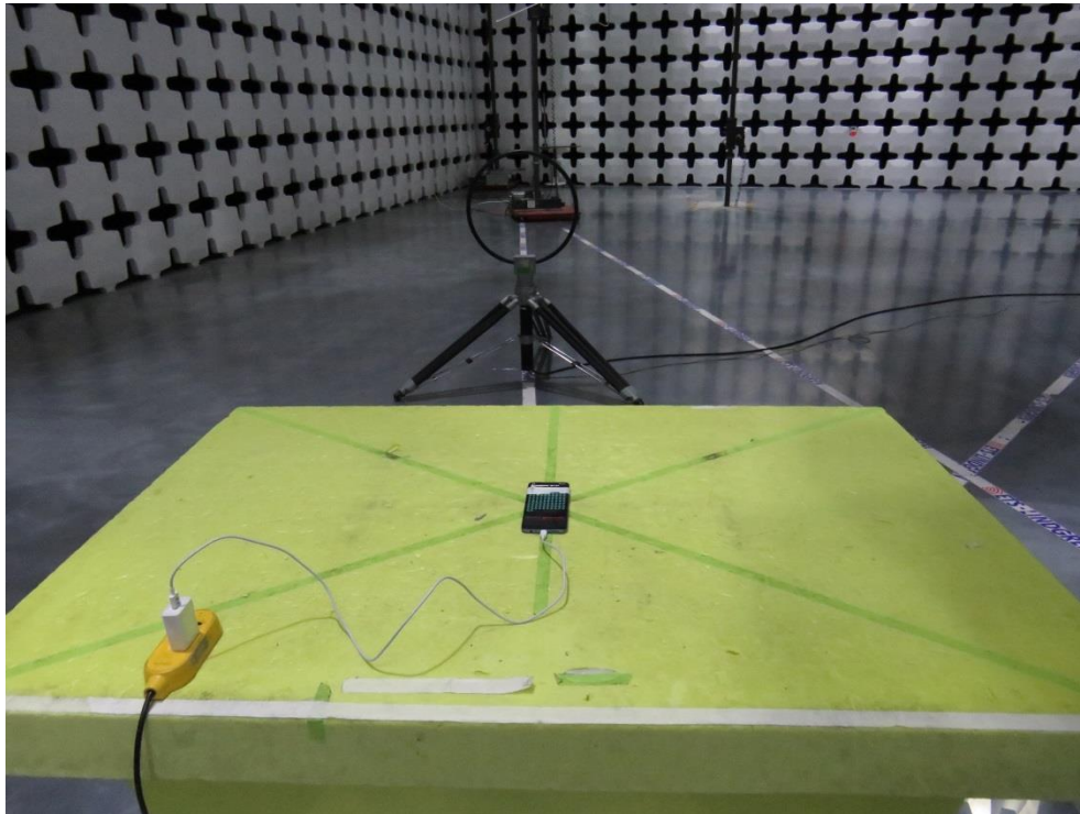
Part15C_RE_NFC_1
