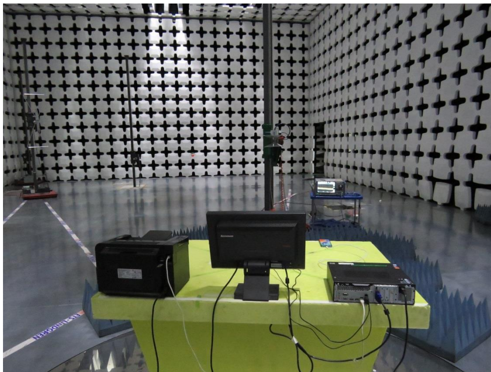
Part15B_RE_H3
