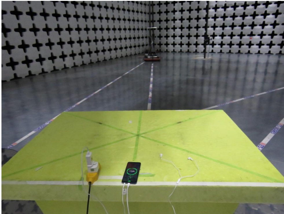
Part15C_RE_NFC_3
