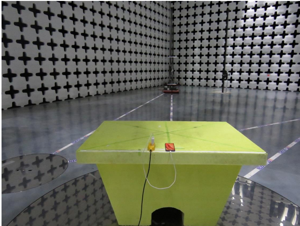
Part15B_RE_L2
