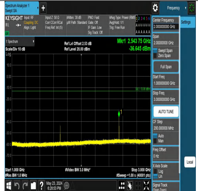
Band5_1.4MHz_QPSK_20643_1RB#0_1000~3000_1000~3000
