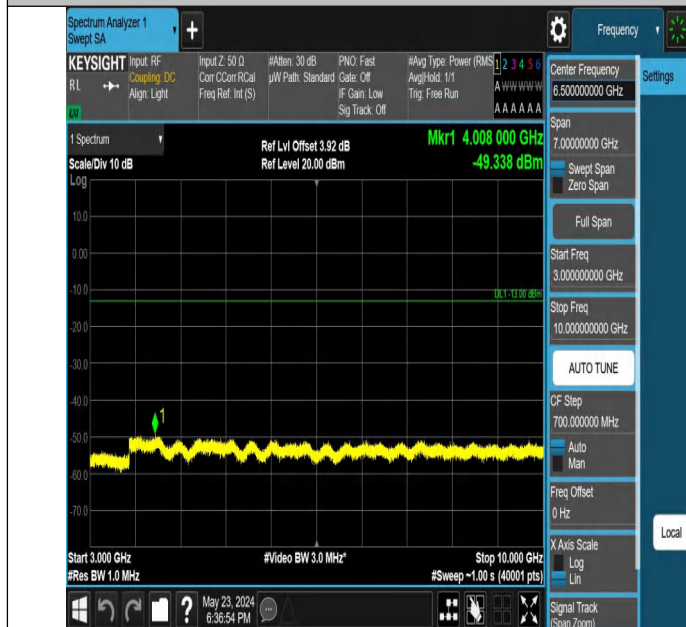
Band5_3MHz_QPSK_20635_1RB#0_3000~10000_3000~10000
