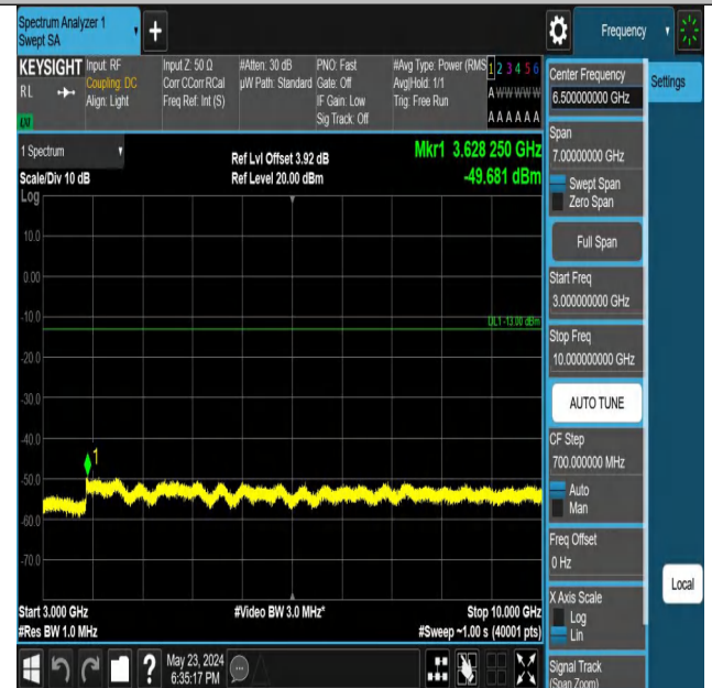
Band5_3MHz_QPSK_20415_1RB#14_3000~10000_3000~10000
