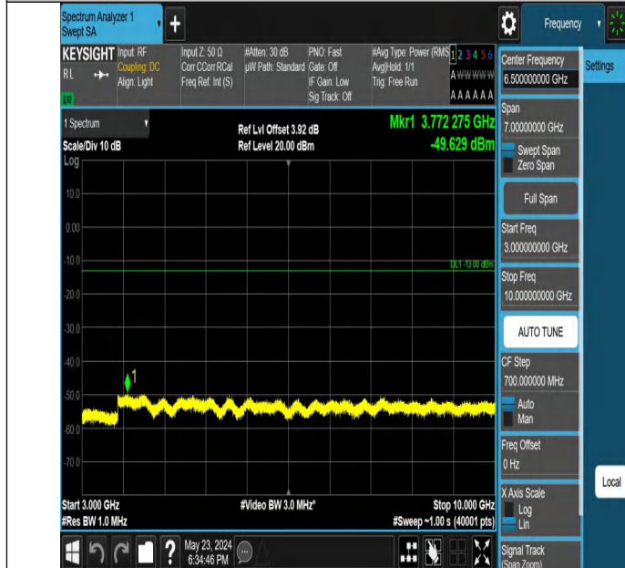
Band5_3MHz_QPSK_20415_1RB#0_3000~10000_3000~10000
