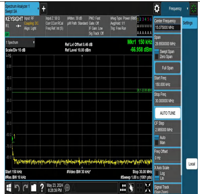
Band5_1.4MHz_QPSK_20643_1RB#0_0.15~30_0.15~30
