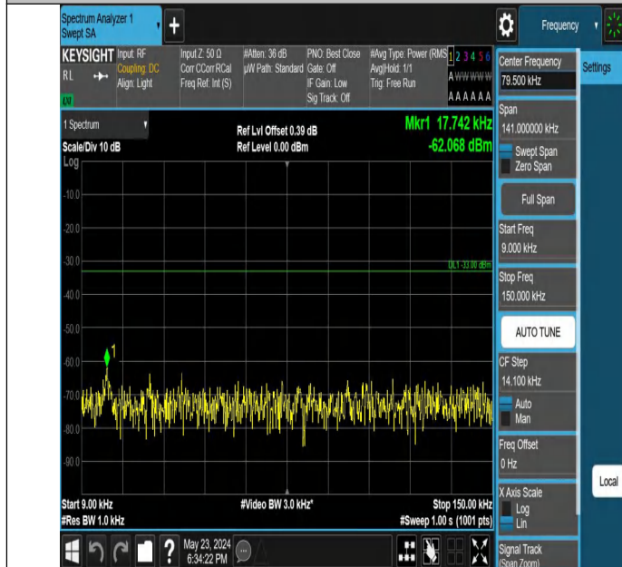
Band5_3MHz_QPSK_20415_1RB#0_0.009~0.15_0.009~0.15
