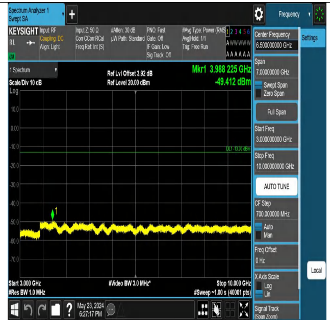
Band5_1.4MHz_QPSK_20407_1RB#5_3000~10000_3000~10000
