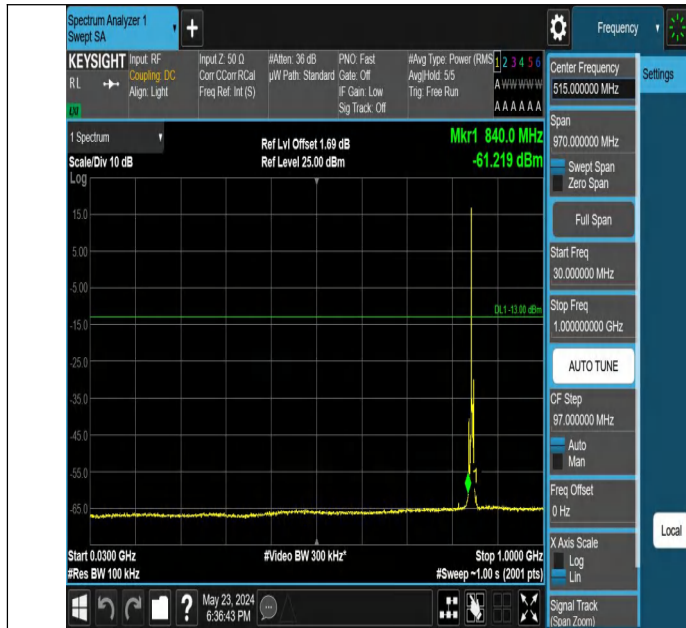
Band5_3MHz_QPSK_20635_1RB#0_30~1000_30~1000
