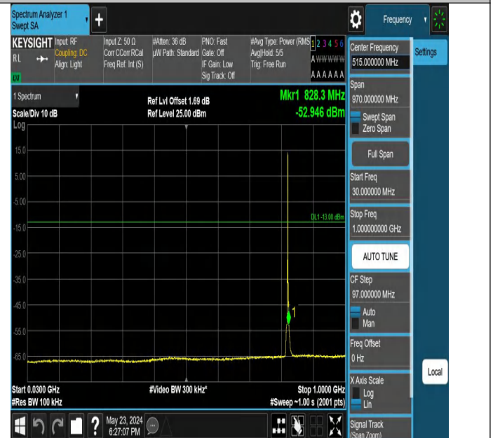
Band5_1.4MHz_QPSK_20407_1RB#5_30~1000_30~1000
