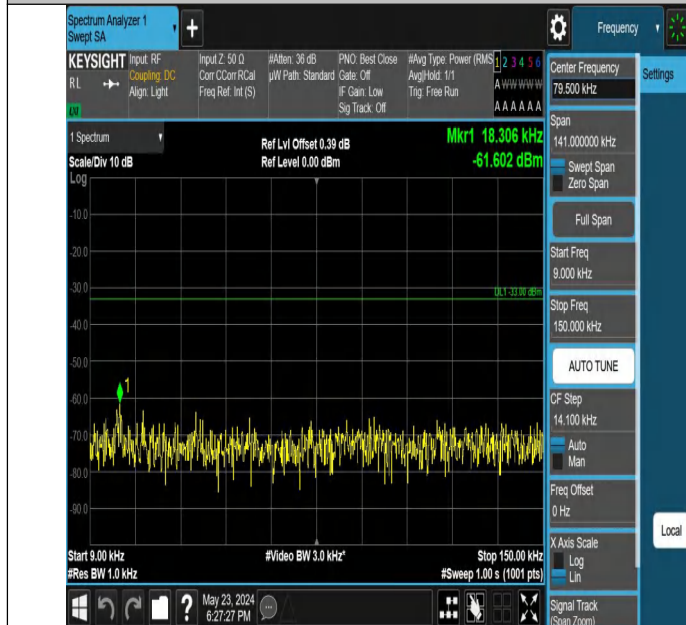
Band5_1.4MHz_QPSK_20525_1RB#0_0.009~0.15_0.009~0.15
