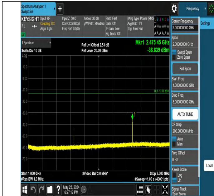
Band5_1.4MHz_QPSK_20407_1RB#5_1000~3000_1000~3000
