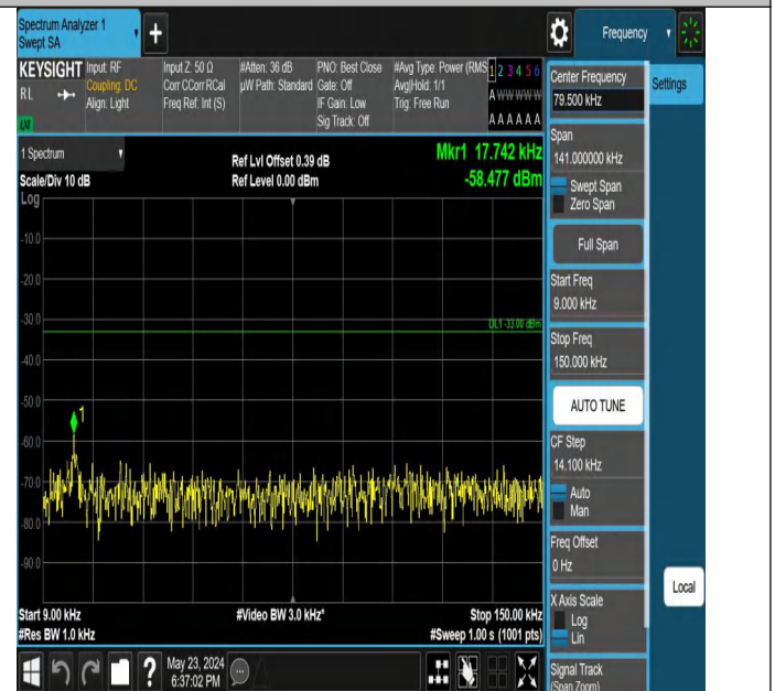
Band5_3MHz_QPSK_20635_1RB#14_0.009~0.15_0.009~0.15
