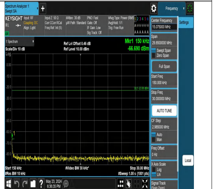
Band5_3MHz_QPSK_20635_1RB#0_0.15~30_0.15~30
