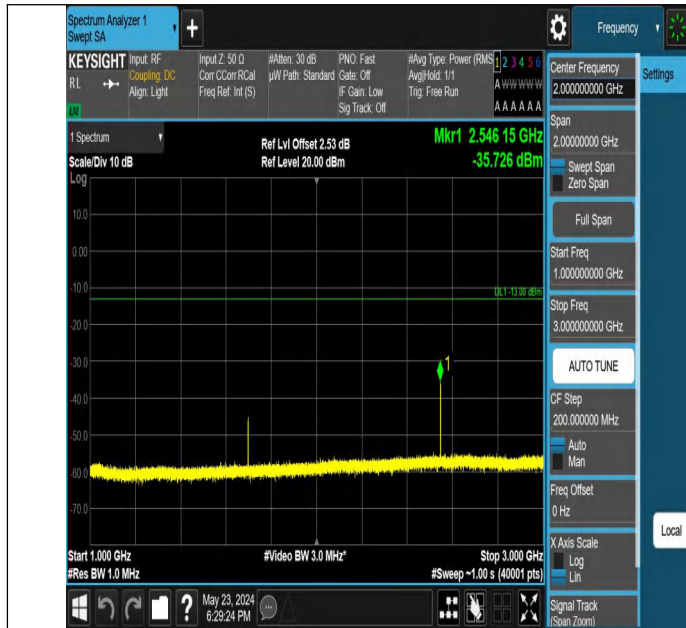
Band5_1.4MHz_QPSK_20643_1RB#5_1000~3000_1000~3000
