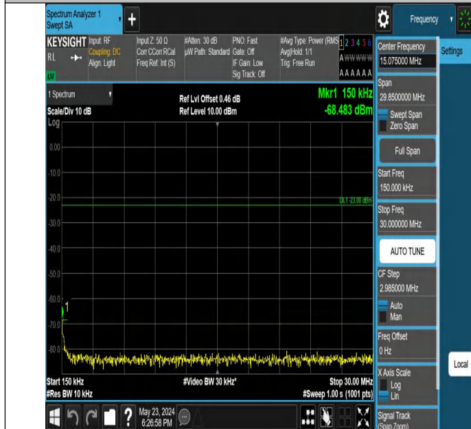
Band5_1.4MHz_QPSK_20407_1RB#5_0.15~30_0.15~30
