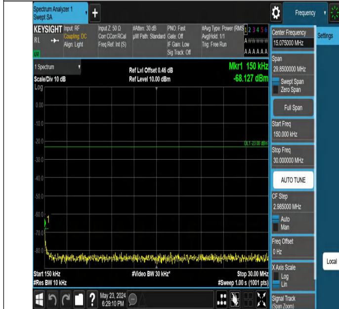
Band5_1.4MHz_QPSK_20643_1RB#5_0.15~30_0.15~30
