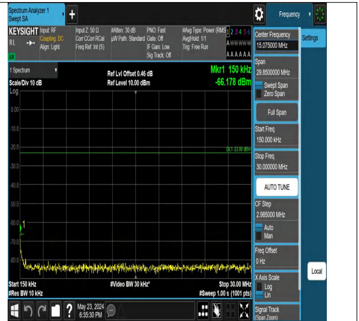
Band5_3MHz_QPSK_20525_1RB#0_0.15~30_0.15~30
