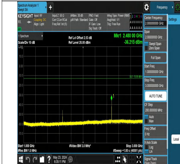
Band5_3MHz_QPSK_20415_1RB#14_1000~3000_1000~3000
