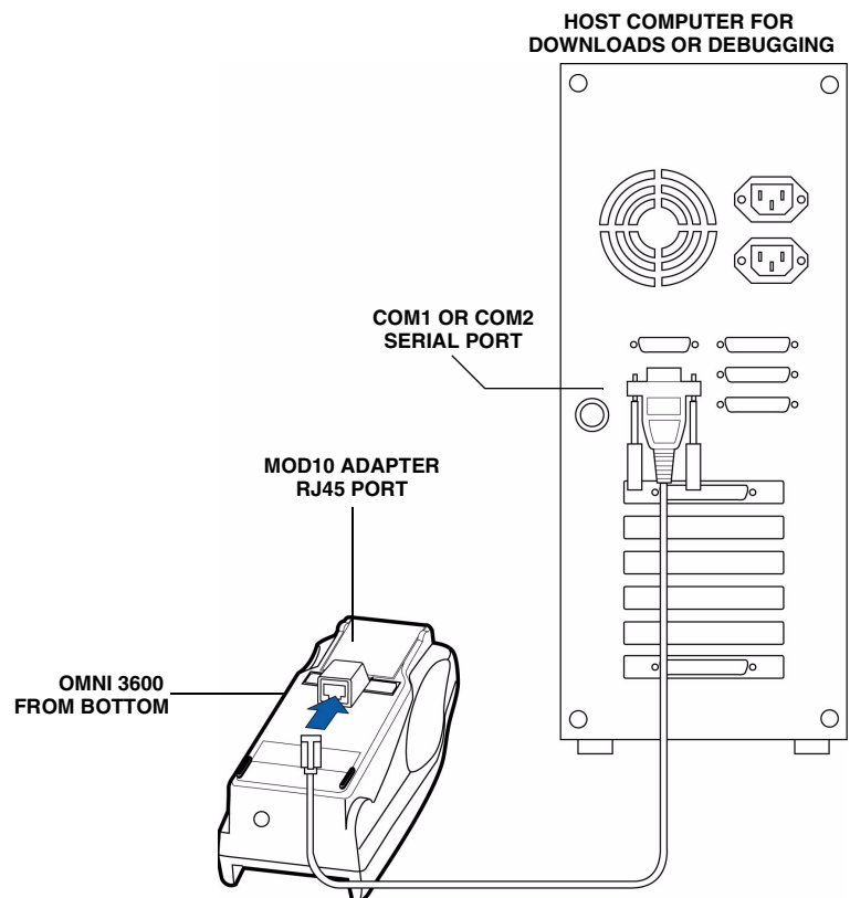
Figure 33 Serial Cable Connection using the MOD10 Adapter
