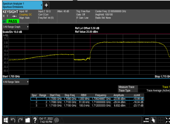
Band4 Channel1312
