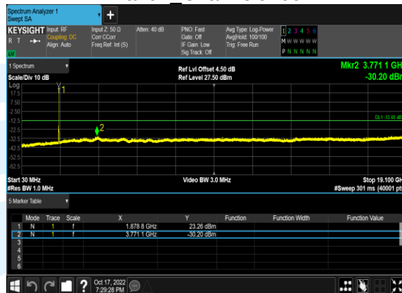
Band2 Channel9400
