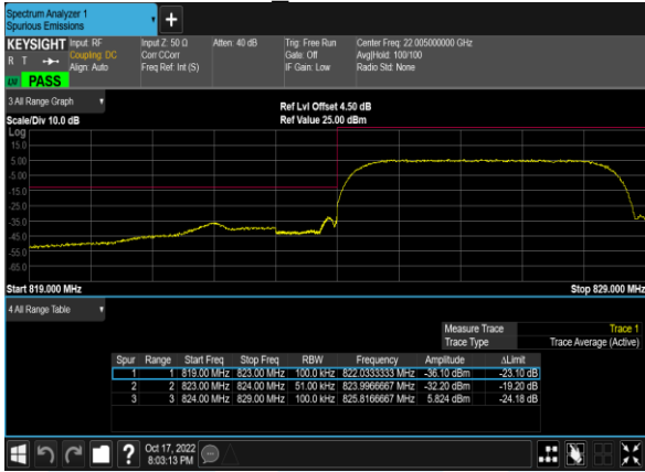
Band5 Channel4132
