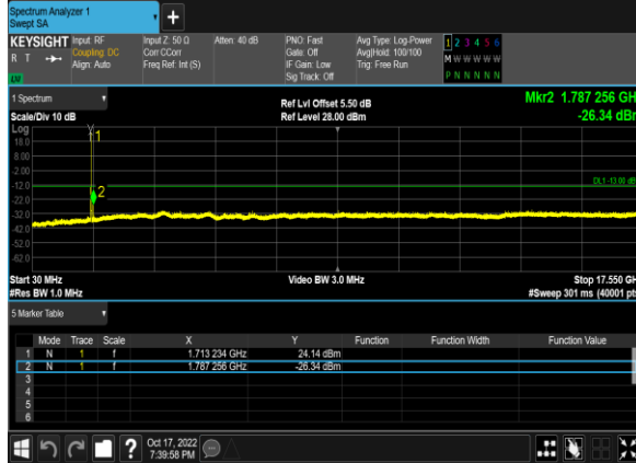
Band4_Channel1513
