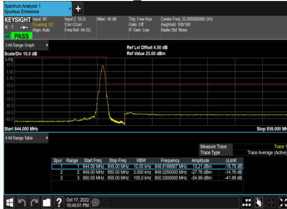
GSM850 Channel251
