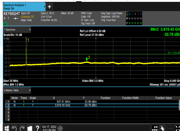
Band5 Channel4182
