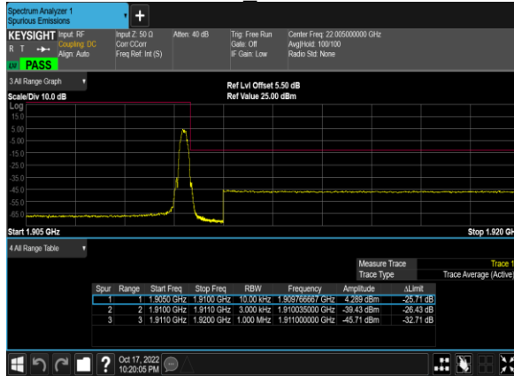
PCS1900 Channel810
