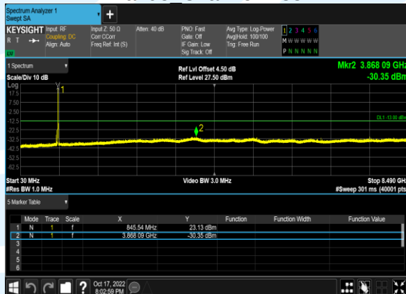
Band5 Channel4233
