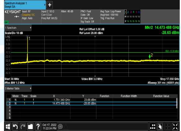
Band4_Channel1412
