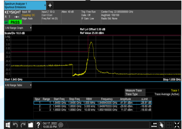
PCS1900 Channel512
