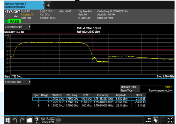
Band4 Channel1513
