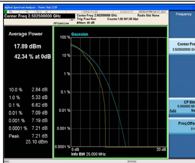
Band7_5MHz_QPSK_20775_25RB#0_6.09_13_PASS
