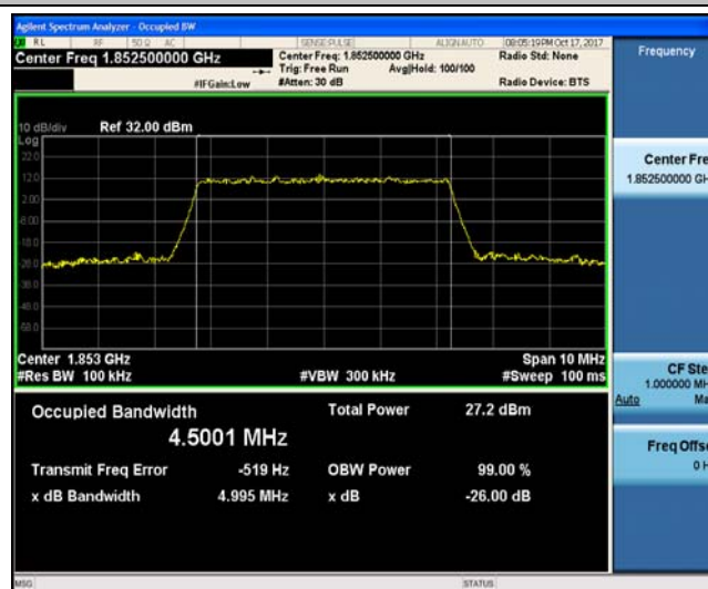
Band2_5MHz_QPSK_18900_25RB#0_4.5070_5.087_PASS
