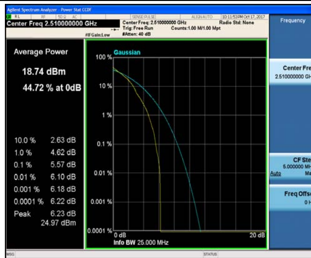
Band7_20MHz_16QAM_20850_1RB#0_6.31_13_PASS
