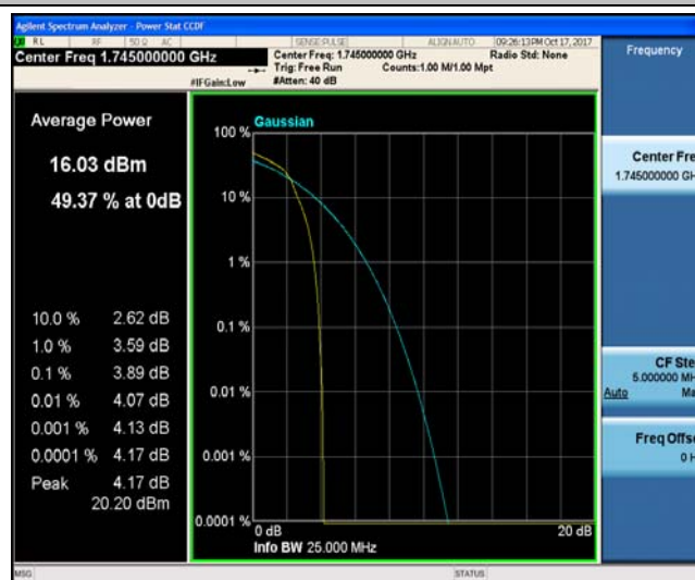
Band4_20MHz_QPSK_20300_100RB#0_4.93_13_PASS
