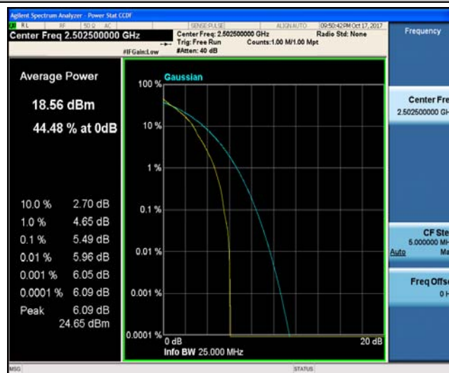
Band7_5MHz_16QAM_20775_1RB#0_6.62_13_PASS
