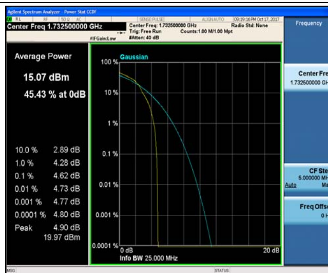
Band4_15MHz_QPSK_20175_75RB#0_4.77_13_PASS
