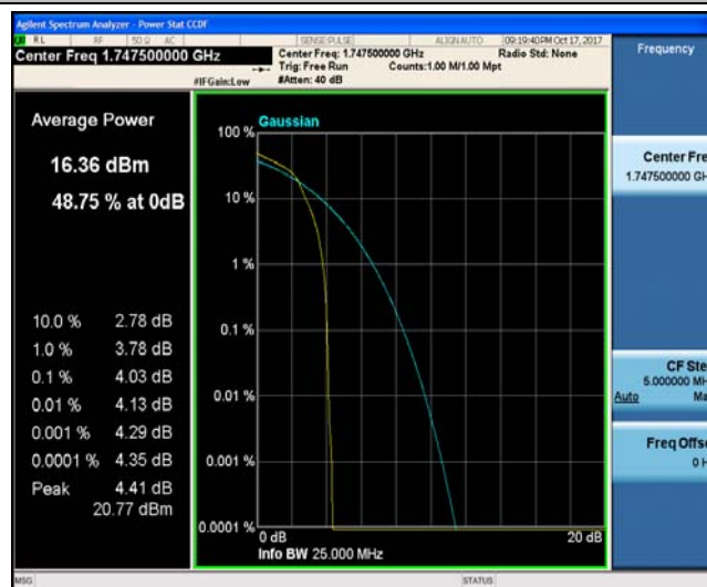
Band4_15MHz_QPSK_20325_75RB#0_5.00_13_PASS
