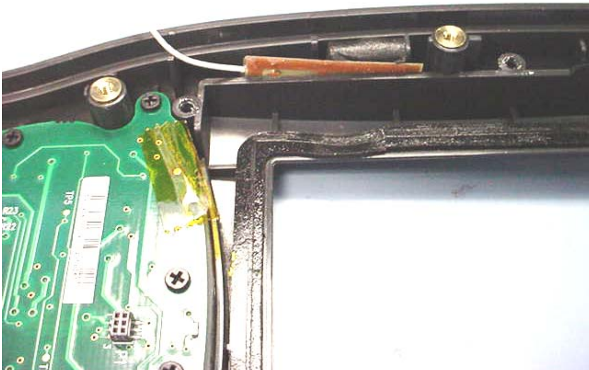
Bluetooth Antenna
