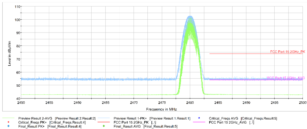
Fig.14. Frequency Band Edges: GFSK, Channel 78, Hopping Off, ch11, 2.45 GHz - 2.50GHz
