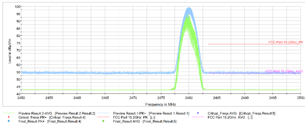
Fig.18. Frequency Band Edges: 8DPSK, Channel 78, 2.45 GHz - 2.50GHz
