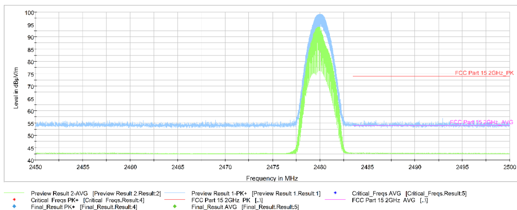
Fig.16. Frequency Band Edges: \pi/4 DQPSK, Channel 78, Hopping Off, 2.45 GHz - 2.50GHz
