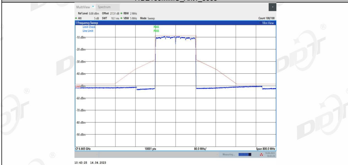
11BE160MIMO Ant2 6665
