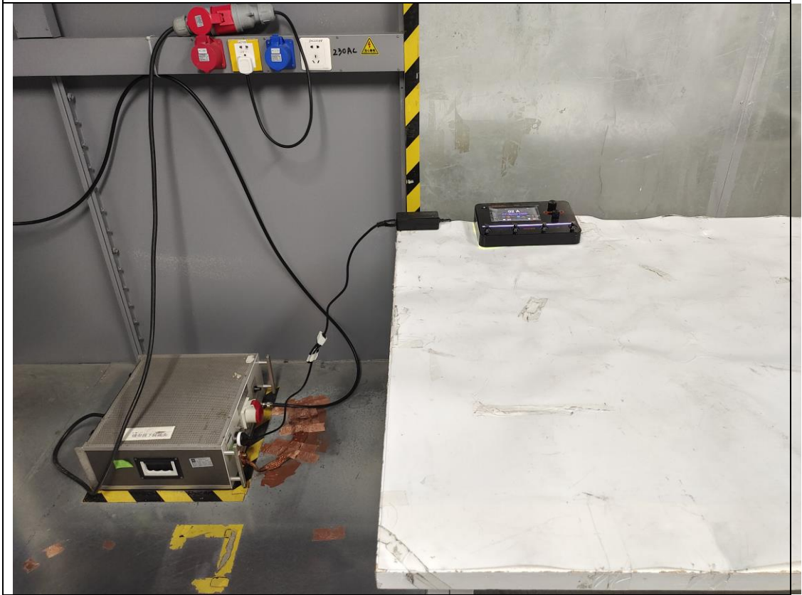
Conducted emission
