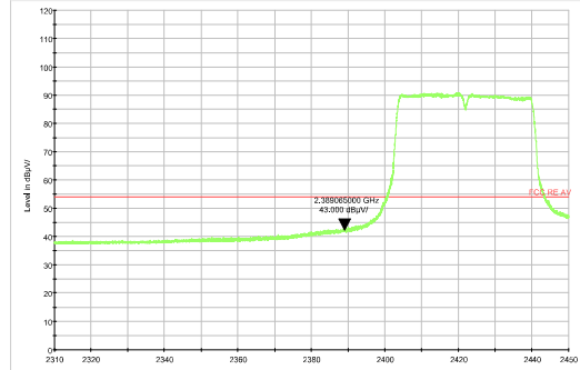
802.11n HT40 -Channel 3 Average
