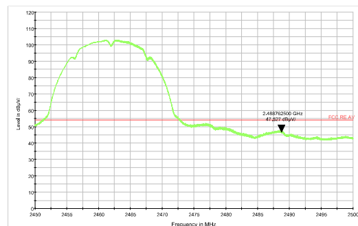
802.11b-Channel 11 Average
