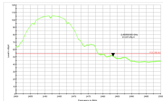
802.11b-Channel 11 Average
