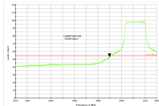
802.11g-Channel 1 Average
