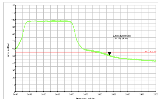
802.11g-Channel 11 Average
