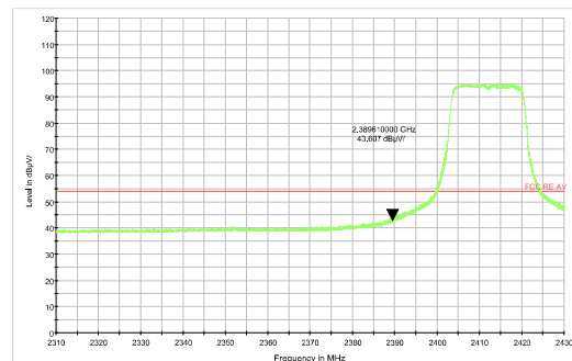
802.11g-Channel 1 Average
