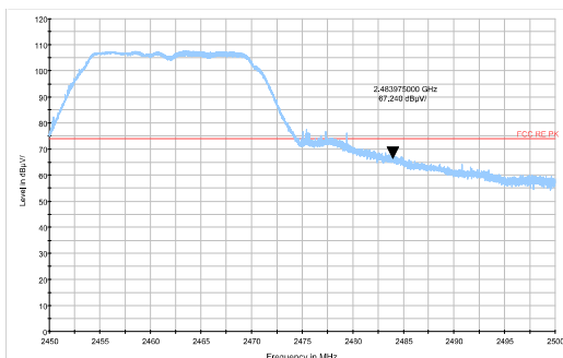
802.11g-Channel 11 Peak
