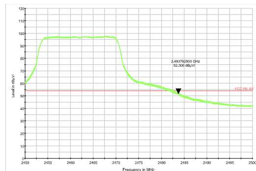
802.11g-Channel 11 Average
