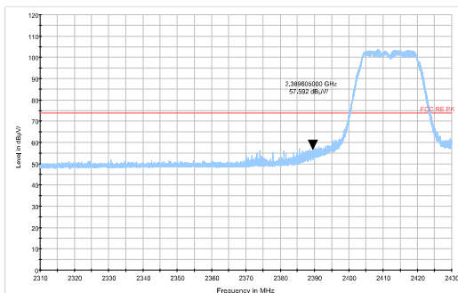
802.11g-Channel 1 Peak
