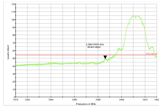
802.11b-Channel 1 Average
