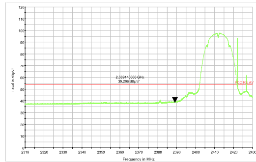
802.11b-Channel 1 Average
