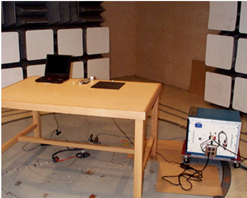
Conducted Emissions
