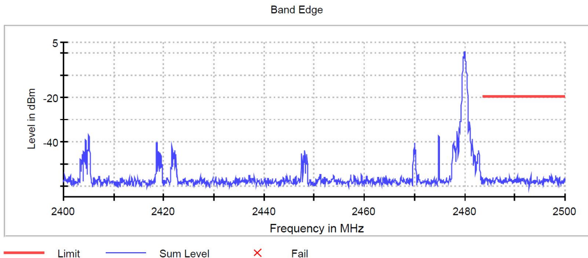
Graph 8: Upper Band Edge Plot
