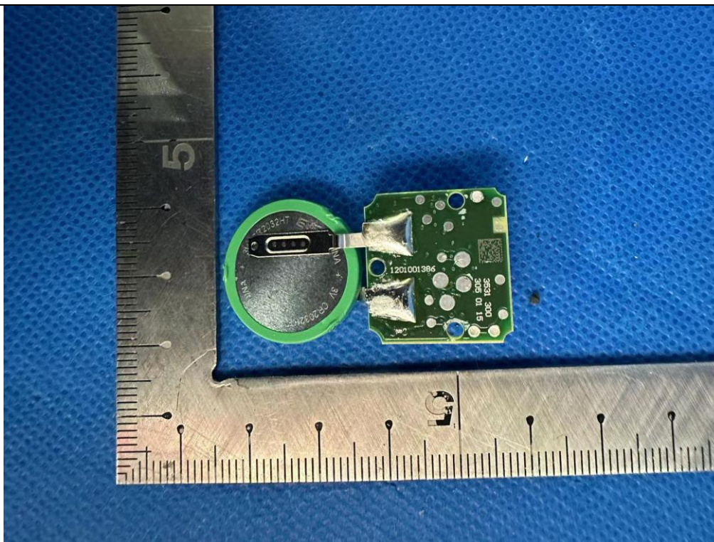
EUT Photo(6)-Antenna
