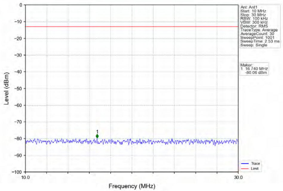
Band2_5MHz_QPSK_LCH_1852.5MHz_RB_1_0_NTNV
