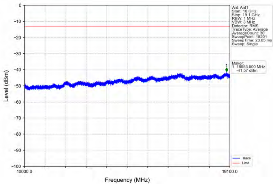
Band2_5MHz_QPSK_HCH_1907.5MHz_RB_1_24_NTNV
