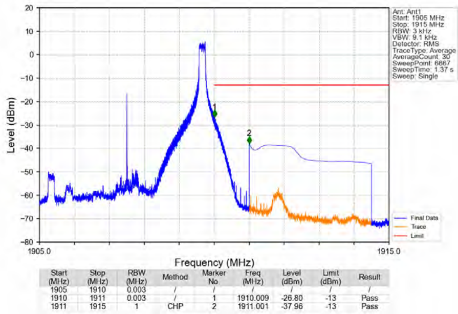
Band2_5MHz_QPSK_HCH_1907.5MHz_RB_1_24_NTNV
