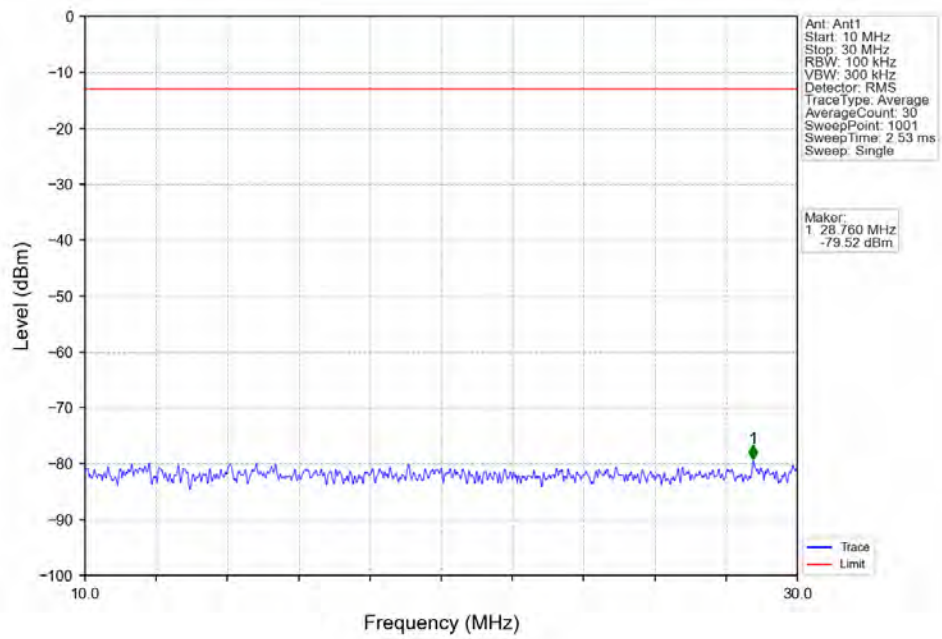
Band2_5MHz_16QAM_LCH_1852.5MHz_RB_1_0_NTNV
