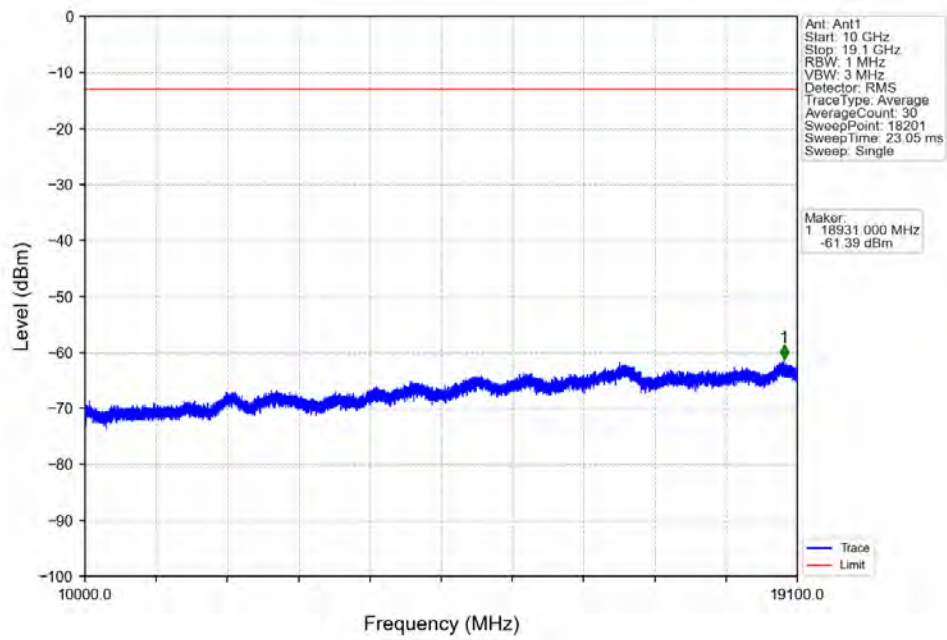
Band2_5MHz_16QAM_LCH_1852.5MHz_RB_1_0_NTNV
