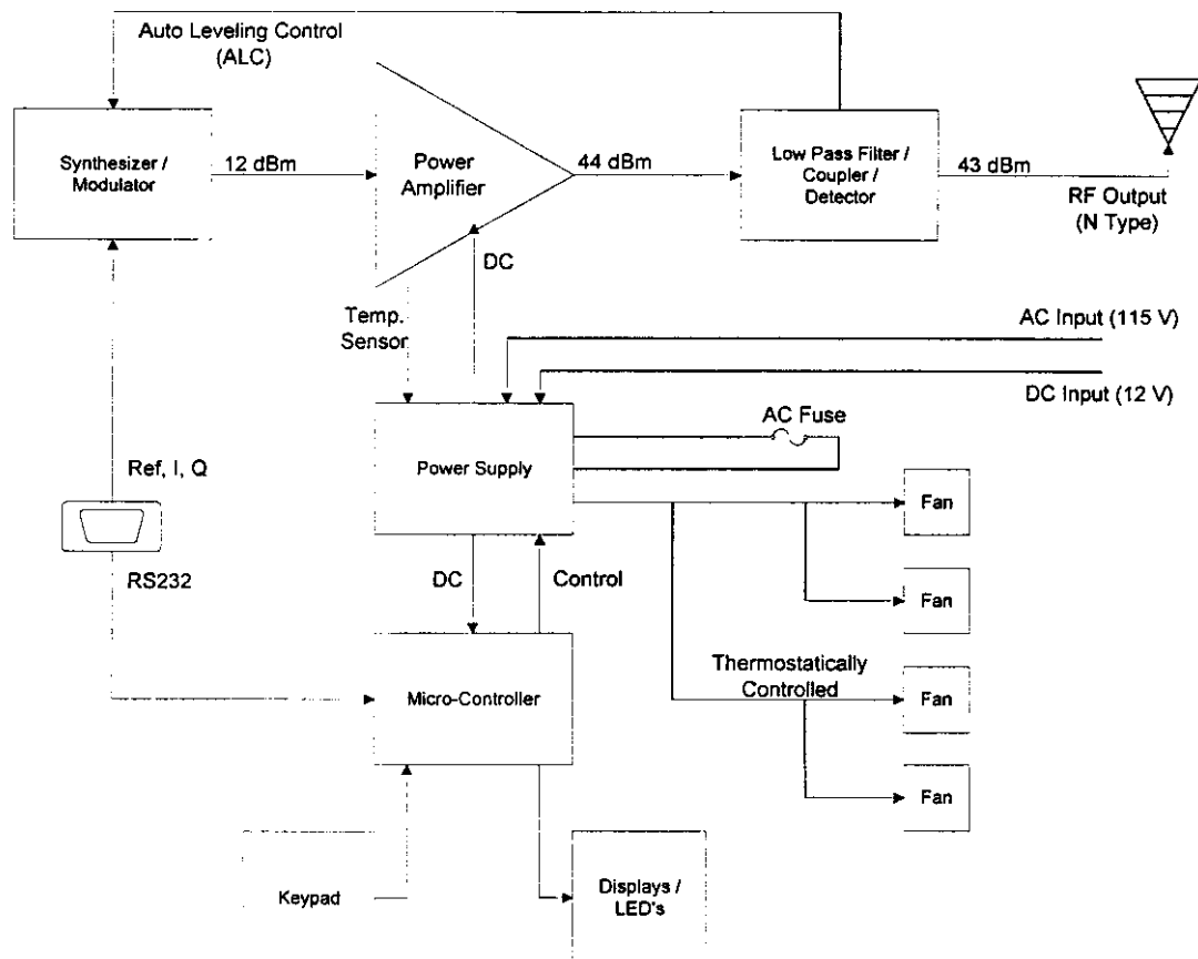
Figure 6.2.1 GMT20 Block Diagram
