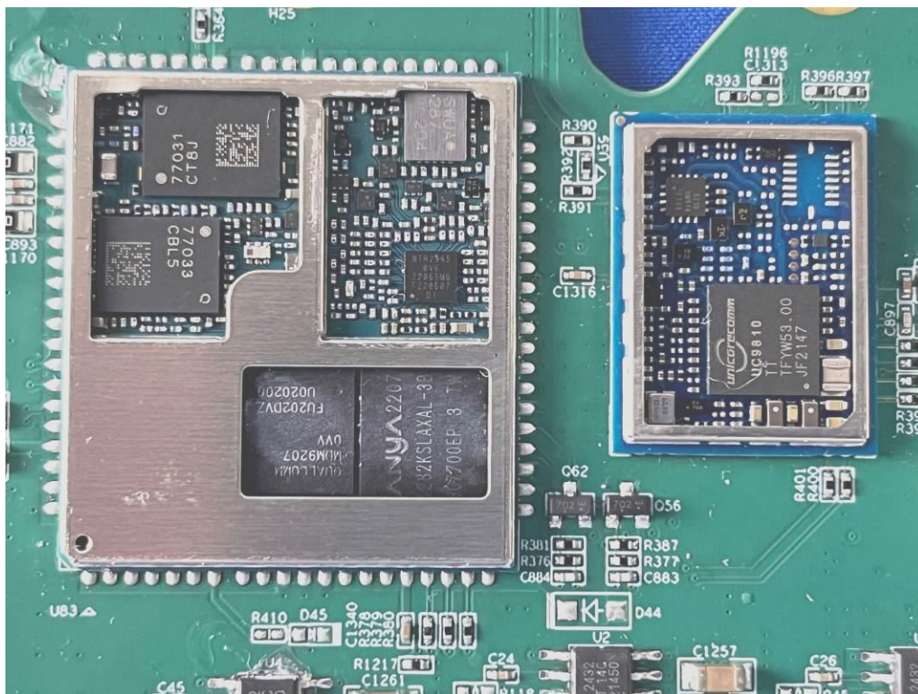
Internal view(PA-3 SE)
