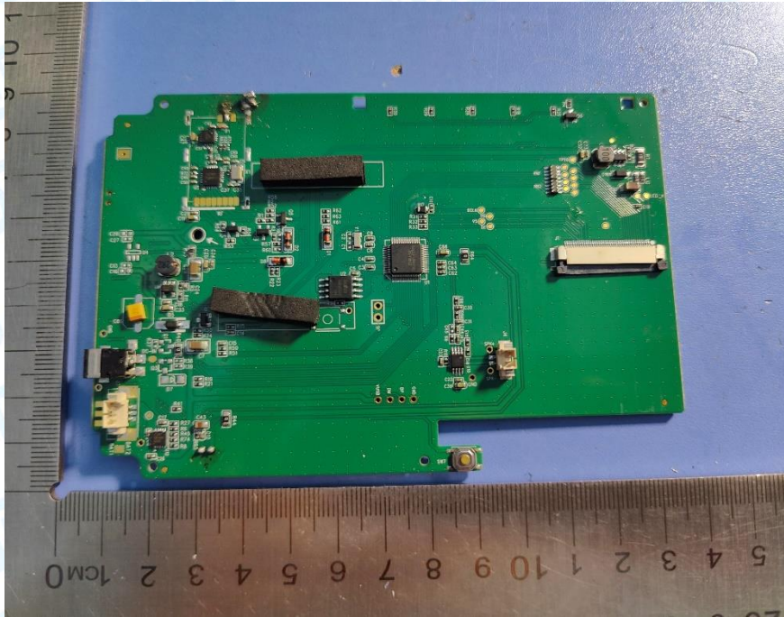
Photo 14 Appearance of PCB
