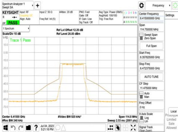
802.11be_20MHz_Chain0_6415MHz_106+26_MRUG
