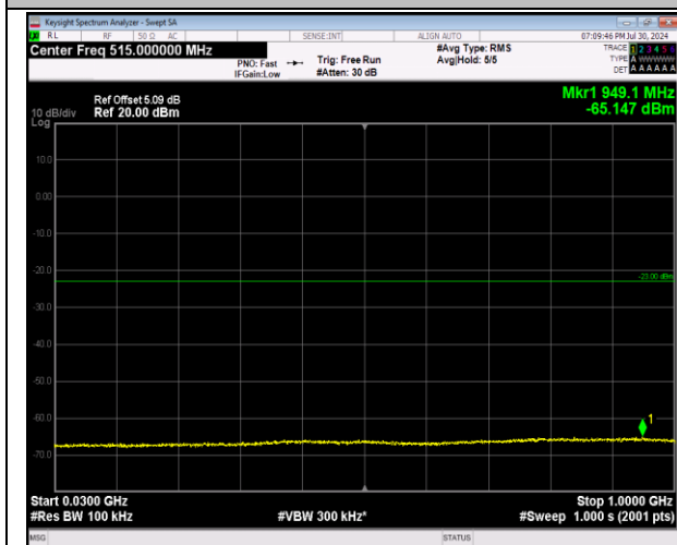
2-2-5MHz-20MHz-64QAM-64QAM-18808-18925-1RB#24-4-0RB#0-30-1000MHz-PASS
