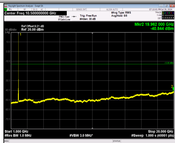
2-2-5MHz-20MHz-64QAM-64QAM-18808-18925-1RB#24-0-0RB#0-1000-20000MHz-PASS
