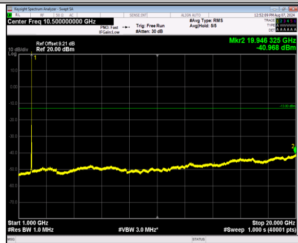
2-2-5MHz-20MHz-QPSK-QPSK-18983-19100-1RB#24-0 RB#0-1000~20000MHz-PASS
