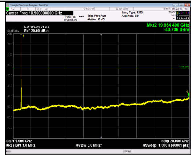
2-2-5MHz-20MHz-16QAM-16QAM-18808-18925-1RB#0- 0RB#0-1000~20000MHz-PASS
