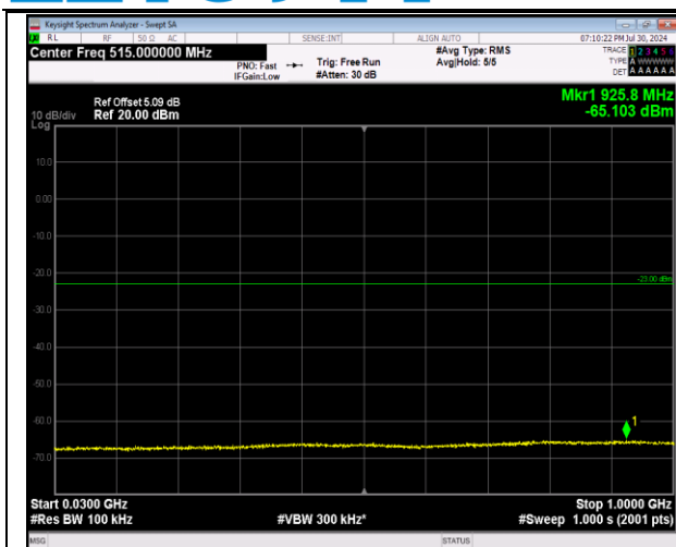
2-2-5MHz-20MHz-64QAM-64QAM-18808-18925-1RB#0-1RB#99-30-1000MHz-PASS
