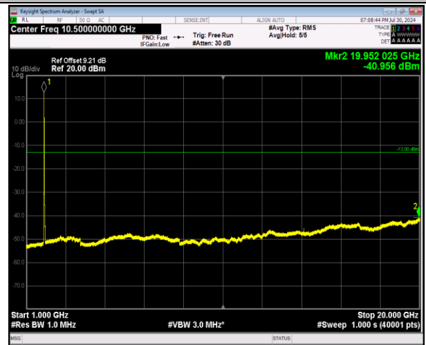
2-2-5MHz-20MHz-64QAM-64QAM-18633-18750-25RB#0-100RB#0-1000-20000MHz-PASS
