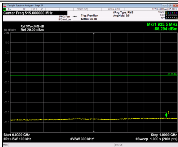
2-2-5MHz-20MHz-16QAM-16QAM-18983-19100-1RB#0- 1RB#99-30~1000MHz-PASS
