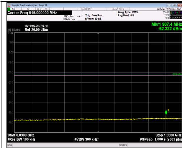
2-2-5MHz-20MHz-16QAM-16QAM-18633-18750-1RB#2 4-0RB#0-30~1000MHz-PASS
