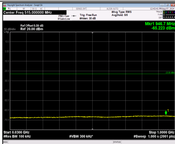
2-2-5MHz-20MHz-16QAM-16QAM-18633-18750-1RB#0- 1RB#99-30~1000MHz-PASS
