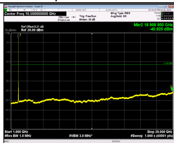
2-2-5MHz-20MHz-64QAM-64QAM-18808-18925-1RB#0-1RB#99-1000-20000MHz-PASS
