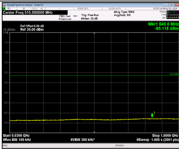
2-2-5MHz-20MHz-64QAM-64QAM-18633-18750-1RB#24-4-0RB#0-30-1000MHz-PASS
