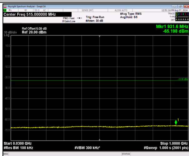
2-2-5MHz-20MHz-16QAM-16QAM-18983-19100-1RB#0- 0RB#0-30~1000MHz-PASS
