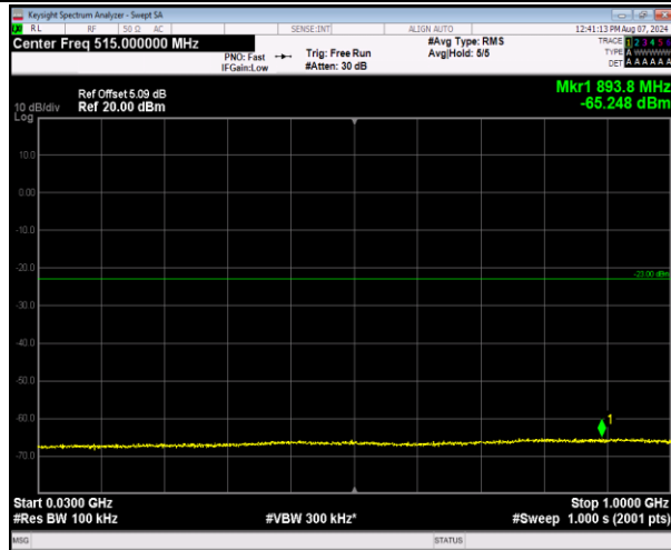
2-2-5MHz-20MHz-16QAM-16QAM-18633-18750-1RB#0- 0RB#0-30~1000MHz-PASS
