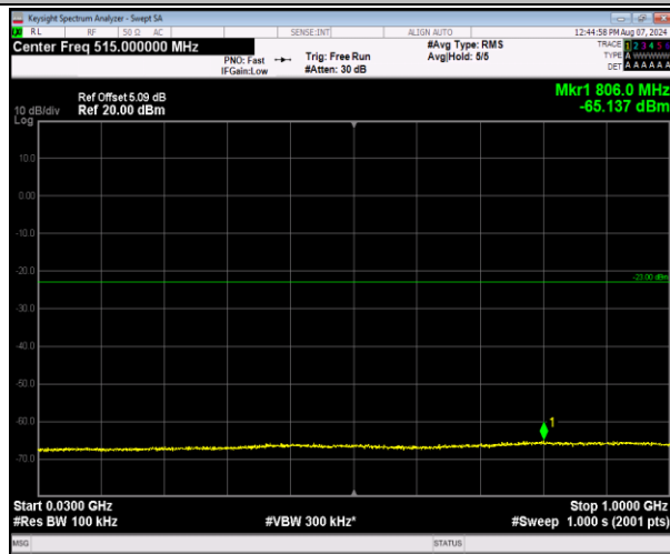
2-2-5MHz-20MHz-16QAM-16QAM-18633-18750-25RB# 0-100RB#0-30~1000MHz-PASS
