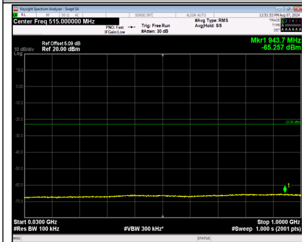
2-2-5MHz-20MHz-QPSK-QPSK-18983-19100-1RB#24-0 RB#0-30~1000MHz-PASS
