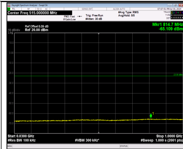
2-2-5MHz-20MHz-64QAM-64QAM-18633-18750-1RB#0-1RB#99-30-1000MHz-PASS
