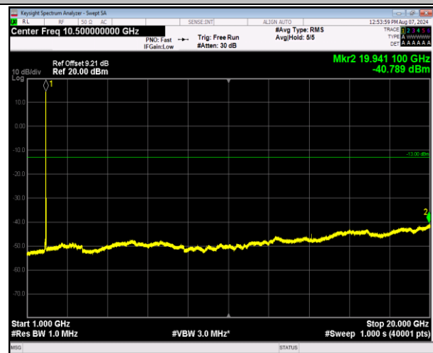
2-2-5MHz-20MHz-16QAM-16QAM-18983-19100-1RB#0- 1RB#99-1000~20000MHz-PASS
