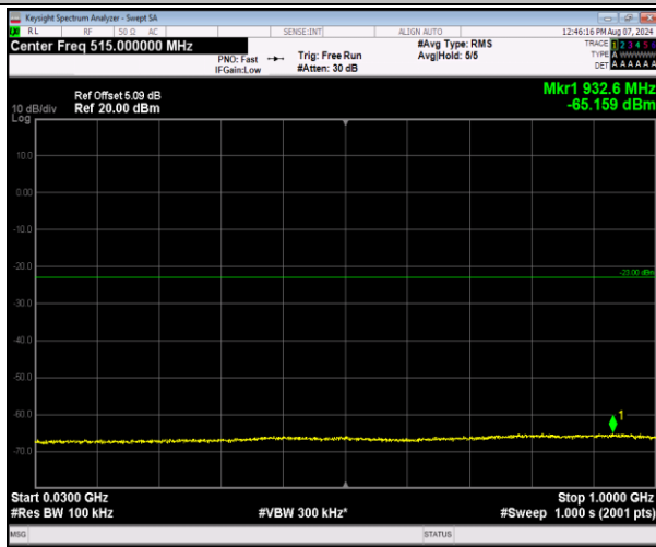
2-2-5MHz-20MHz-16QAM-16QAM-18808-18925-1RB#0- 0RB#0-30~1000MHz-PASS
