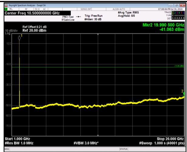
2-2-5MHz-20MHz-64QAM-64QAM-18633-18750-1RB#0-1RB#99-1000-20000MHz-PASS
