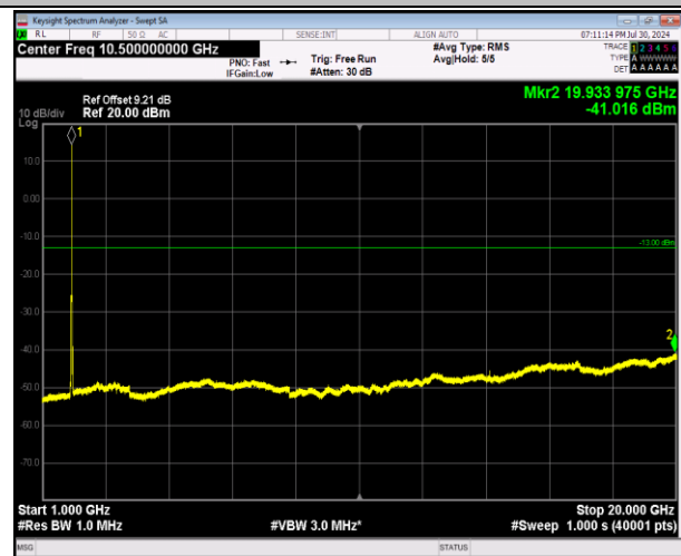
2-2-5MHz-20MHz-64QAM-64QAM-18808-18925-25RB#0-100RB#0-1000-20000MHz-PASS
