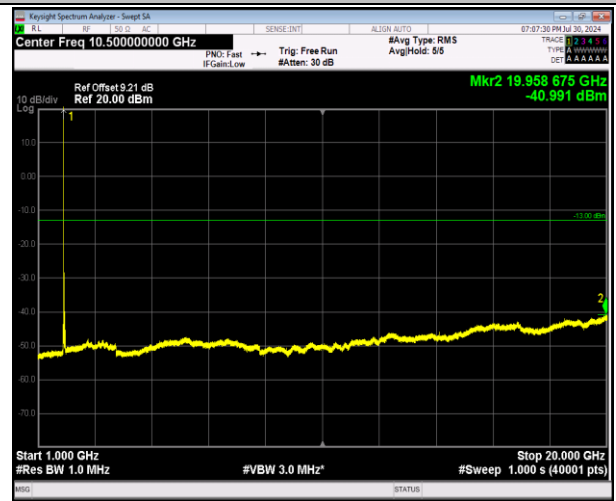
2-2-5MHz-20MHz-64QAM-64QAM-18633-18750-1RB#24-0RB#0-1000-20000MHz-PASS
