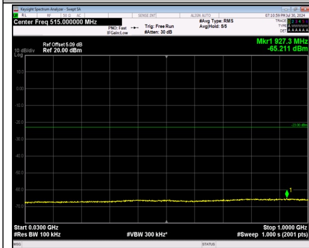
2-2-5MHz-20MHz-64QAM-64QAM-18808-18925-25RB#0-100RB#0-30-1000MHz-PASS
