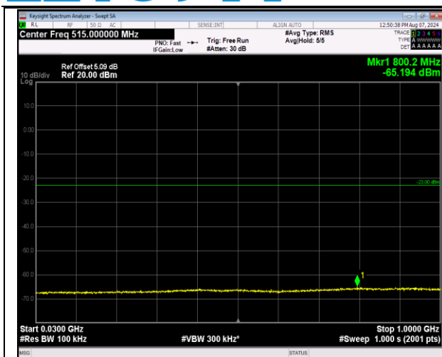
2-2-5MHz-20MHz-QPSK-QPSK-18983-19100-1RB#0-0R B#0-30~1000MHz-PASS
