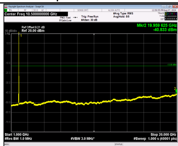
2-2-5MHz-20MHz-QPSK-QPSK-18983-19100-1RB#0-0R B#0-1000~20000MHz-PASS
