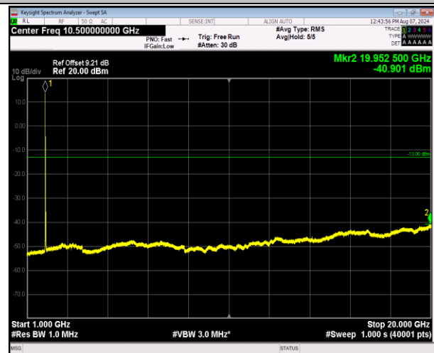
2-2-5MHz-20MHz-16QAM-16QAM-18633-18750-1RB#0- 1RB#99-1000~20000MHz-PASS
