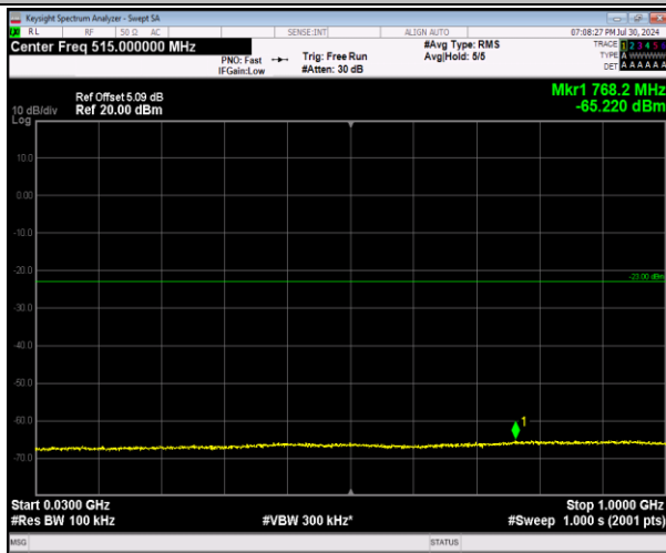
2-2-5MHz-20MHz-64QAM-64QAM-18633-18750-25RB#0-100RB#0-30-1000MHz-PASS
