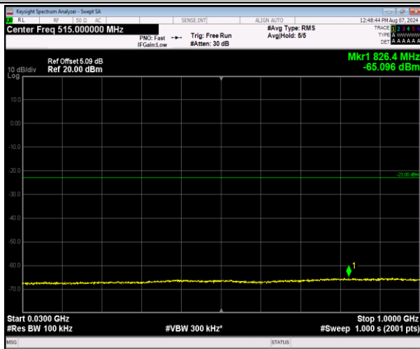
2-2-5MHz-20MHz-16QAM-16QAM-18808-18925-1RB#0- 1RB#99-30~1000MHz-PASS
