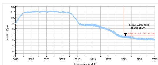
802.11a-Channel 140: Peak
