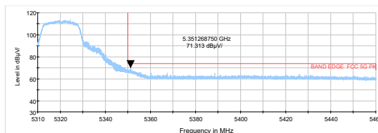
802.11a-Channel 64: Peak
