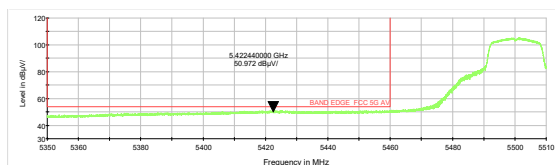
802.11a-Channel 100: Average
