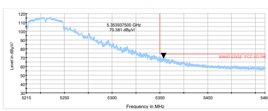
802.11n HT40-Channel 46: Average
