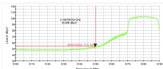
802.11ac VHT20-Channel 36: Average
