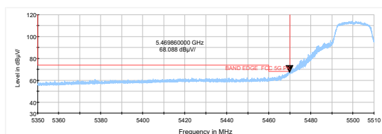
802.11a-Channel 100: Peak
