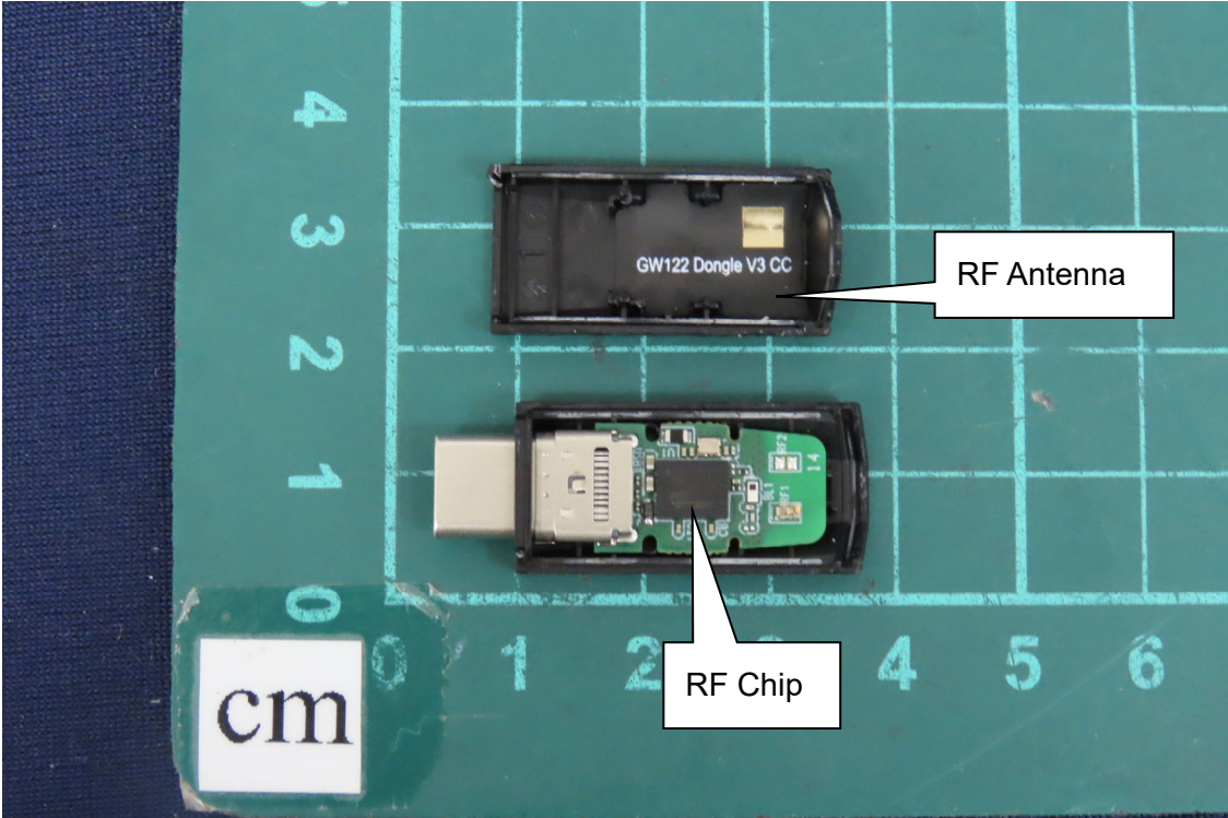
(1) EUT Photo
