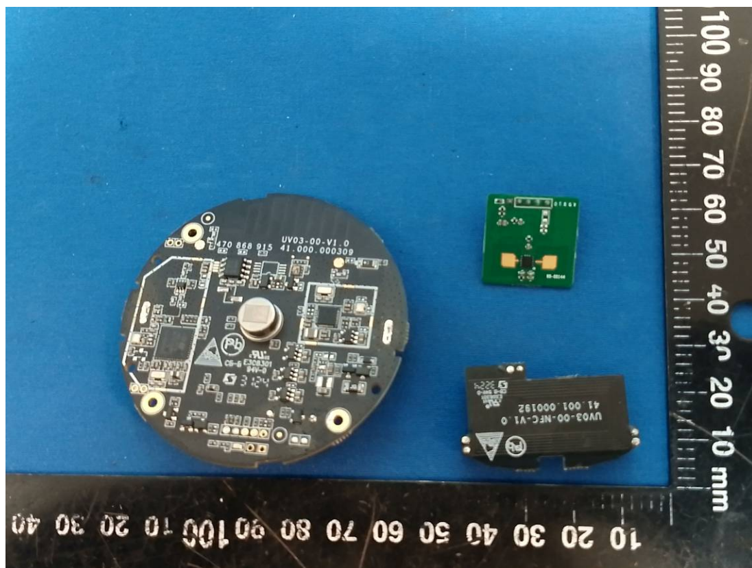
NFC Antenna(only receive)
