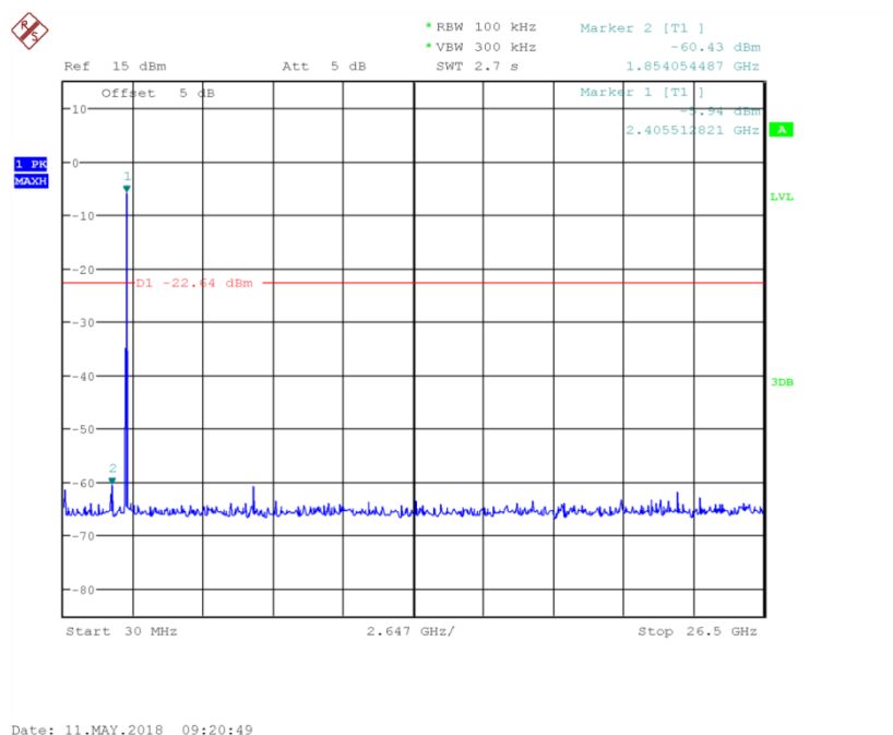
Fig.13 Conducted spurious emission: Ch0, 30MHz~26GHz
