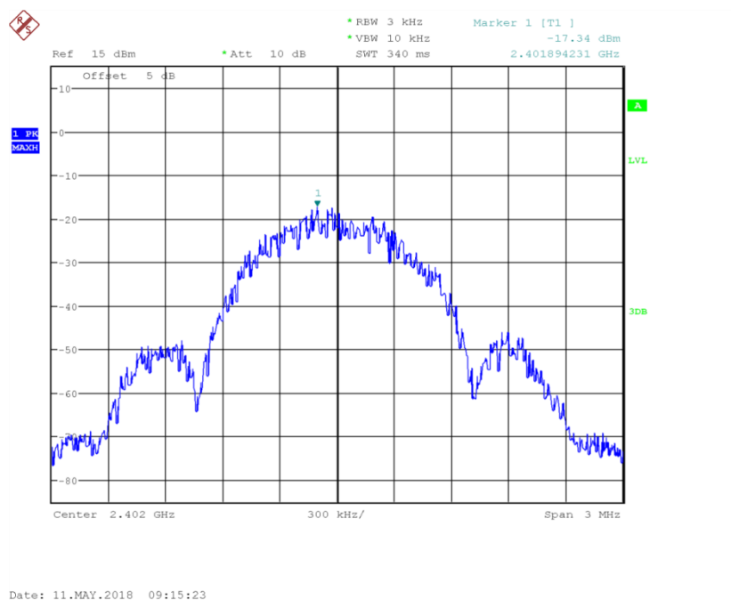
Fig.4 Power spectral density: CH0
