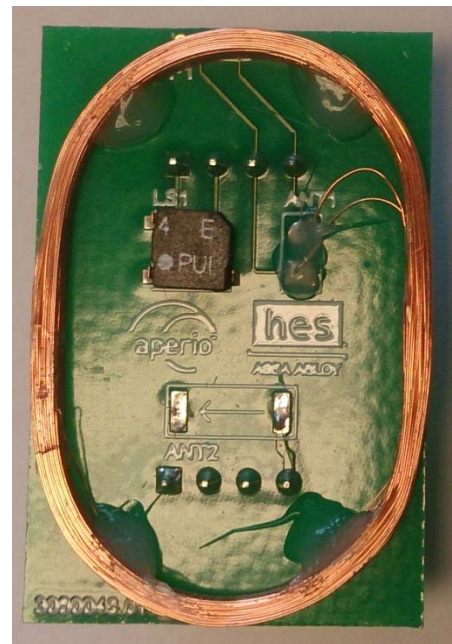
R100-PA2 antenna board – top view
