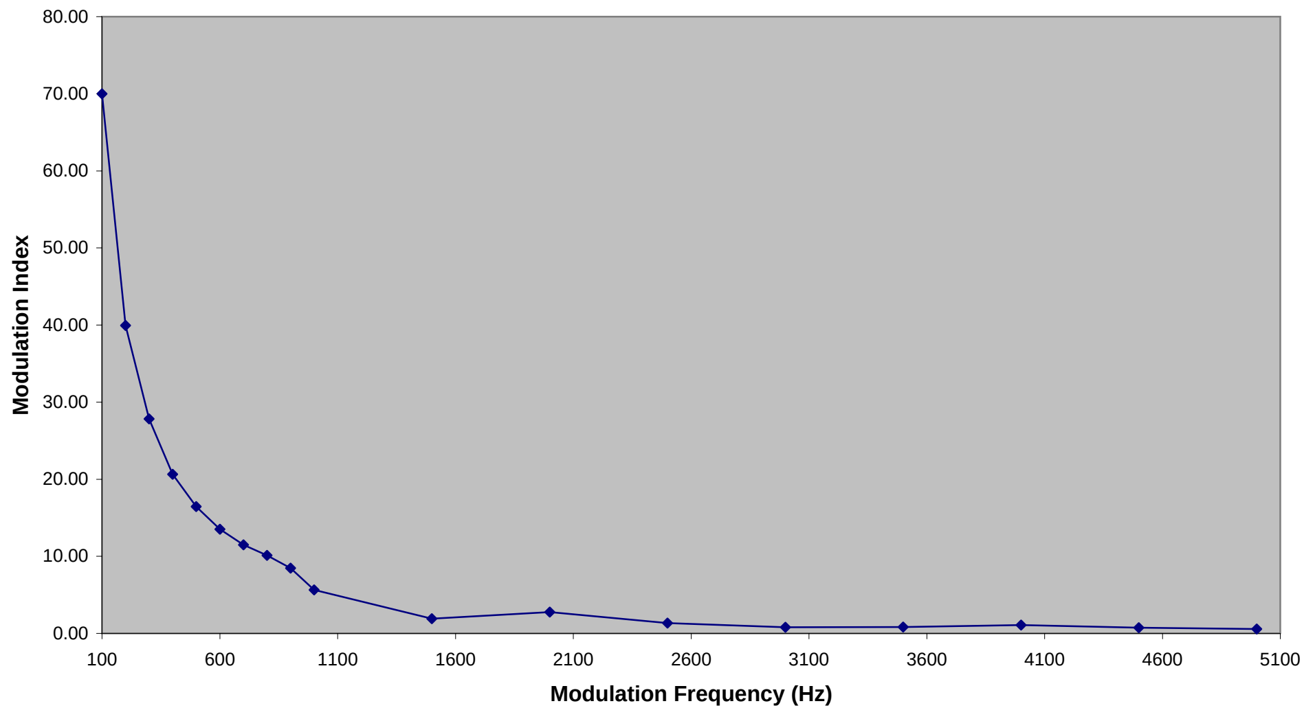
Modulation Frequency Response (171.905MHz)
