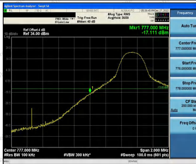
Band13-5MHz-QPSK-23205-1RB#24
