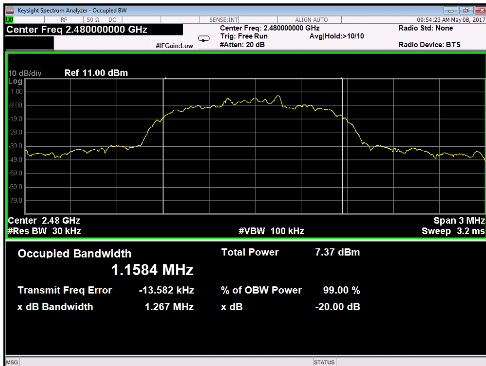
78 Channel @ 8-DPSK
