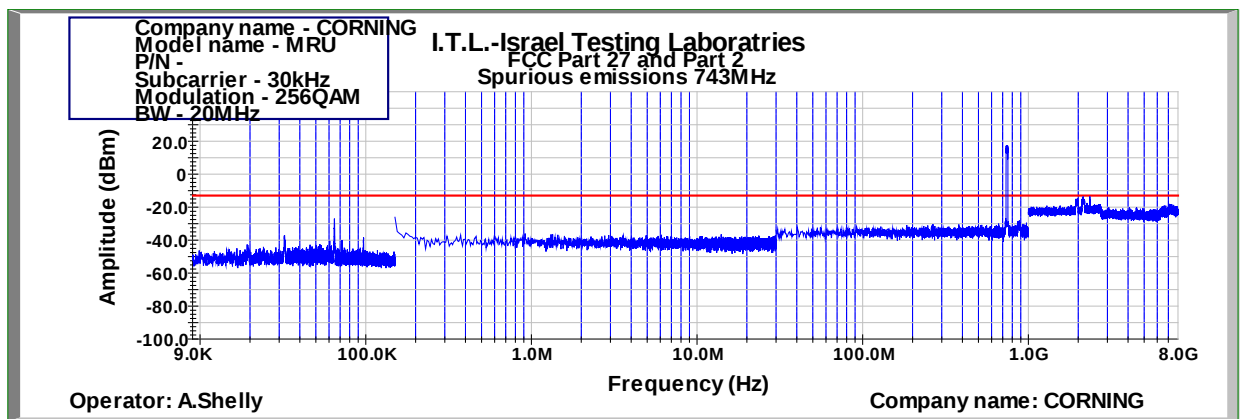
Figure 498: Spurious Emissions at Antenna Terminal 256QAM 20MHz B.W.; 743.0MHz, 30kHz
