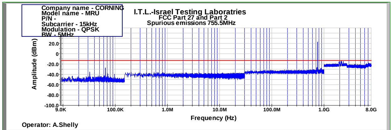
Figure 507: Spurious Emissions at Antenna Terminal QPSK 5MHz B.W.; 755.5MHz, 15kHz
