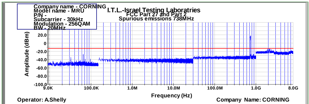
Figure 495: Spurious Emissions at Antenna Terminal 256QAM 20MHz B.W.; 738.0MHz, 30kHz
