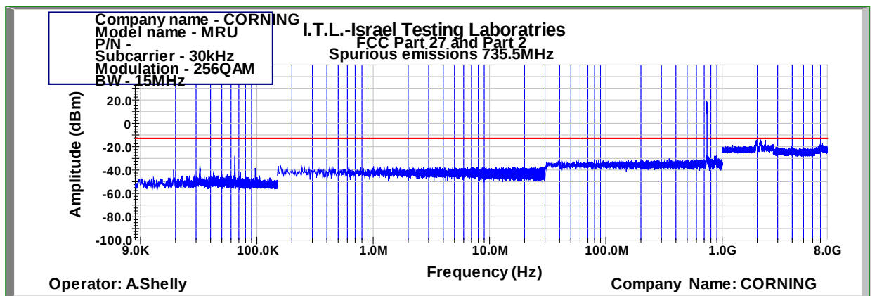
Figure 486: Spurious Emissions at Antenna Terminal 256QAM 15MHz B.W.; 735.5MHz, 30kHz
