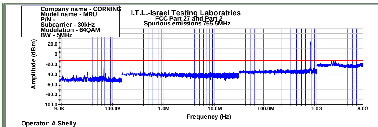
Figure 442: Spurious Emissions at Antenna Terminal 64QAM 5MHz B.W.; 755.5MHz, 30kHz
