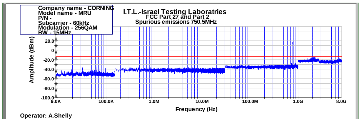
Figure 493: Spurious Emissions at Antenna Terminal 256QAM 15MHz B.W.; 750.5MHz, 60kHz
