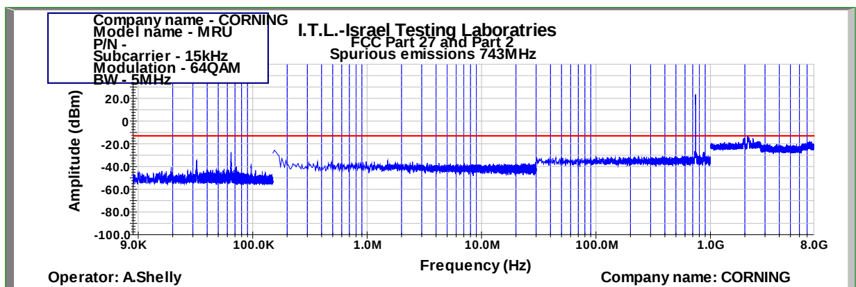
Figure 439: Spurious Emissions at Antenna Terminal 64QAM 5MHz B.W.; 743.0MHz, 15kHz
