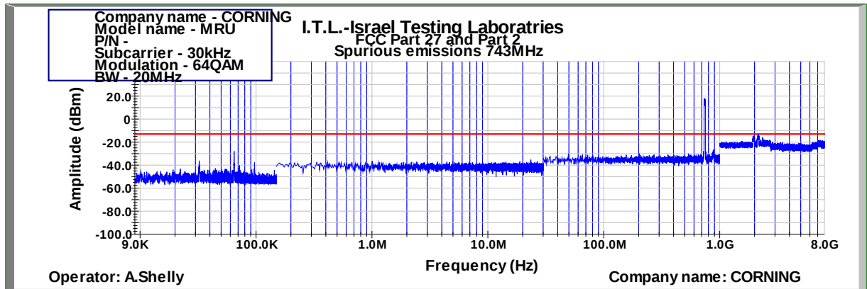
Figure 465: Spurious Emissions at Antenna Terminal 64QAM 20MHz B.W.; 743.0MHz, 30kHz
