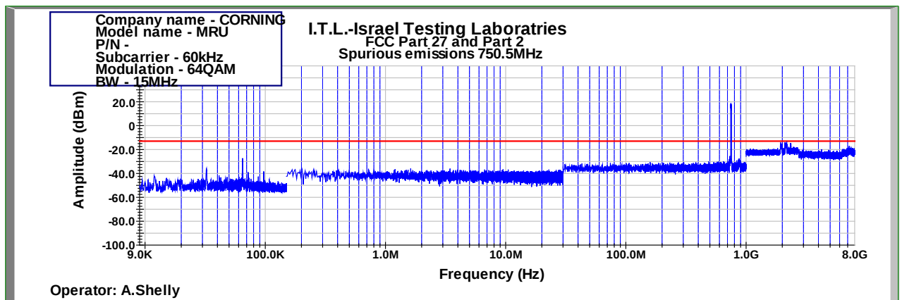
Figure 460: Spurious Emissions at Antenna Terminal 64QAM 15MHz B.W.; 750.5MHz, 60kHz
