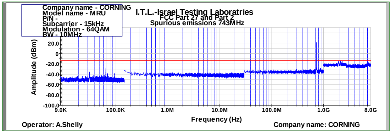
Figure 446: Spurious Emissions at Antenna Terminal 64QAM 10MHz B.W.; 743.0MHz, 15kHz
