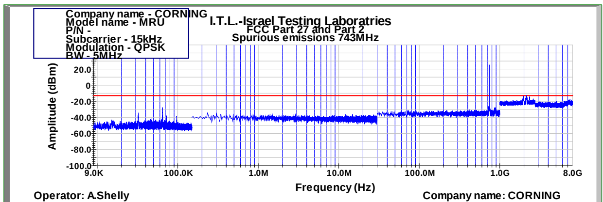
Figure 505: Spurious Emissions at Antenna Terminal QPSK 5MHz B.W.; 743.0MHz, 15kHz
