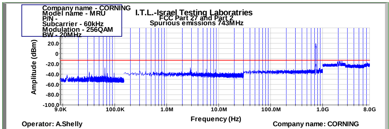
Figure 499: Spurious Emissions at Antenna Terminal 256QAM 20MHz B.W.; 743.0MHz, 60kHz
