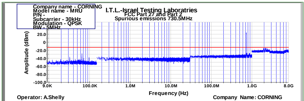
Figure 504: Spurious Emissions at Antenna Terminal QPSK 5MHz B.W.; 730.5MHz, 30kHz
