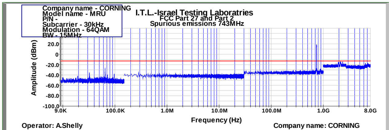
Figure 456: Spurious Emissions at Antenna Terminal 64QAM 15MHz B.W.; 743.0MHz, 30kHz
