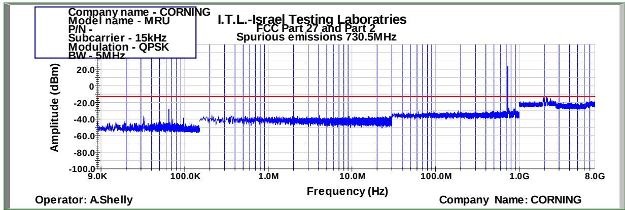
Figure 503: Spurious Emissions at Antenna Terminal QPSK 5MHz B.W.; 730.5MHz, 15kHz
