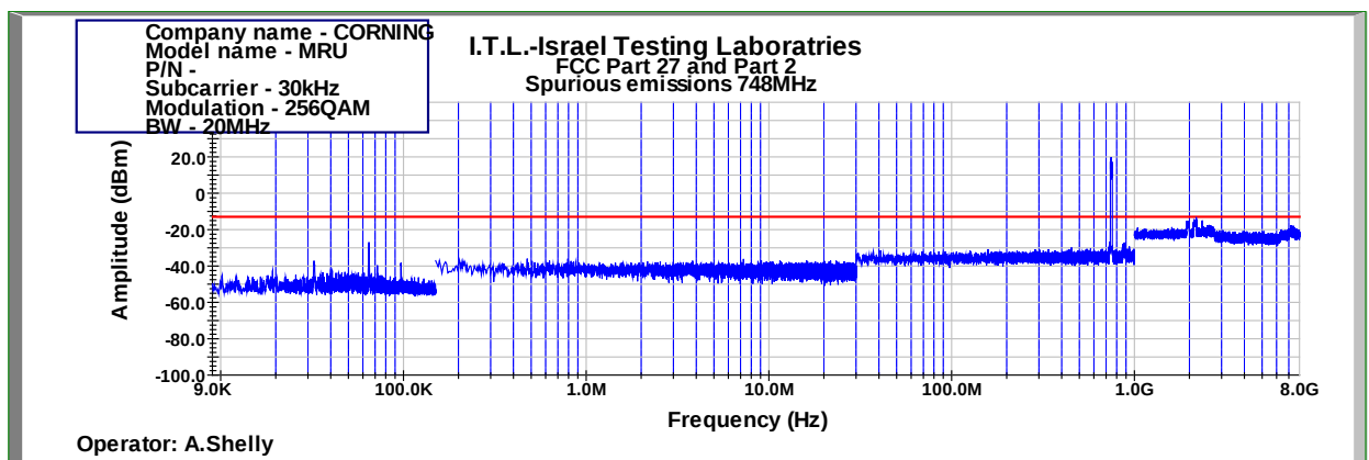
Figure 501: Spurious Emissions at Antenna Terminal 256QAM 20MHz B.W.; 748.0MHz, 30kHz
