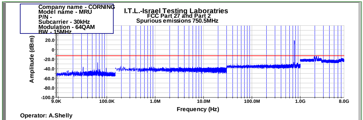
Figure 459: Spurious Emissions at Antenna Terminal 64QAM 15MHz B.W.; 750.5MHz, 30kHz
