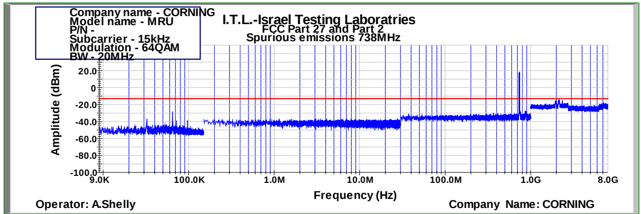
Figure 461: Spurious Emissions at Antenna Terminal 64QAM 20MHz B.W.; 738.0MHz, 15kHz
