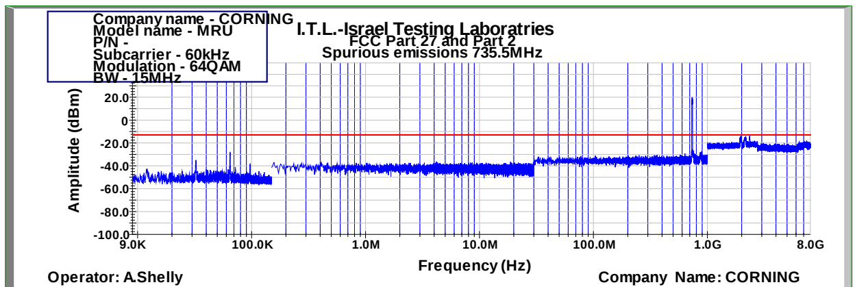
Figure 454: Spurious Emissions at Antenna Terminal 64QAM 15MHz B.W.; 735.5MHz, 60kHz
