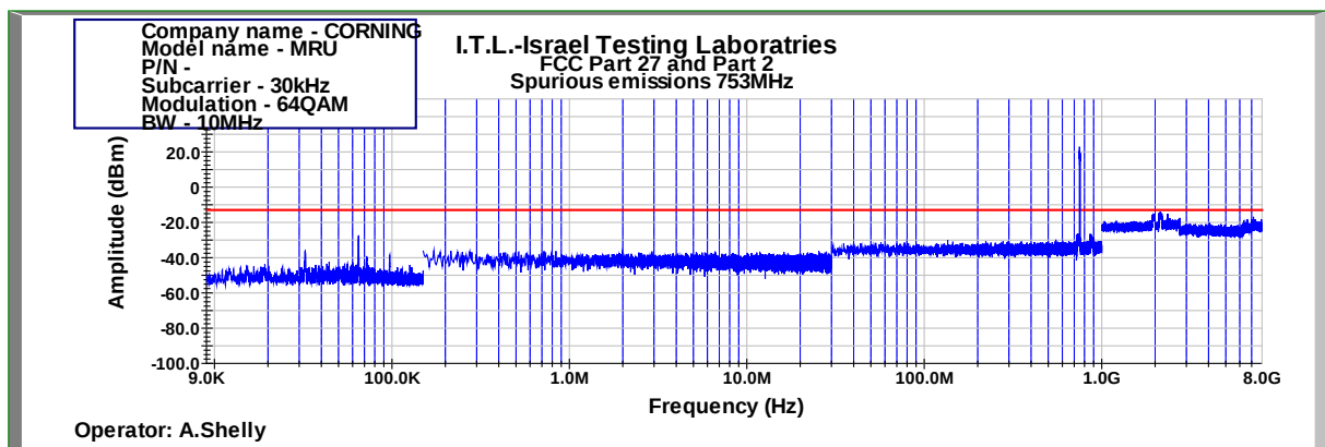
Figure 450: Spurious Emissions at Antenna Terminal 64QAM 10MHz B.W.; 753.0MHz, 30kHz
