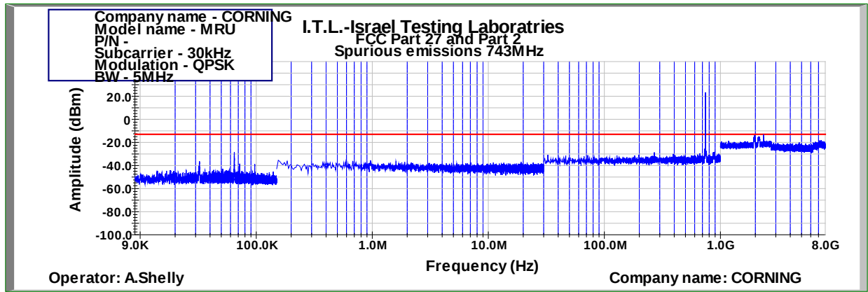
Figure 506: Spurious Emissions at Antenna Terminal QPSK 5MHz B.W.; 743.0MHz, 30kHz
