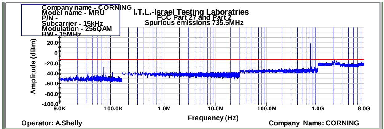
Figure 485: Spurious Emissions at Antenna Terminal 256QAM 15MHz B.W.; 735.5MHz, 15kHz
