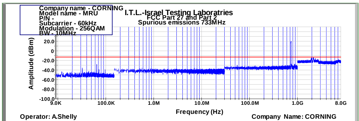
Figure 478: Spurious Emissions at Antenna Terminal 256QAM 10MHz B.W.; 733.0MHz, 60kHz
