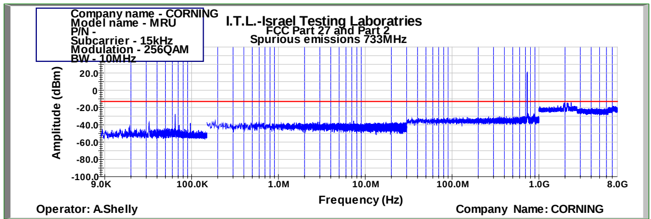
Figure 476: Spurious Emissions at Antenna Terminal 256QAM 10MHz B.W.; 733.0MHz, 15kHz
