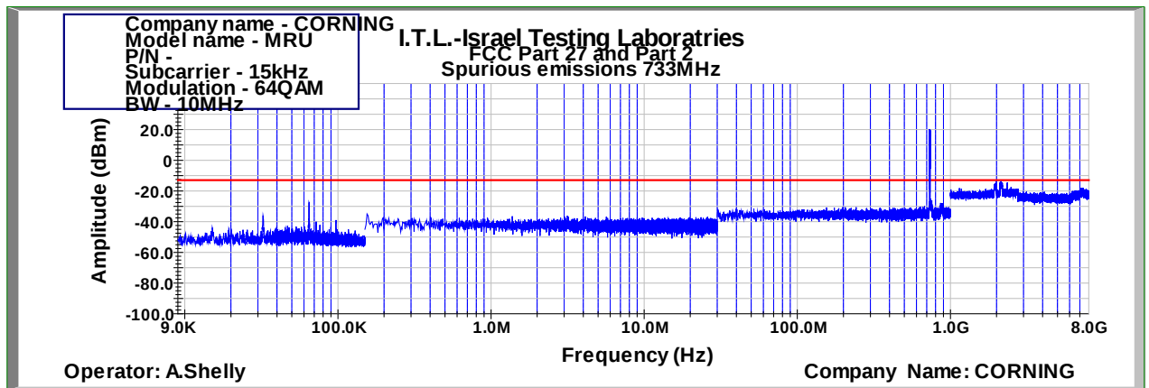
Figure 443: Spurious Emissions at Antenna Terminal 64QAM 10MHz B.W.; 733.0MHz, 15kHz
