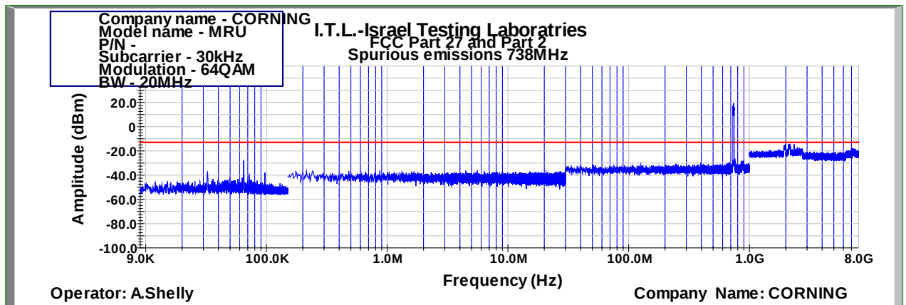
Figure 462: Spurious Emissions at Antenna Terminal 64QAM 20MHz B.W.; 738.0MHz, 30kHz
