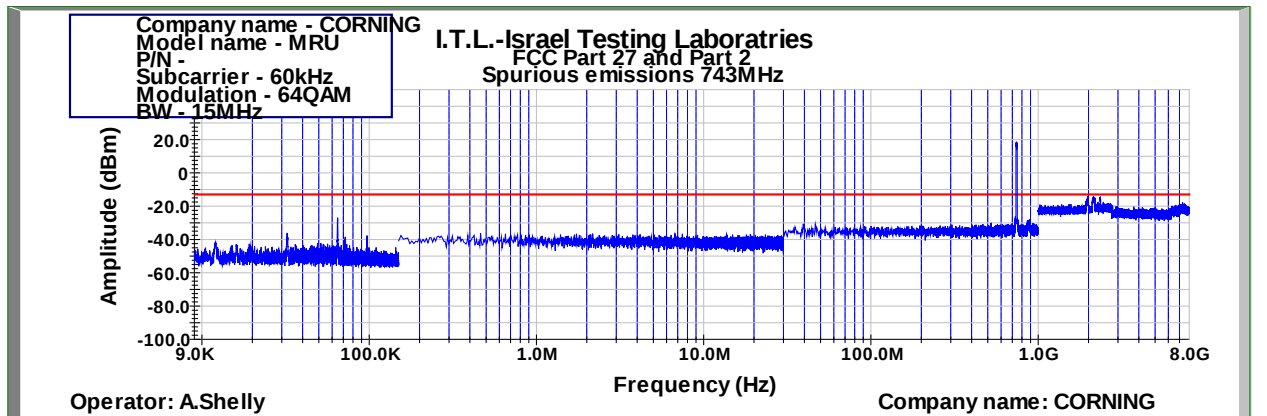
Figure 457: Spurious Emissions at Antenna Terminal 64QAM 15MHz B.W.; 743.0MHz, 60kHz
