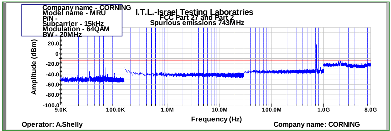
Figure 464: Spurious Emissions at Antenna Terminal 64QAM 20MHz B.W.; 743.0MHz, 15kHz
