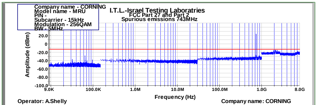
Figure 472: Spurious Emissions at Antenna Terminal 256QAM 5MHz B.W.; 743.0MHz, 15kHz
