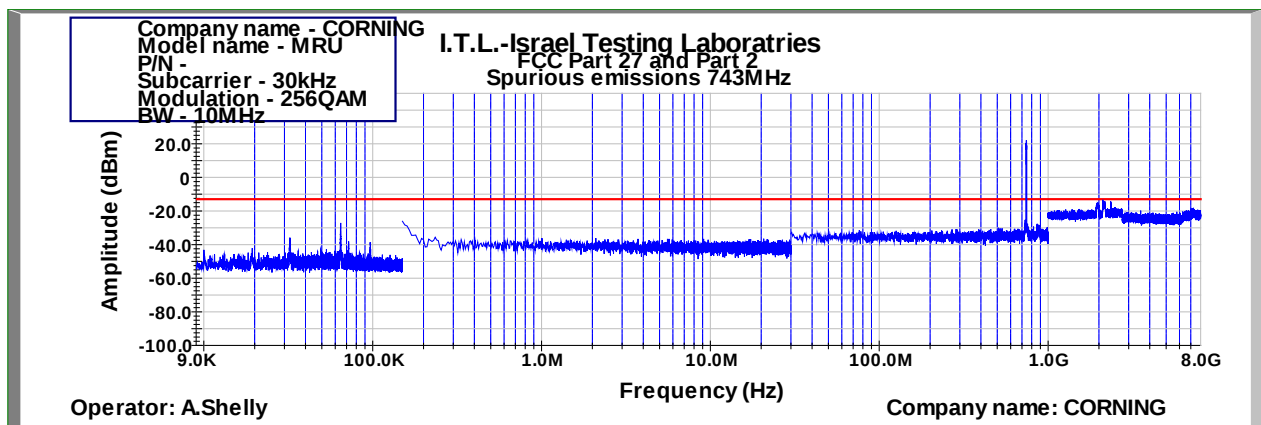
Figure 480: Spurious Emissions at Antenna Terminal 256QAM 10MHz B.W.; 743.0MHz, 30kHz
