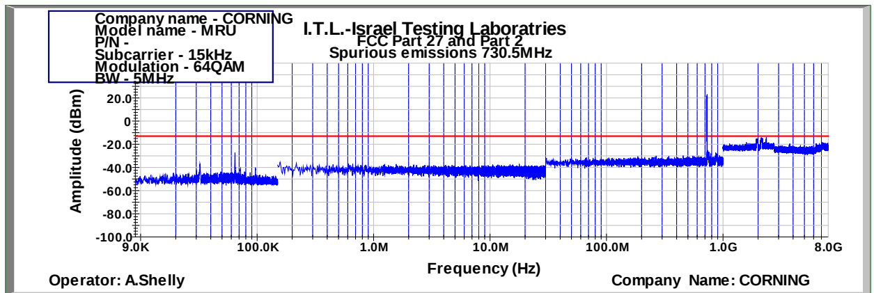
Figure 437: Spurious Emissions at Antenna Terminal 64QAM 5MHz B.W.; 730.5MHz, 15kHz
