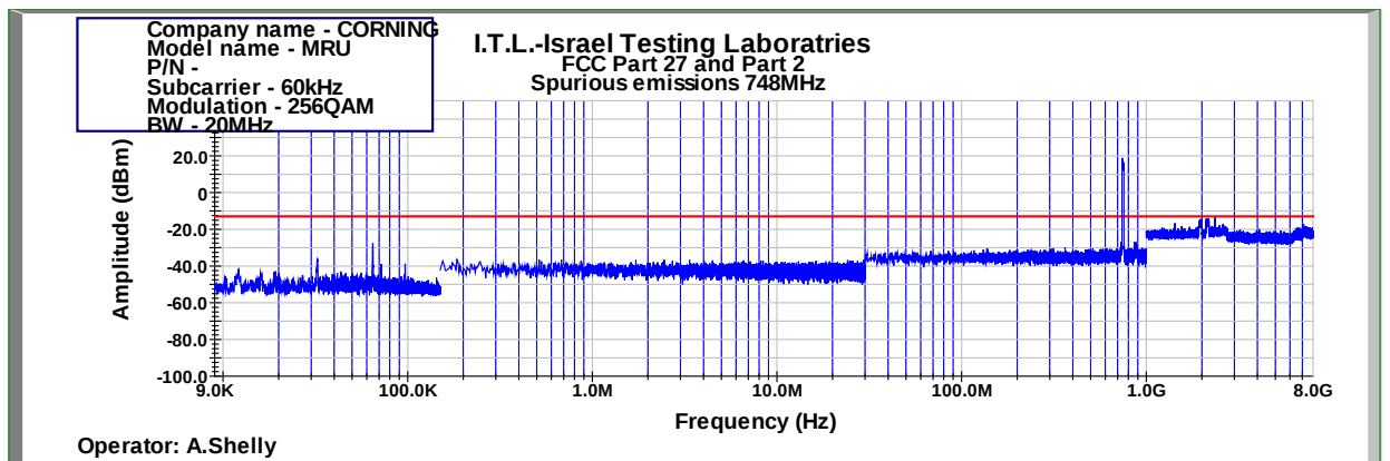
Figure 502: Spurious Emissions at Antenna Terminal 256QAM 20MHz B.W.; 748.0MHz, 60kHz
