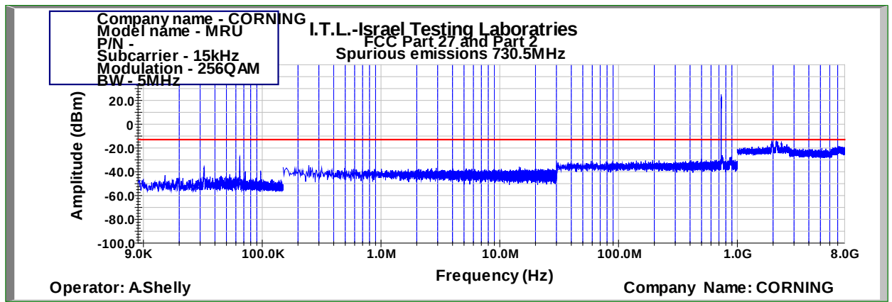
Figure 470: Spurious Emissions at Antenna Terminal 256QAM 5MHz B.W.; 730.5MHz, 15kHz
