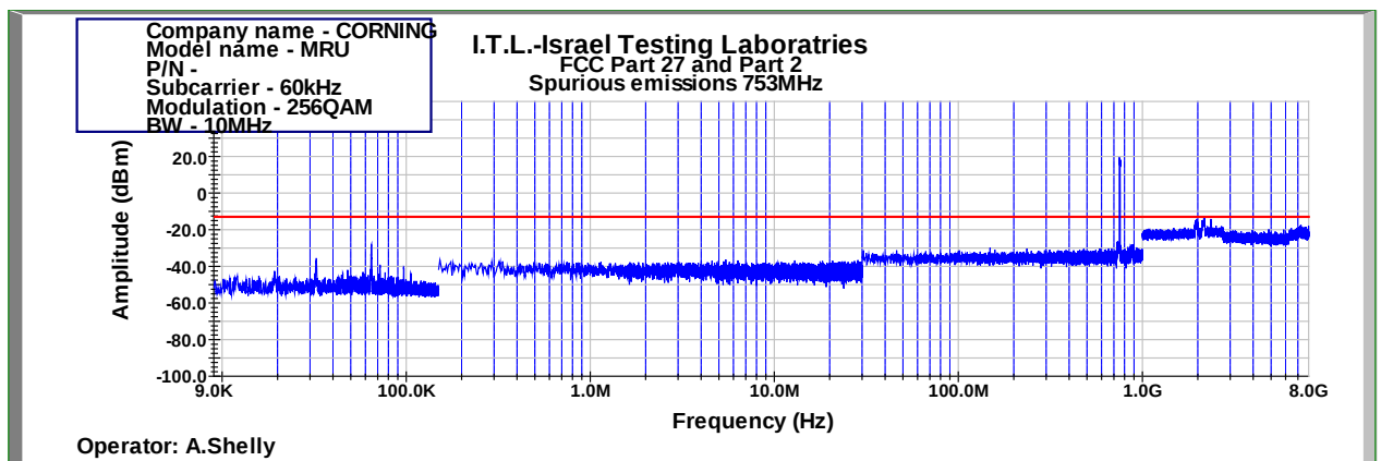
Figure 484: Spurious Emissions at Antenna Terminal 256QAM 10MHz B.W.; 753.0MHz, 60kHz
