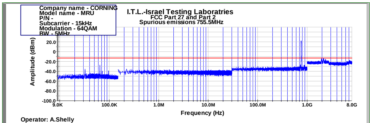
Figure 441: Spurious Emissions at Antenna Terminal 64QAM 5MHz B.W.; 755.5MHz, 15kHz
