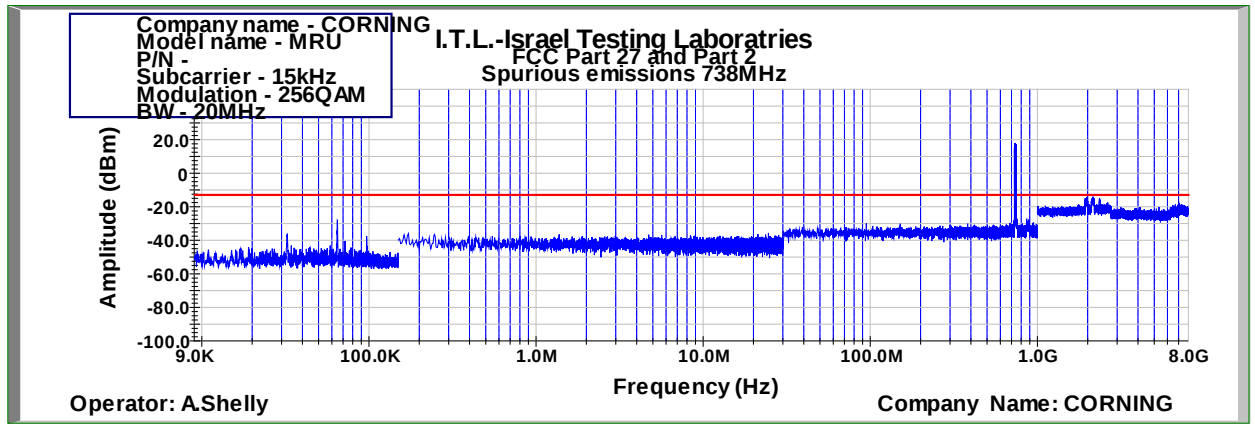
Figure 494: Spurious Emissions at Antenna Terminal 256QAM 20MHz B.W.; 738.0MHz, 15kHz
