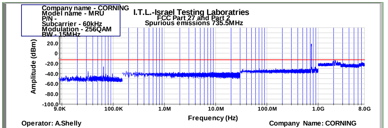
Figure 487: Spurious Emissions at Antenna Terminal 256QAM 15MHz B.W.; 735.5MHz, 60kHz
