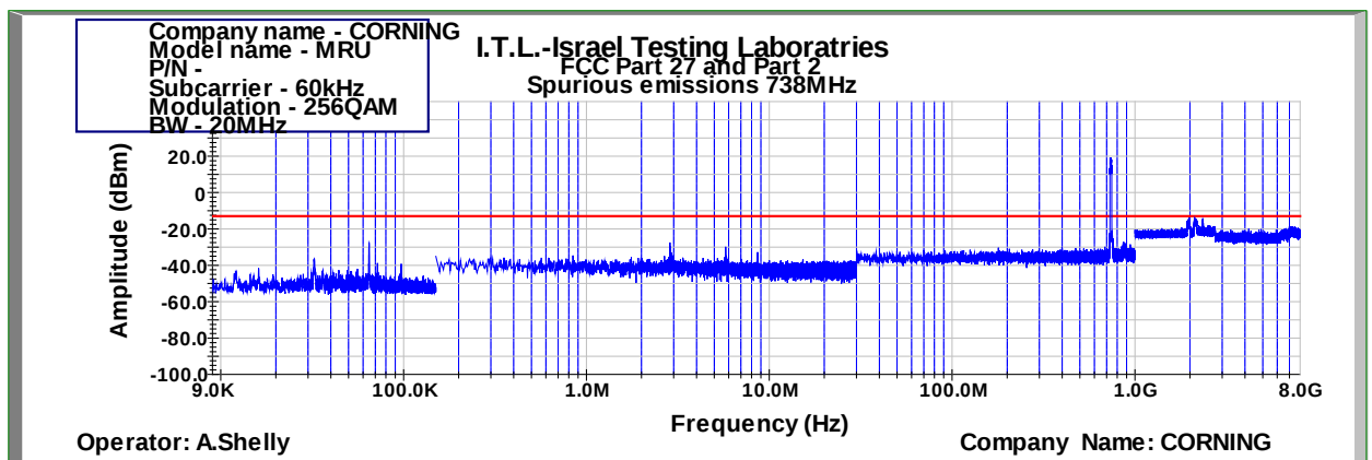
Figure 496: Spurious Emissions at Antenna Terminal 256QAM 20MHz B.W.; 738.0MHz, 60kHz
