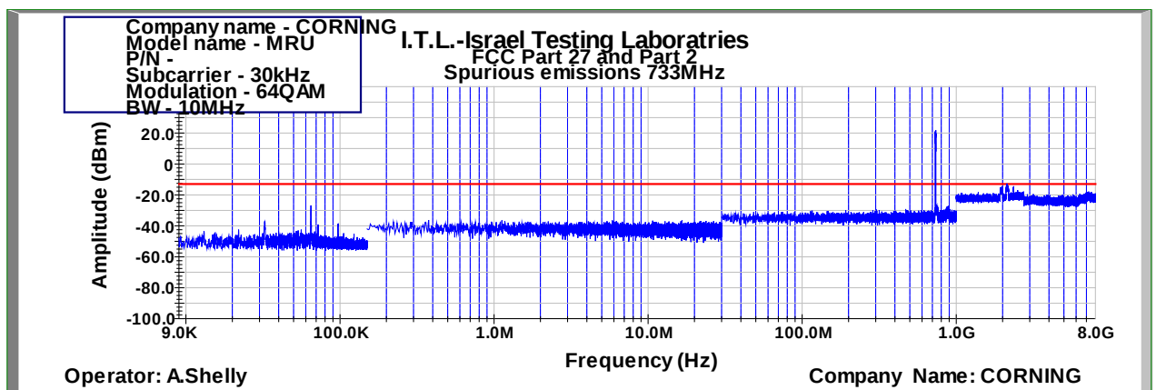
Figure 444: Spurious Emissions at Antenna Terminal 64QAM 10MHz B.W.; 733.0MHz, 30kHz
