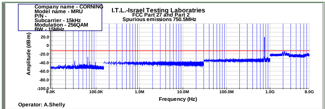
Figure 491: Spurious Emissions at Antenna Terminal 256QAM 15MHz B.W.; 750.5MHz, 15kHz
