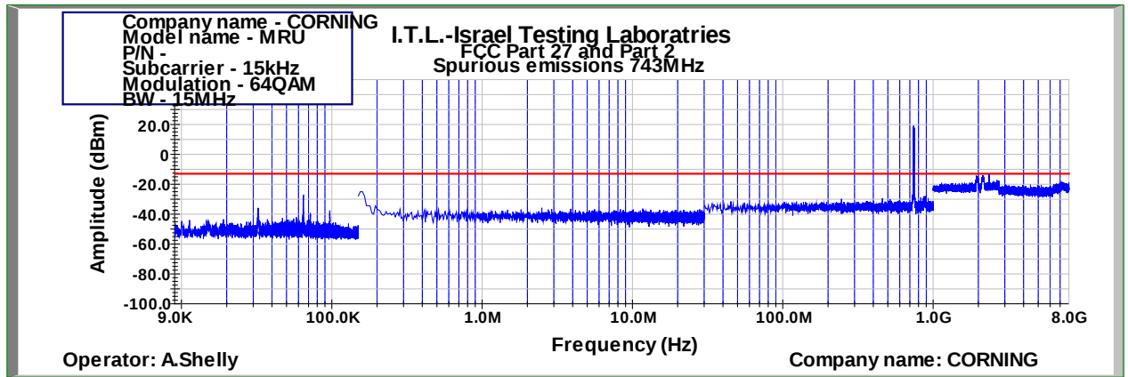
Figure 455: Spurious Emissions at Antenna Terminal 64QAM 15MHz B.W.; 743.0MHz, 15kHz
