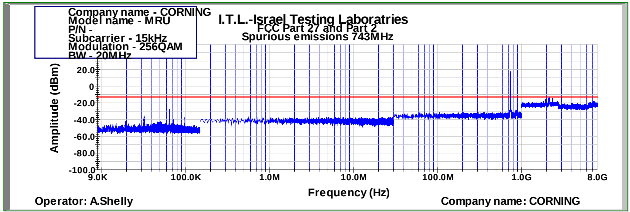
Figure 497: Spurious Emissions at Antenna Terminal 256QAM 20MHz B.W.; 743.0MHz, 15kHz
