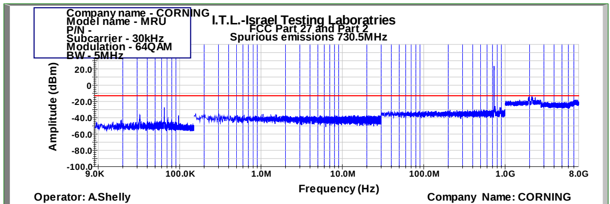
Figure 438: Spurious Emissions at Antenna Terminal 64QAM 5MHz B.W.; 730.5MHz, 30kHz
