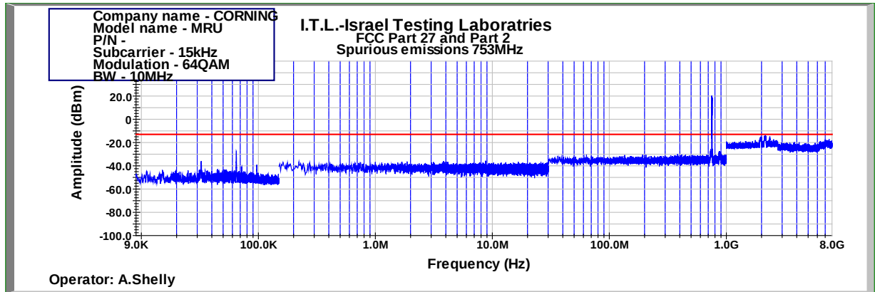
Figure 449: Spurious Emissions at Antenna Terminal 64QAM 10MHz B.W.; 753.0MHz, 15kHz
