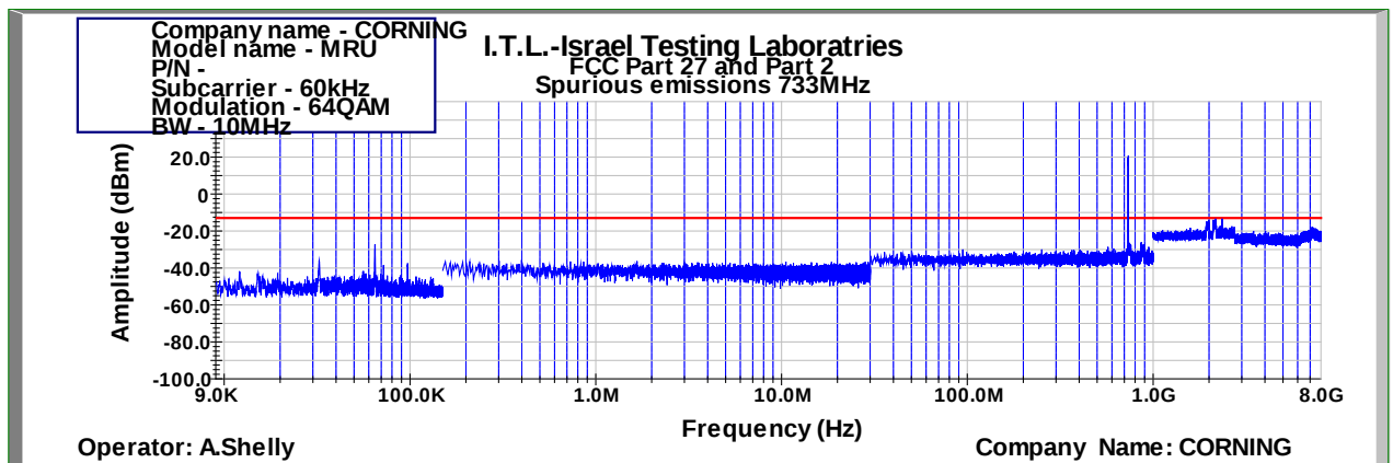
Figure 445: Spurious Emissions at Antenna Terminal 64QAM 10MHz B.W.; 733.0MHz, 60kHz
