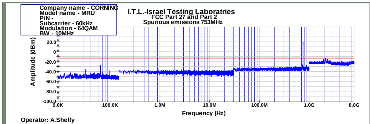
Figure 451: Spurious Emissions at Antenna Terminal 64QAM 10MHz B.W.; 753.0MHz, 60kHz
