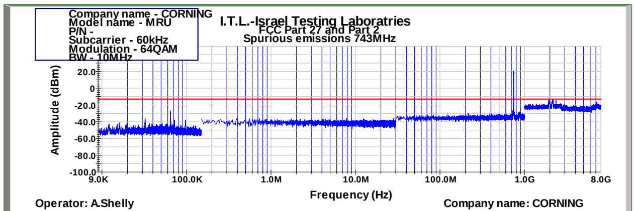
Figure 448: Spurious Emissions at Antenna Terminal 64QAM 10MHz B.W.; 743.0MHz, 60kHz
