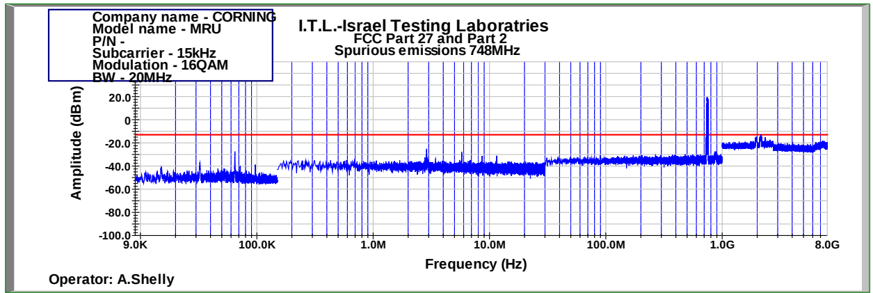
Figure 434: Spurious Emissions at Antenna Terminal 16QAM 20MHz B.W.; 748.0MHz, 15kHz
