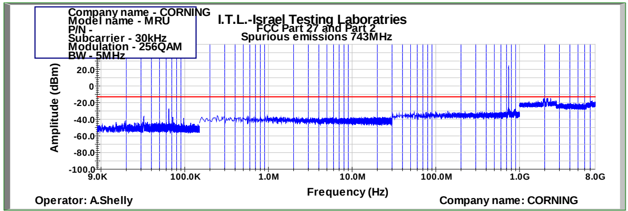
Figure 473: Spurious Emissions at Antenna Terminal 256QAM 5MHz B.W.; 743.0MHz, 30kHz
