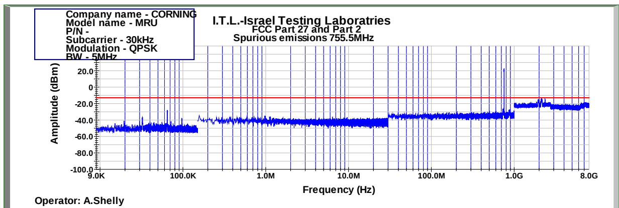
Figure 508: Spurious Emissions at Antenna Terminal QPSK 5MHz B.W.; 755.5MHz, 30kHz
