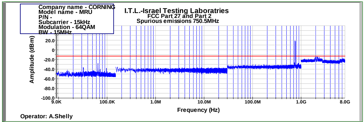
Figure 458: Spurious Emissions at Antenna Terminal 64QAM 15MHz B.W.; 750.5MHz, 15kHz
