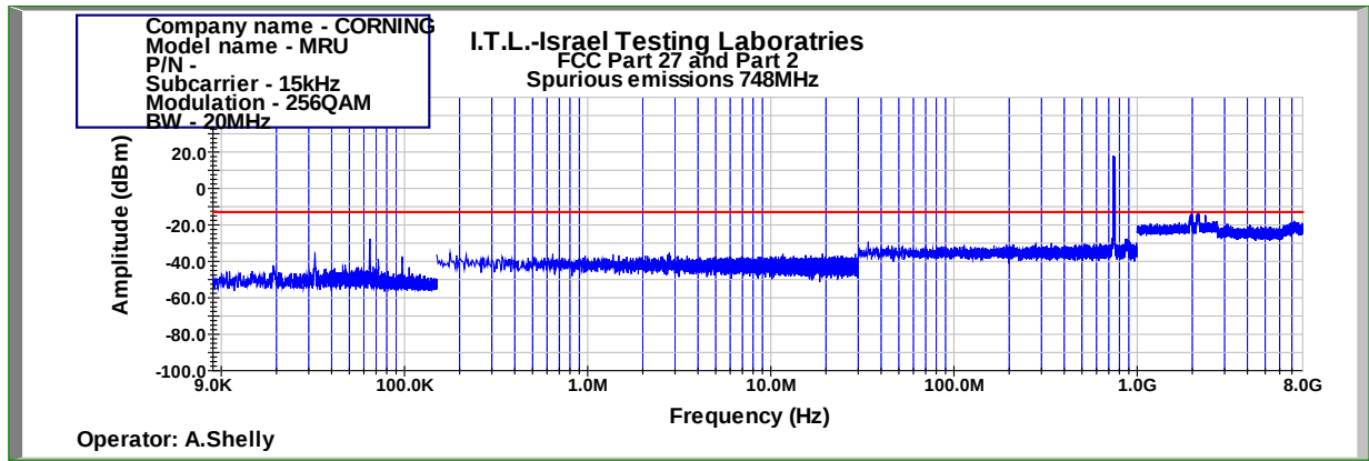
Figure 500: Spurious Emissions at Antenna Terminal 256QAM 20MHz B.W.; 748.0MHz, 15kHz
