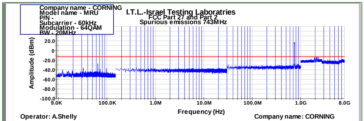
Figure 466: Spurious Emissions at Antenna Terminal 64QAM 20MHz B.W.; 743.0MHz, 60kHz
