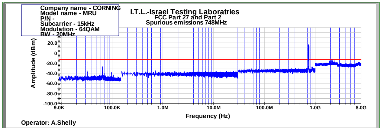
Figure 467: Spurious Emissions at Antenna Terminal 64QAM 20MHz B.W.; 748.0MHz, 15kHz
