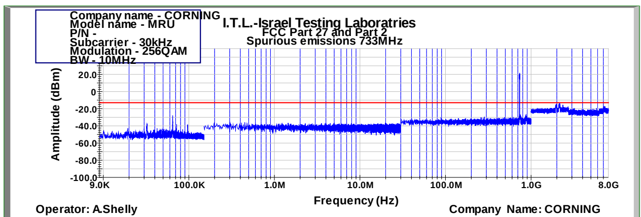
Figure 477: Spurious Emissions at Antenna Terminal 256QAM 10MHz B.W.; 733.0MHz, 30kHz
