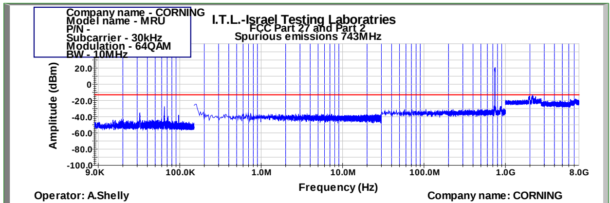
Figure 447: Spurious Emissions at Antenna Terminal 64QAM 10MHz B.W.; 743.0MHz, 30kHz
