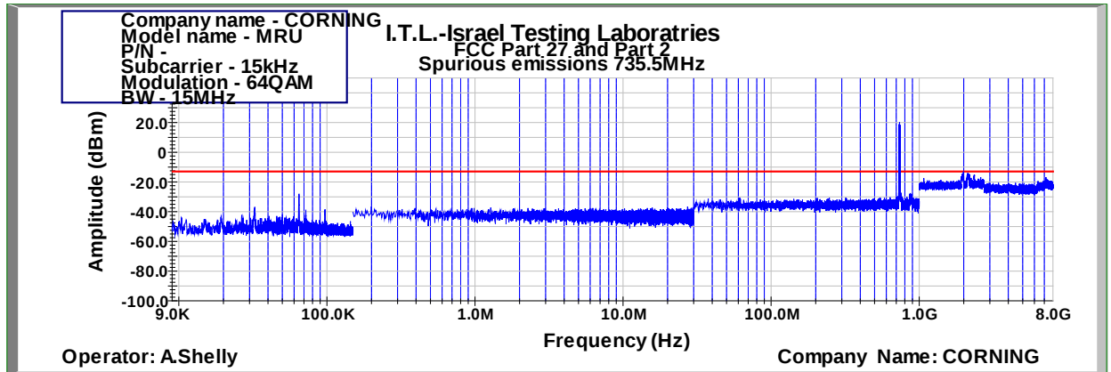
Figure 452: Spurious Emissions at Antenna Terminal 64QAM 15MHz B.W.; 735.5MHz, 15kHz
