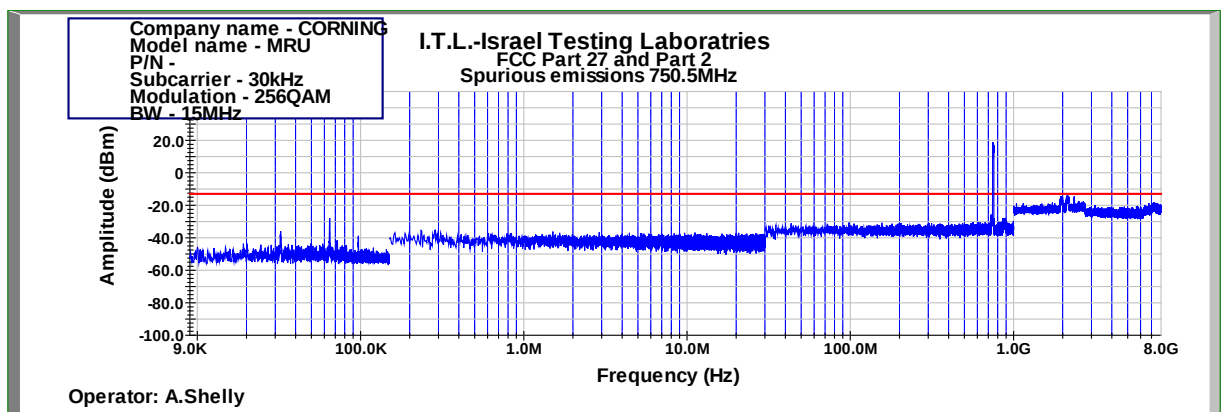
Figure 492: Spurious Emissions at Antenna Terminal 256QAM 15MHz B.W.; 750.5MHz, 30kHz
