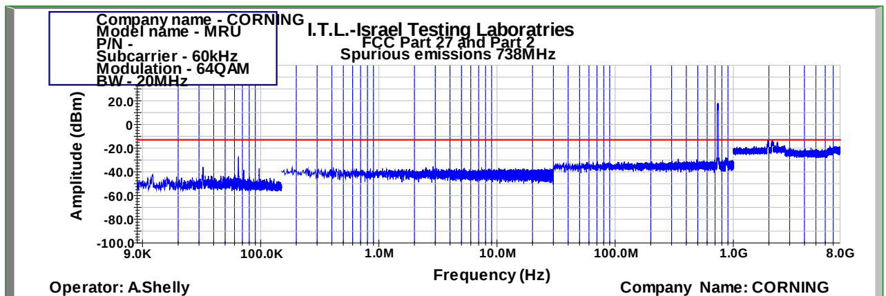
Figure 463: Spurious Emissions at Antenna Terminal 64QAM 20MHz B.W.; 738.0MHz, 60kHz
