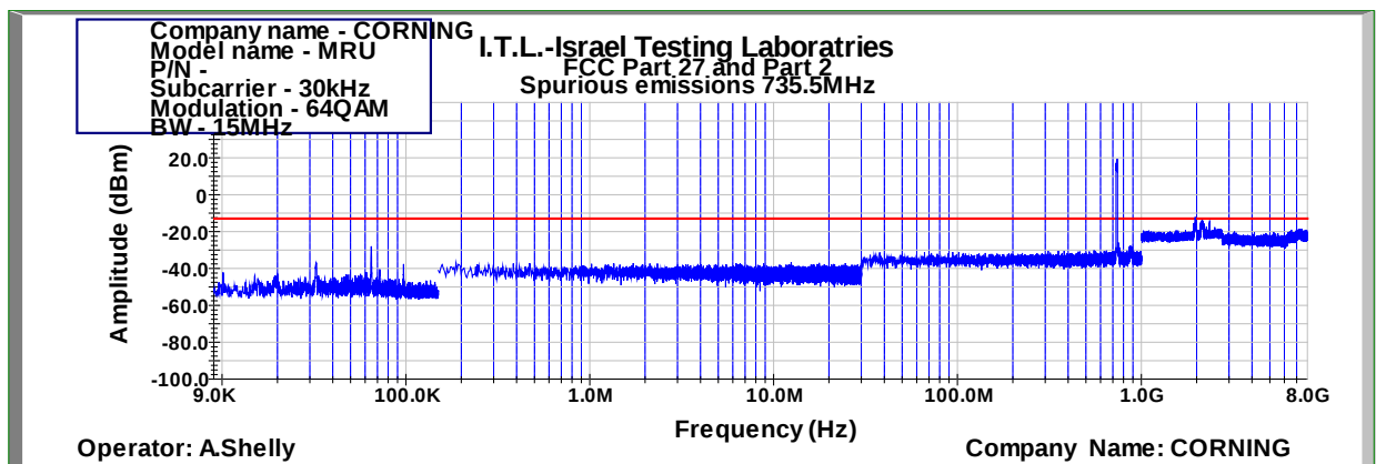
Figure 453: Spurious Emissions at Antenna Terminal 64QAM 15MHz B.W.; 735.5MHz, 30kHz
