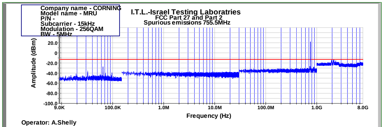
Figure 474: Spurious Emissions at Antenna Terminal 256QAM 5MHz B.W.; 755.5MHz, 15kHz
