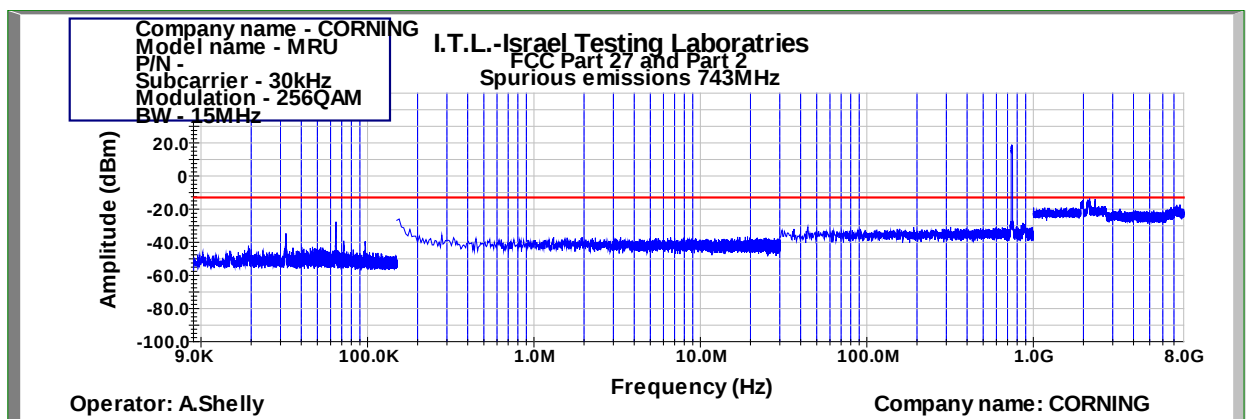
Figure 489: Spurious Emissions at Antenna Terminal 256QAM 15MHz B.W.; 743.0MHz, 30kHz
