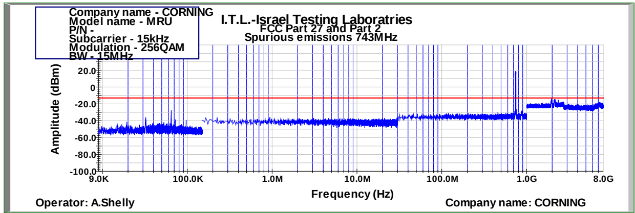
Figure 488: Spurious Emissions at Antenna Terminal 256QAM 15MHz B.W.; 743.0MHz, 15kHz
