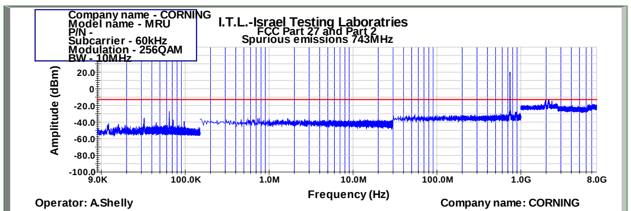
Figure 481: Spurious Emissions at Antenna Terminal 256QAM 10MHz B.W.; 743.0MHz, 60kHz
