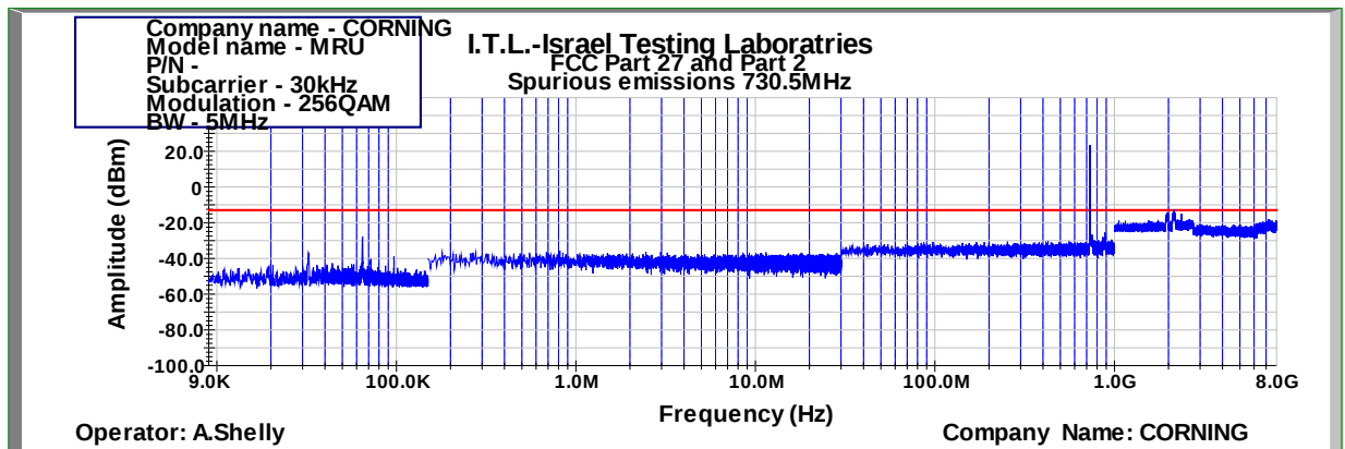
Figure 471: Spurious Emissions at Antenna Terminal 256QAM 5MHz B.W.; 730.5MHz, 30kHz
