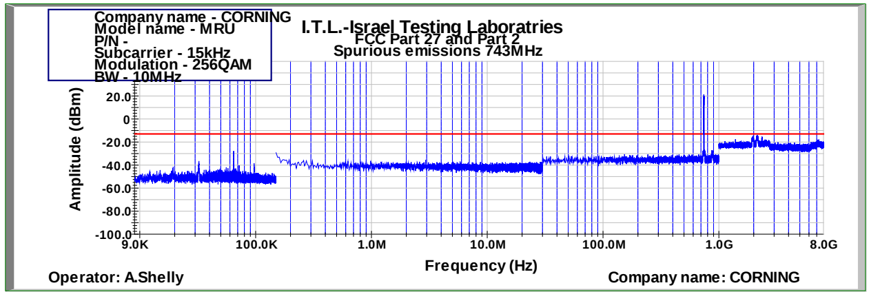
Figure 479: Spurious Emissions at Antenna Terminal 256QAM 10MHz B.W.; 743.0MHz, 15kHz
