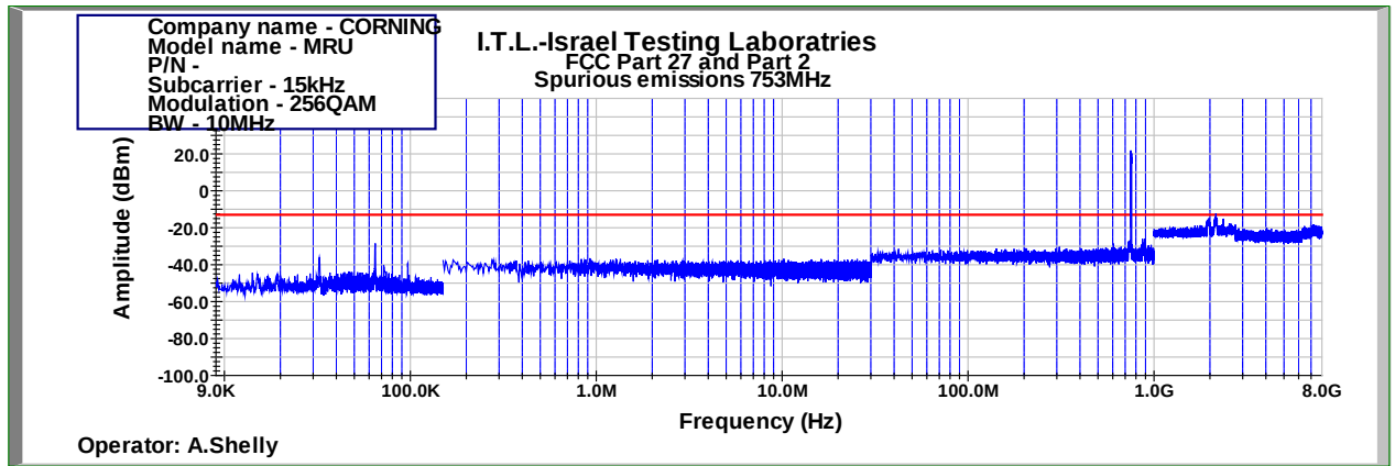
Figure 482: Spurious Emissions at Antenna Terminal 256QAM 10MHz B.W.; 753.0MHz, 15kHz
