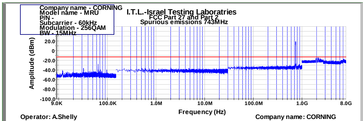
Figure 490: Spurious Emissions at Antenna Terminal 256QAM 15MHz B.W.; 743.0MHz, 60kHz
