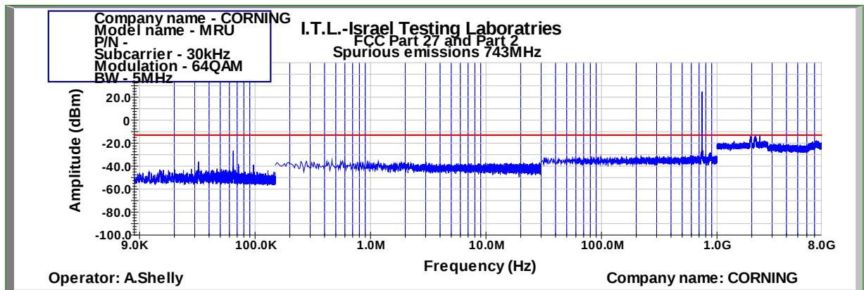
Figure 440: Spurious Emissions at Antenna Terminal 64QAM 5MHz B.W.; 743.0MHz, 30kHz
