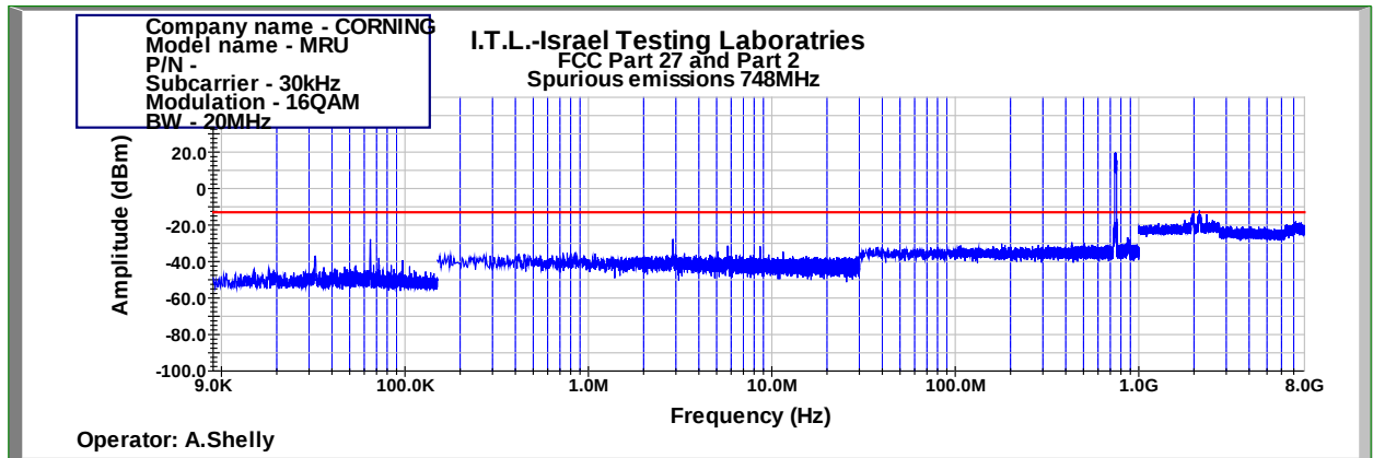
Figure 435: Spurious Emissions at Antenna Terminal 16QAM 20MHz B.W.; 748.0MHz, 30kHz
