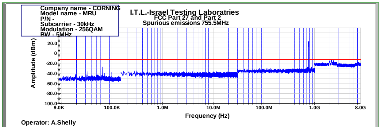
Figure 475: Spurious Emissions at Antenna Terminal 256QAM 5MHz B.W.; 755.5MHz, 30kHz
