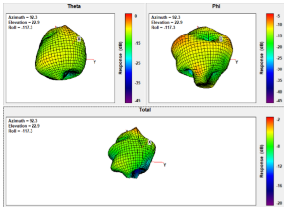
Ant4 Freq. 6175 MHz:
