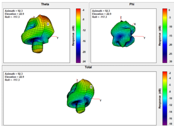
Ant4 Freq. 6475 MHz:
