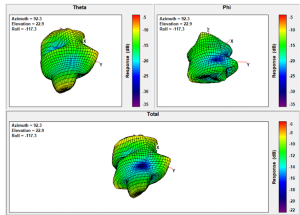
Ant4 Freq. 6700 MHz:
