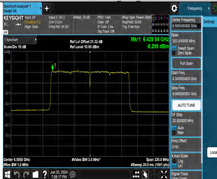
11BE160MIMO Ant2 6505
