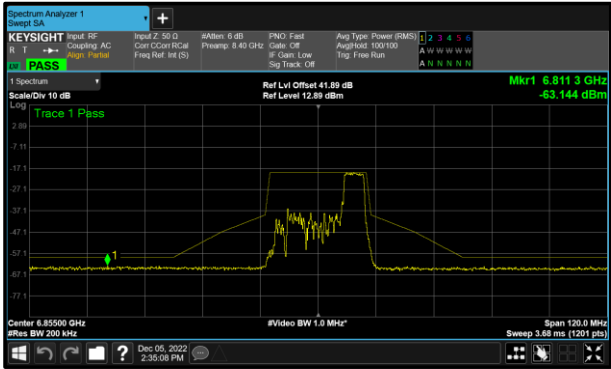
Figure 97 - A(Core 0) 802.11ax HE20 RU52 6855 MHz (CH181)
