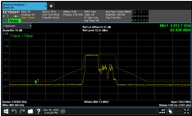
Figure 95 - A(Core 0) 802.11ax HE20 RU106 5955 MHz (CH1)
