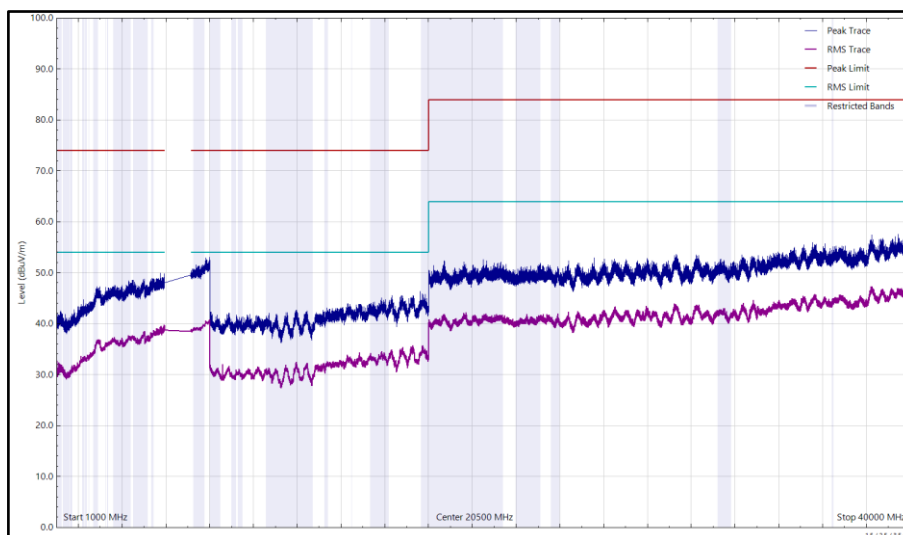
Figure 109 - U-NII-6 - 6435 MHz (CH97), HE20, SU, CDD, Core 0 + Core 1, 1 GHz to 40 GHz, Horizontal
