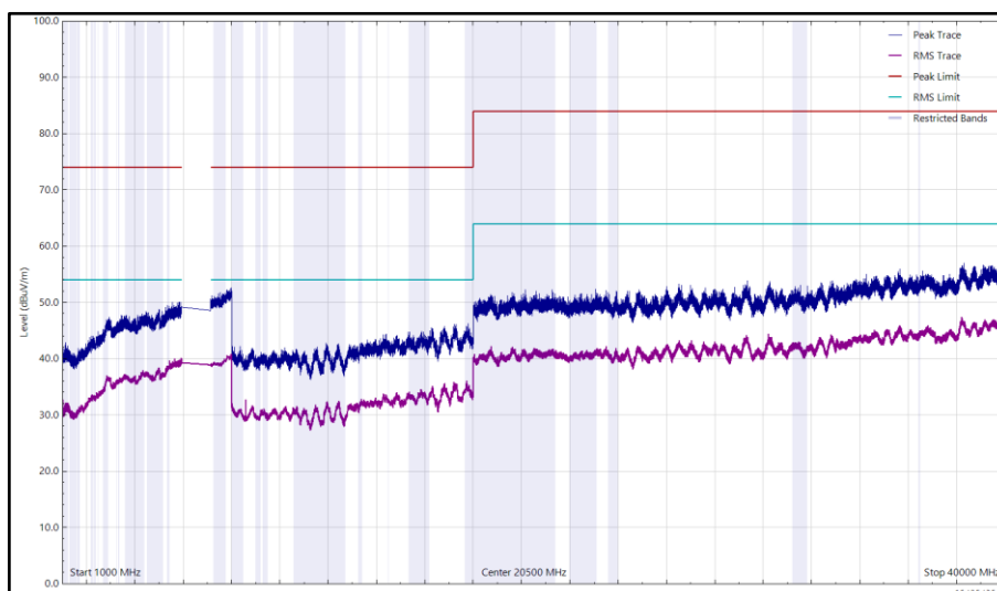
Figure 110 - U-NII-6 - 6435 MHz (CH97), HE20, SU, CDD, Core 0 + Core 1, 1 GHz to 40 GHz, Vertical
