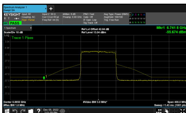
Figure 94 - A(Core 0) 802.11ax HE80 SU 6865 MHz (CH183)
