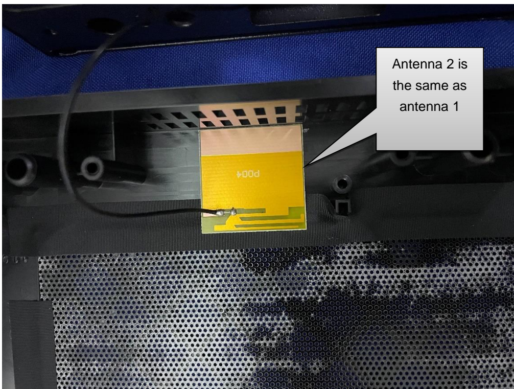
Antenna Interface
