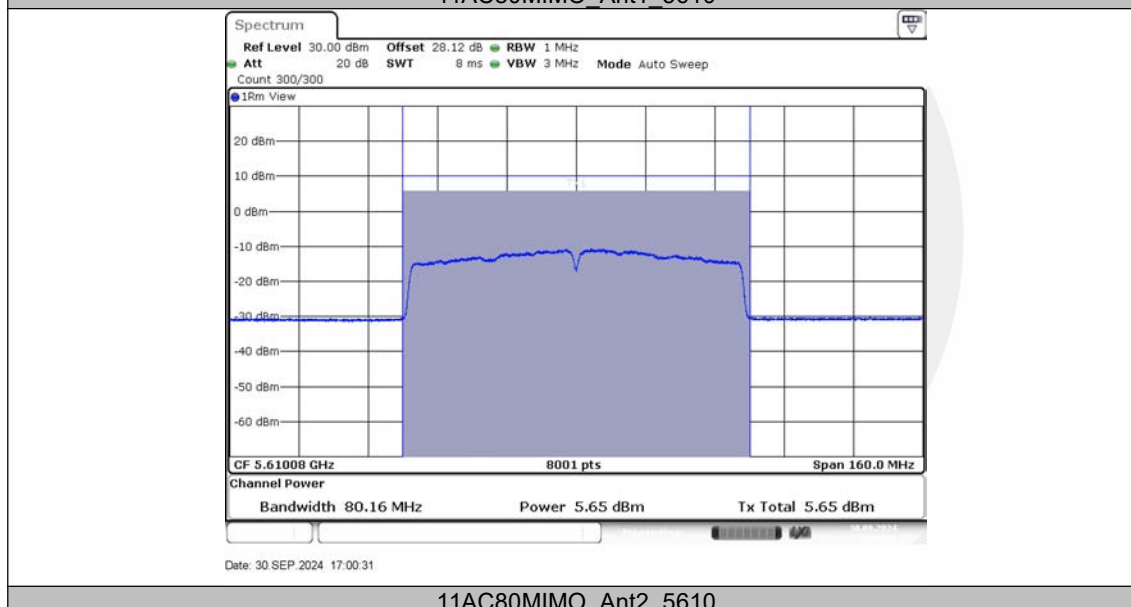
11AC80MIMO Ant2_5610
