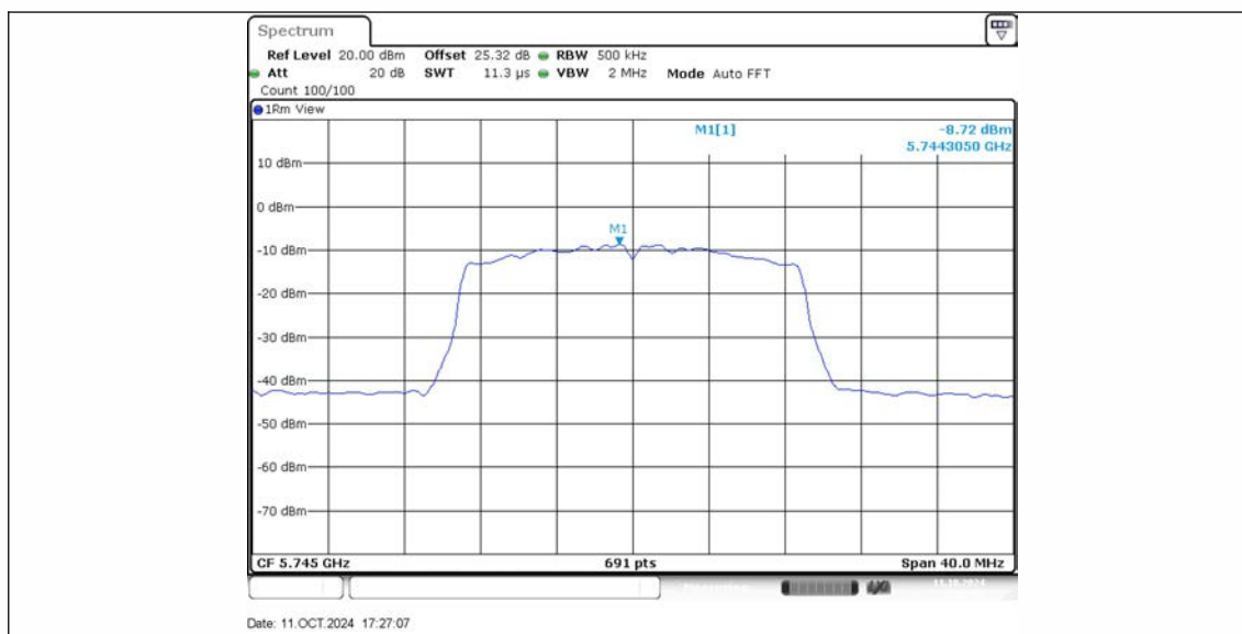
11AC20MIMO Ant2 5745
