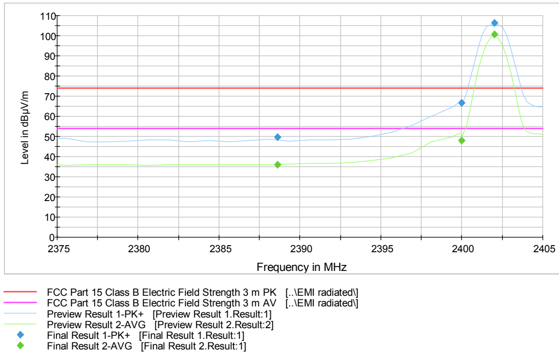
Figure 2: Radiated Band Edge measurement graph (ch low), A-variant
