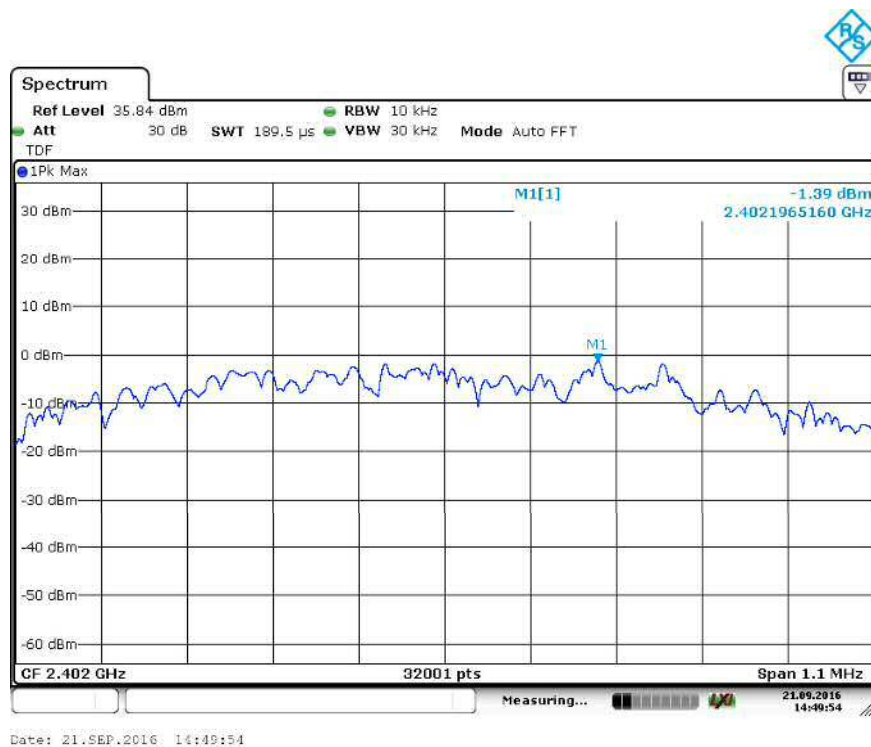
Figure 11: Power spectral density channel low
