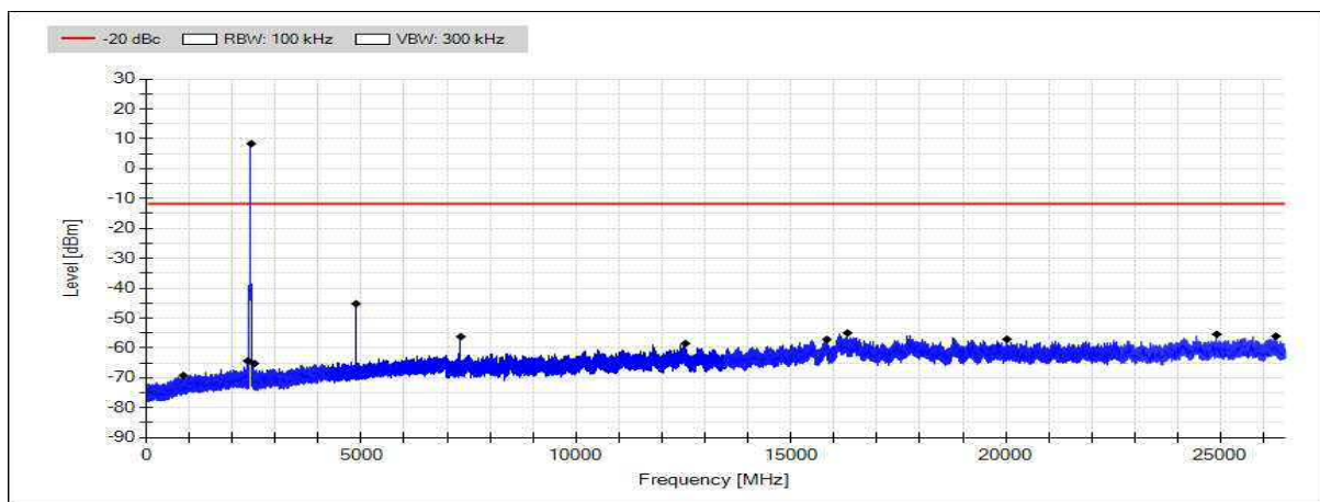
Figure 6: Conducted spurious emissions 30 - 26500 MHz channel mid
