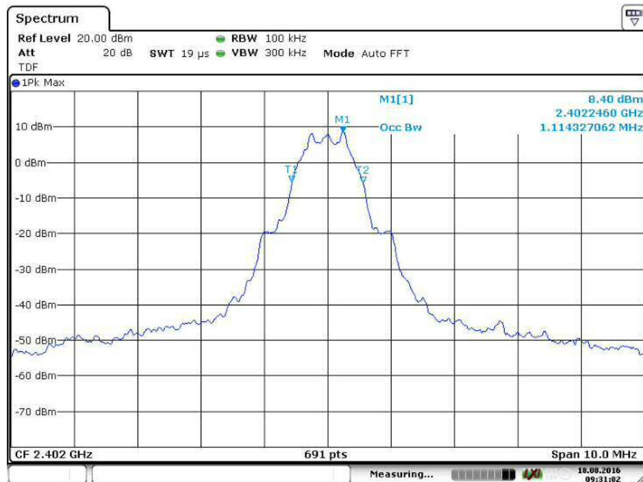
Figure 14: 99% OBW channel low
