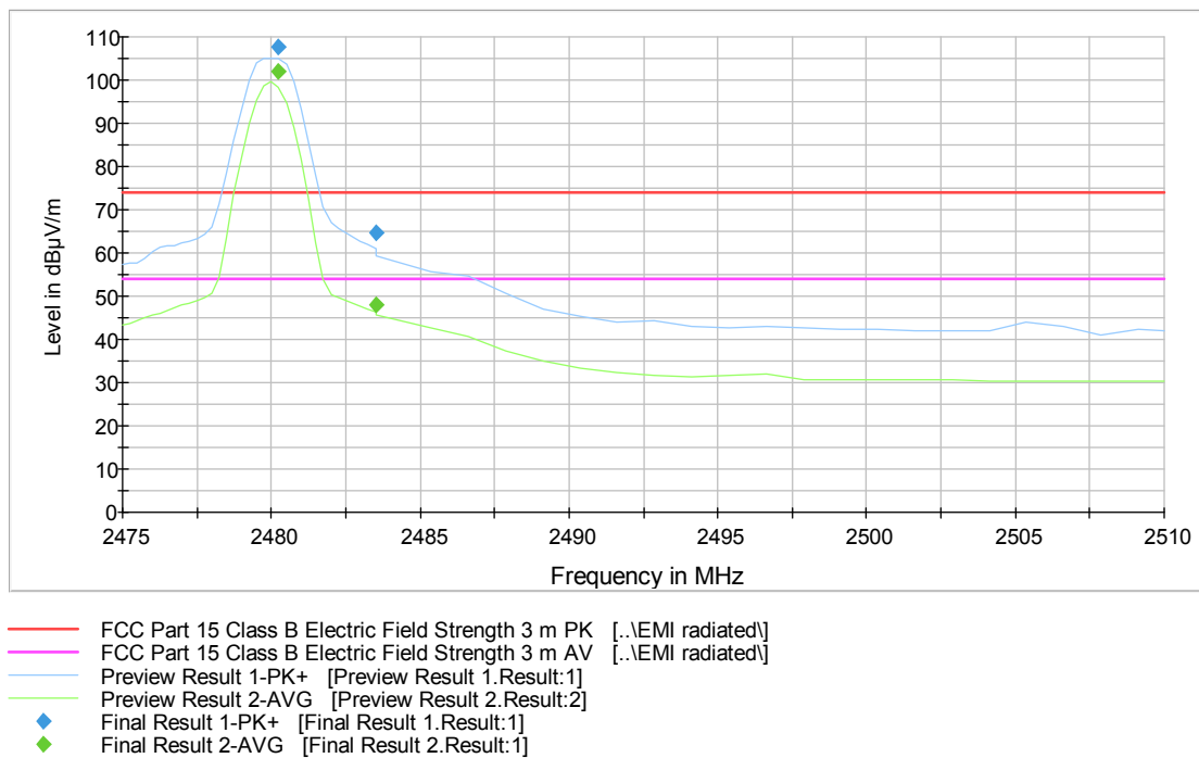
Figure 3: Radiated Band Edge measurement graph (ch high), A-variant
